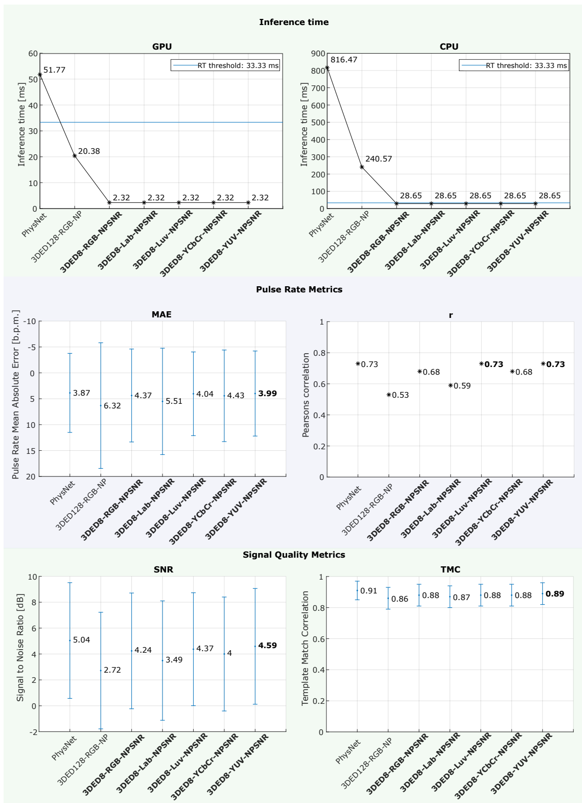
Figure 6.9: 3DED8-NPSNR network results when changing the color channel. In the first row the GPU and CPU inference time, in the second row the pulse rate metrics, and in the third one, the signal quality metrics. The experiments names in bold indicate that they are suitable for real-time in GPU and CPU.
