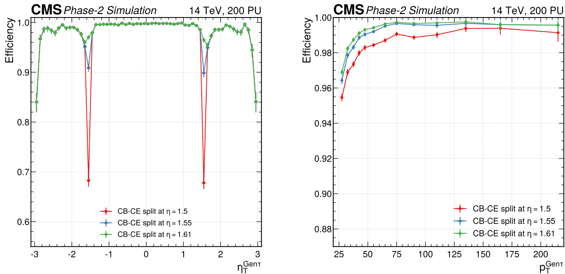
Figure 4.16: L1 \tau_h matching efficiency for the TAUMINATOR algorithm as a function of the \eta (left) and p_T (right) of the generated \tau_h . Results are shown for the different |\eta_{\text{seed}}| thresholds on the \text{CL}^{5 \times 9} seeding TT after which geometrical matching with a \text{CL}^{3\text{D}} is required.
