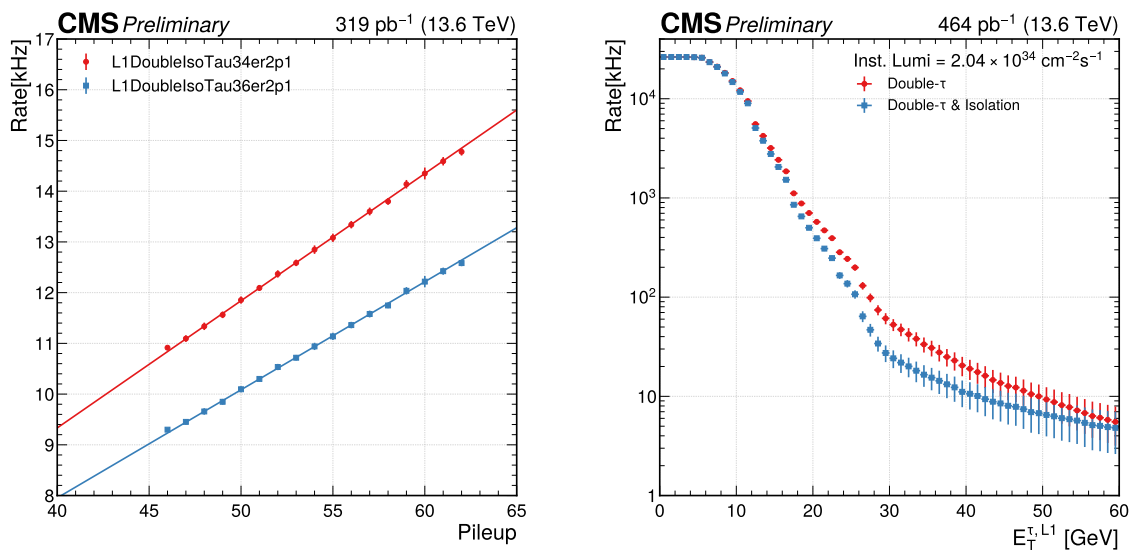
Figure 3.20: Level-1 trigger rate as a function of pileup, evaluated in a single LHC fill, for two Level-1 \tau_h trigger seeds: double isolated \tau_h with E_T > 34 GeV and |\eta| < 2.1 (red), and double isolated \tau_h with E_T > 36 GeV and |\eta| < 2.1 (blue). Rate and pileup are averaged over a time interval of a luminosity section , corresponding to 2^{18} LHC orbits or 23.31 sec of data-taking. The functional form of the fits consists of a second-degree polynomial (left). Level-1 double- \tau_h trigger rate as a function of the E_T threshold applied on both candidates, for both isolated and non-isolated candidates (right). Both results are measured in Run-3 2023 data.
