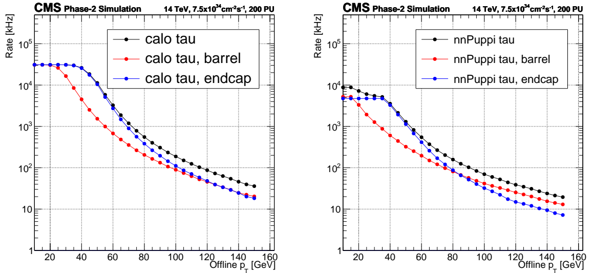
Figure 4.9: Level-1 single- \tau_h rate of the candidate for the CALOTAU (left) and the NNPUPI Tau (right) algorithms as a function of the offline p_T , defined as the generator p_T value at which the trigger turnon crosses the 90% efficiency point. The rate is evaluated in a Monte Carlo simulated minimum-bias dataset with 200 pileup interactions; the separate barrel and endcap contributions are reported.
