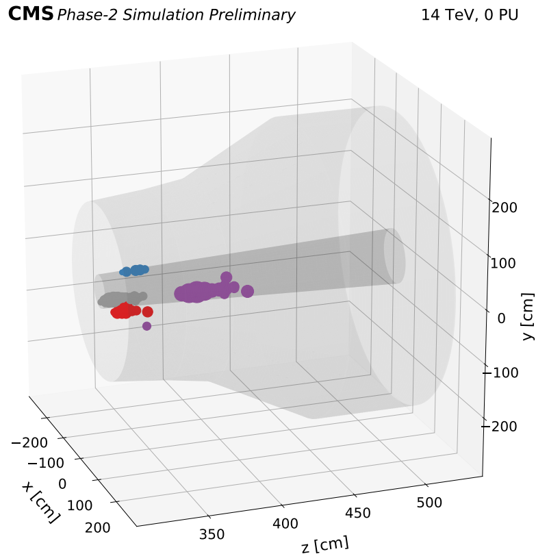
Figure 4.6: Exemplary reconstruction of CL^{3D} s in the HGCal detector for an event with no pile-up in which four 3D clusters are reconstructed and displayed in four different colours. The HGCal geometrical outer envelope is shown in dim-grey, while the inner envelope where the beam pipe lies is shown in darker grey.
