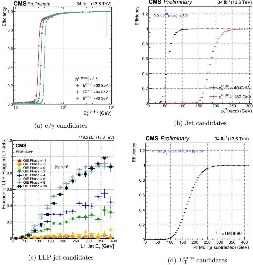
Figure 2.19: Level-1 performance of selected objects relevant for the calorimeter trigger. (a) The L1 e/\gamma trigger efficiency as a function of the offline reconstructed E_T for three different high E_T thresholds on the L1 trigger e/\gamma candidate; the functional form of the fits consists of a cumulative Crystal Ball function with a polynomial tail in the low E_T region. (b) L1 jet efficiency as a function of the offline jet p_T , for two L1 p_T thresholds. Low p_T^{L1} jets are observed to show a response below unity, resulting in a 50% efficiency for the p_T^{L1} > 40 GeV condition reached above the corresponding offline p_T value. This feature is primarily due to the limited accuracy of the jet energy corrections derived from simulations [152]. (c) The HCAL LLP-flagged L1 delayed jet fraction as a function of jet E_T during the 2023 HCAL phase scan demonstrates that the delayed jet fraction reaches unity as the phase delay increases. The delayed jet fraction begins decreasing at the largest delays (10 ns and above), as at these large delay settings, the total hadronic jet energy is reduced due to a significant amount of the jet energy being pushed into the subsequent bunch crossing. No direct selection is made with respect to jet E_T : the implicit requirement for a jet to have at least two cells with E_T > 4 GeV sculpts this distribution [153]. (d) L1 ETMHF90 efficiency, evaluated as the fraction of events for which the magnitude of the vector sum of all TT is E_T > 90 GeV, as a function of the offline transverse momentum of the event, removing the contribution from muons. In order to mitigate the impact of PU collisions, low E_T TTs are excluded from the ETMHF TT sum. Moreover, jet-level energy corrections are not propagated. These two effects result in a sizeable shift of the ETMHF response with respect to the offline measurement of the missing transverse energy [152].
