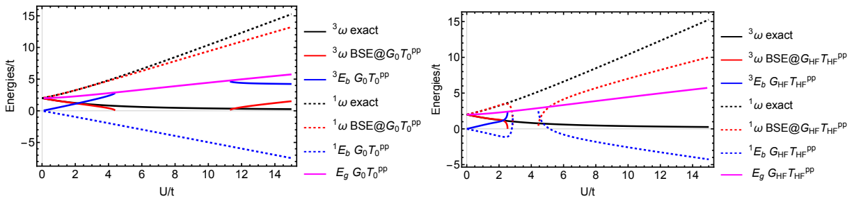
(a) Neutral excitation energies with G_0
