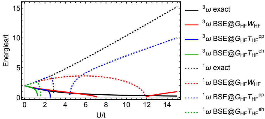
Figure 4.5 – Neutral excitation energies: exact (black), BSE@ GW (red), BSE@ GT^{pp} (blue) and BSE@ GT^{eh} (green) as functions of U/t in the symmetric Hubbard dimer ( \Delta v = 0 ) for the triplet (solid) and singlet (dashed) excited states.
