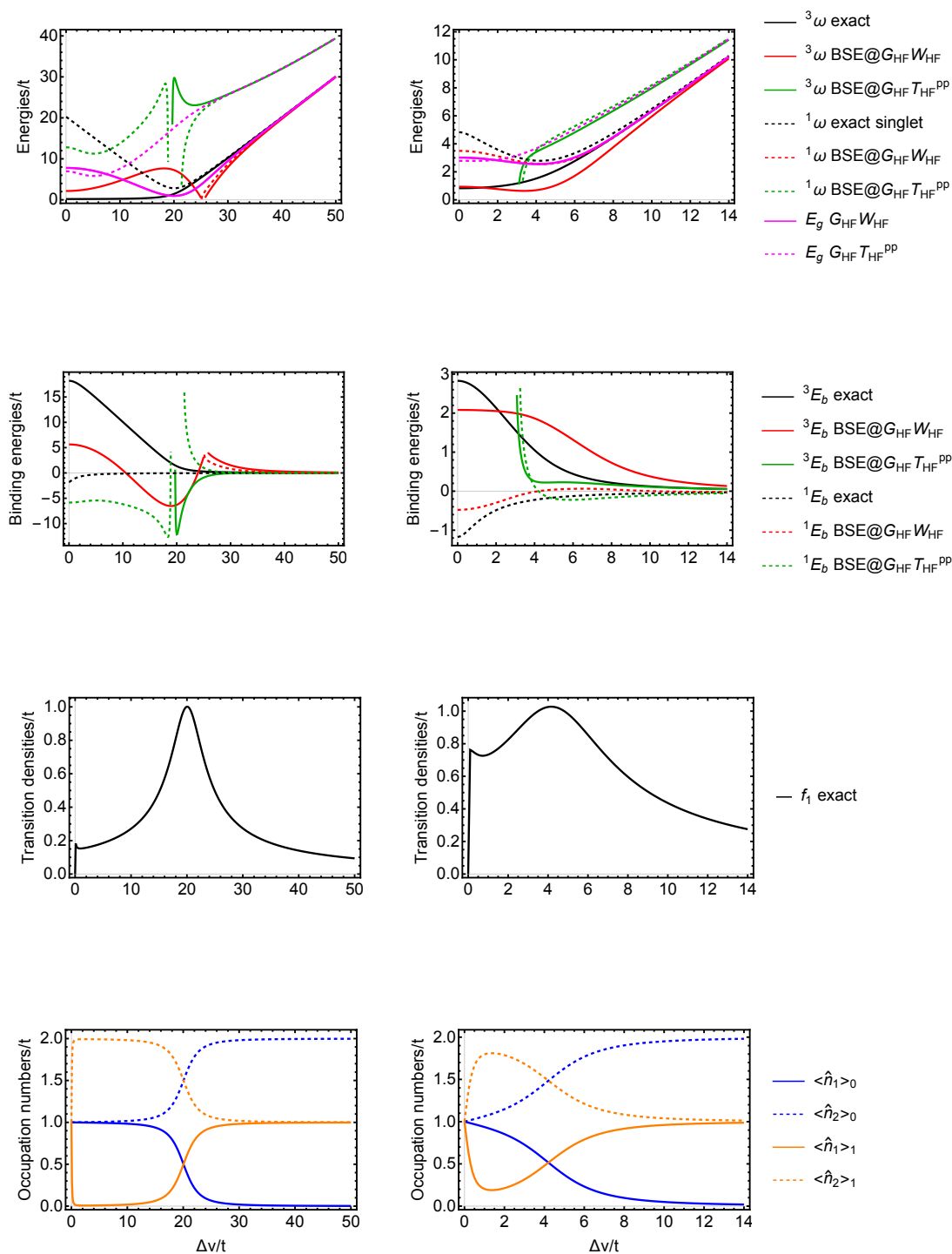
Figure 7.11 – Neutral excitations (first row), binding energies (second row), transitions densities (third row), and occupation numbers (fourth row) of the ground state and the first singlet excited state as functions of \Delta v/t . Results obtained for U/t = 20 (left column) and U/t = 4 (right column).
