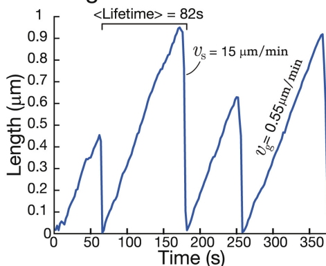
Figure 2.3: (Top) Base model of microtubule simulations dynamics, (Bottom) plot of the length as a function of time for one simulation, adapted from [126].
