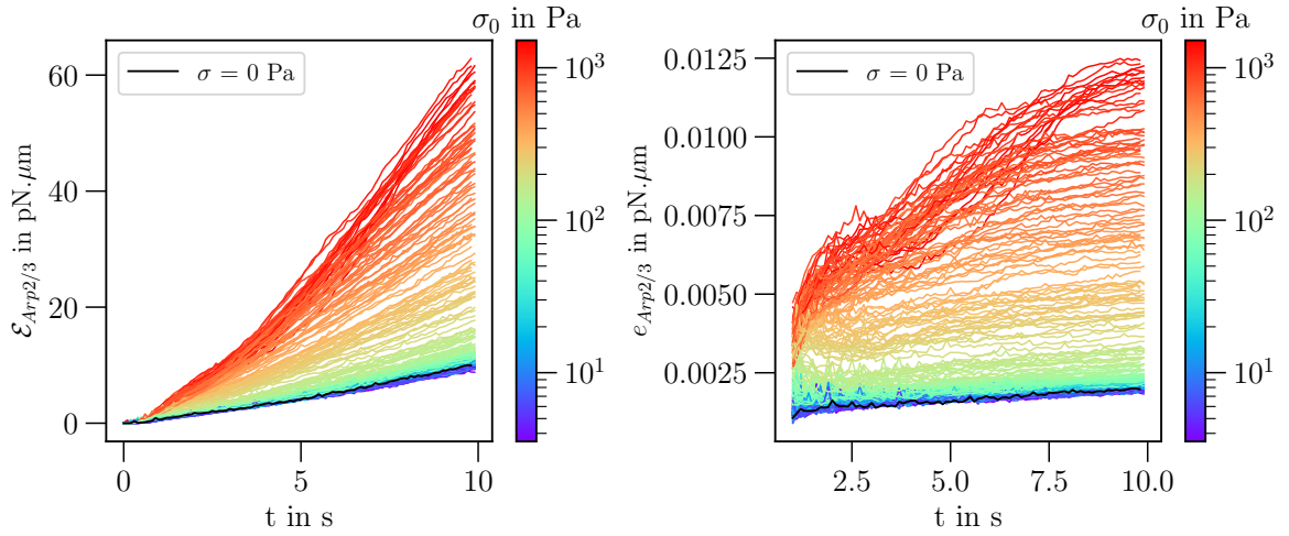
Figure A.14: Arp2/3 elastic energy as a function of time t for various stress \sigma_0 in Pa on (Left). Arp2/3 elastic energy per Arp2/3 on (Right), with f_s = 3.87 pN.
