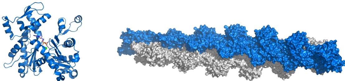
Figure 1.3: (Left) Ribbon diagram of G-Actin adapted from [24]. (Right) Representation of a 13 monomers F-Actin, work of Thomas Spletstoeser.
