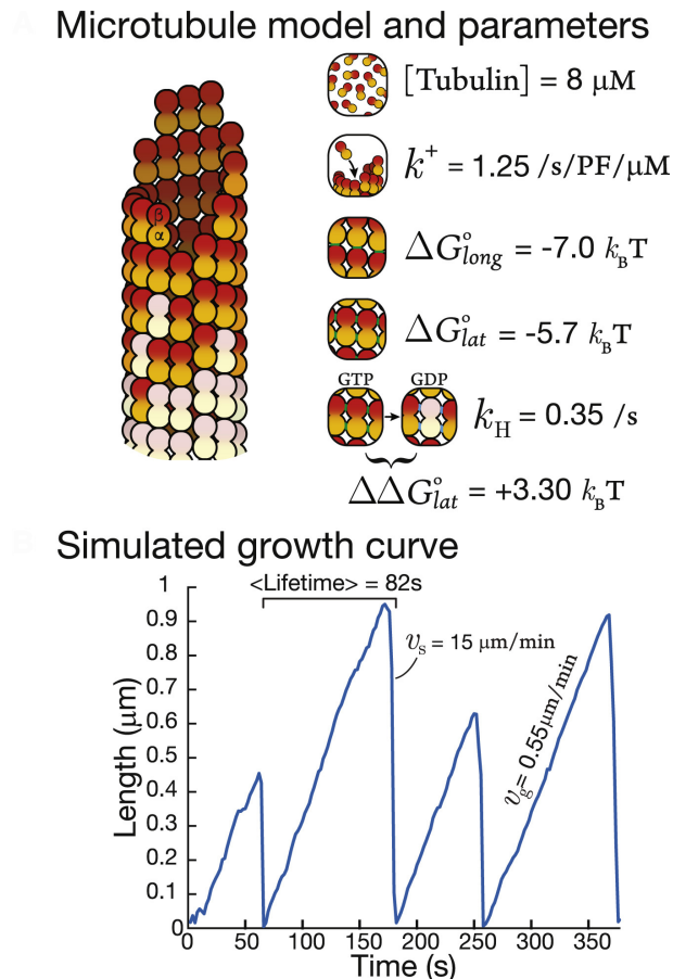
Figure 2.3: (Top) Base model of microtubule simulations dynamics, (Bottom) plot of the length as a function of time for one simulation, adapted from [126].
