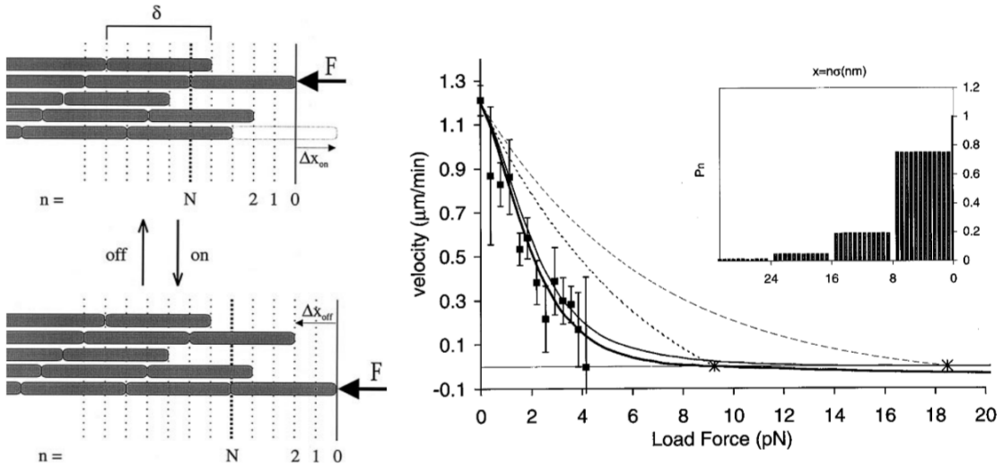
Figure 3.6: (Left) Discrete version of the Mogilner-Oster model for a polymer with N = 5 independently growing filaments. The addition of a monomer permits a displacement of the wall \Delta x_{on} , despite the force F . At the stall force, the two configurations are in equilibrium leading to detailed balance. (Right) The force-velocity relation for growing microtubules. Squares are the experiments from Dogterom et al. Solid lines are simulation results from the discrete theory:
