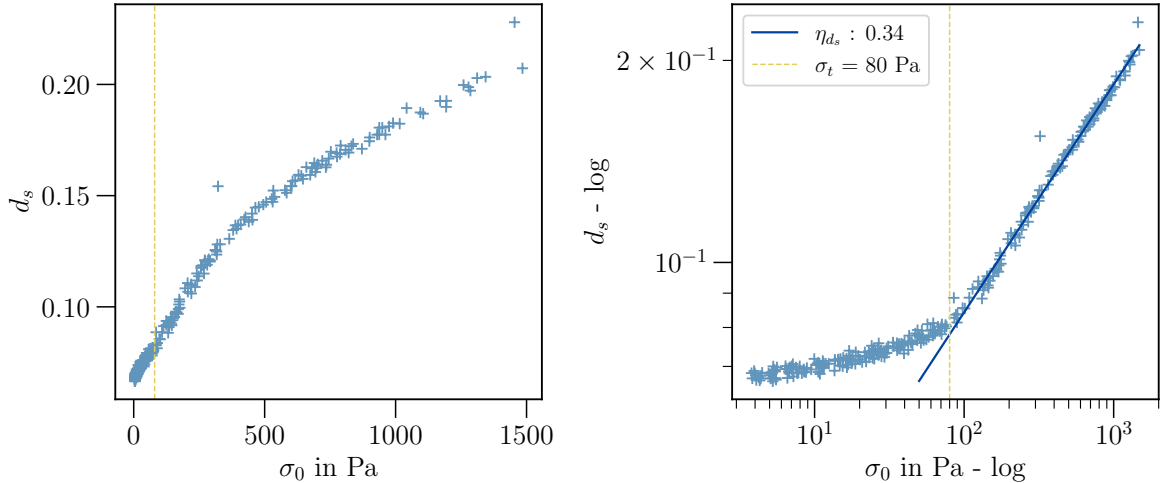
Figure 6.3: Near-stationary density for various stress in normal (Left) and log-log scales (Right), with f_s = \text{inf} pN. We see a power-law behavior for high stress after a constant value phase that ends around 80 Pa (yellow dotted line). The fit for the power-law scaling is represented in the log-log plot.
