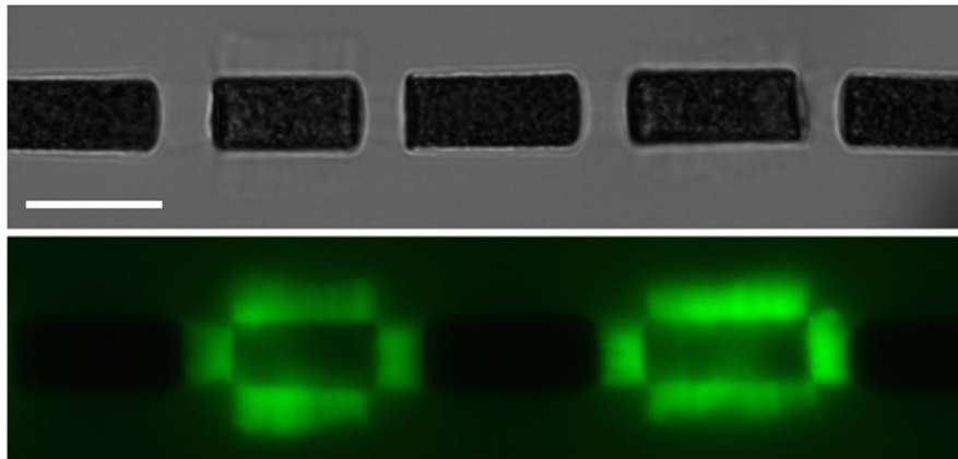
Figure 2.15: Chain of magnetic cylinders ( 6 \mu\text{m} in diameter) in an horizontal magnetic field. Top: Bright field image. Bottom: Fluorescent image (actin is labelled). Actin networks have grown from cylinders covered by the activator of the polymerization for around 15 minutes. Non actin-covered cylinders have been passivated. The cylinders are seen from the side, the circular faces being perpendicular to the image. Scale bar 10 \mu\text{m} , from [89].
