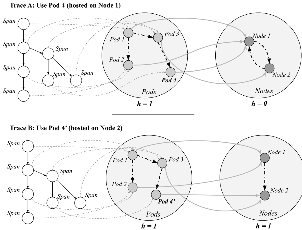
Figure 3.5: Examples of Flow Hierarchy Metric Calculation at Each Layer of the Containment Hierarchy for Two Traces
