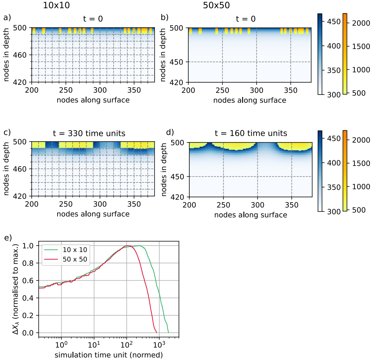
Figure 4.24 – Spatial distribution of the lambda phase domains at the initial state of the 500x500 system with a) 10x10, b) 50x50 grainsize. c and d shows the state of the system at the peak position for the two grains respectively. e) Evolution of the \lambda -phase fraction (normalised to its maximum value) with delays for the two different grain sizes. The simulation time unit is also normed to the peak position of the experimental dynamics of "flake-type" \text{Ti}_3\text{O}_5
