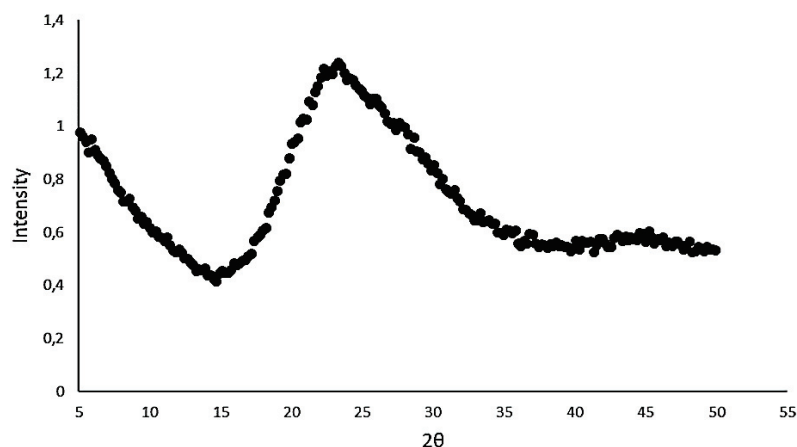
Figure 2.5: X-ray diffraction of TIB-PVAL
