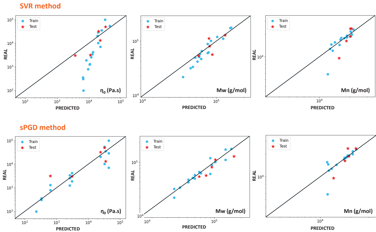
Figure VA-12. Results of zero-shear viscosity and weight and number average molecular weights predicted by SVR and sPGD methods versus the experimental ones. The blue dots correspond to training data, and the red stars correspond to test data for HDPE and UHMWPE indiscriminately
