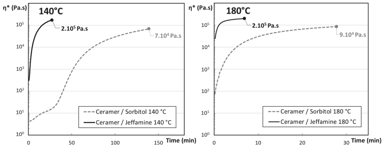
Figure VI-4. Variation of the absolute complex viscosity versus time for the two reactive systems at the temperature T=140^\circ\text{C} and 180^\circ\text{C} ; \omega=1 rad/s
