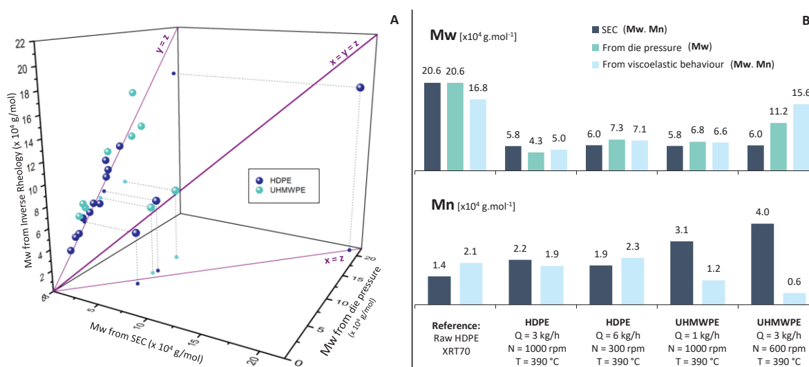
Figure VA-7. A: Comparison of weight average molecular weight (Mw) of degraded polyethylenes obtained from the estimated zero shear rate viscosity versus the one obtained from viscoelastic behaviour measurements. B: Comparison of weight average (Mw) and number average (Mn) molecular weight values obtained with different specified methodologies
