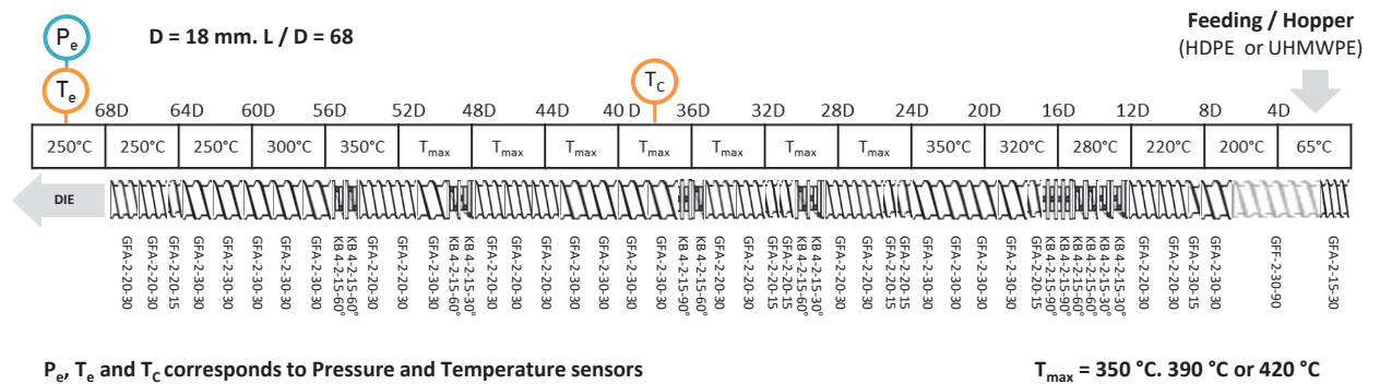
Figure VA-3. Scheme of the screw and temperature profiles used
