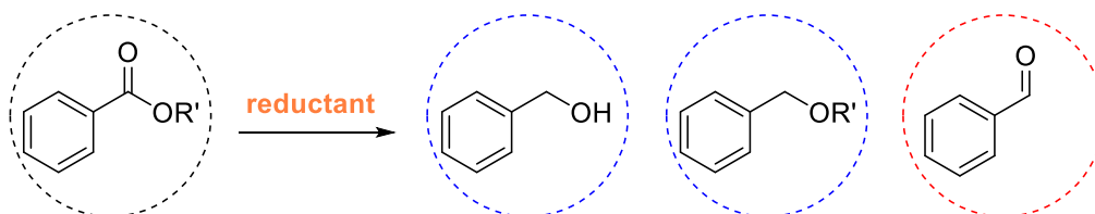
Scheme 15. Reduction of carboxylic acids and esters into alcohols, ethers, or aldehydes.
