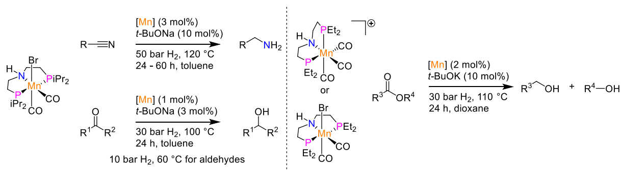
Scheme 2. Mn(I) pincer complexes bearing a PN-sp 3 P ligand for the hydrogenation of nitriles, aldehydes or ketones ( left ), and esters ( right ).
