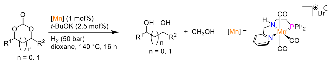
Scheme 10. Mn(I) complex of a PN-sp 3 N ligand for the hydrogenation of CO 2 -derived carbonates.
