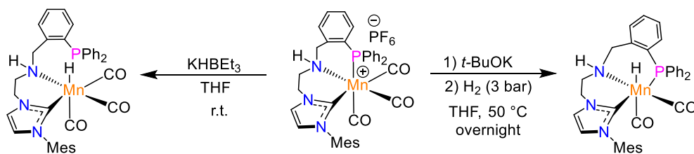
Scheme 15. Mn(I) complex based on a CNP pincer ligand for the hydrogenation of ketones, imines, aldehydes, and esters.
