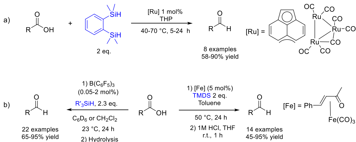
Scheme 2. Hydrosilylation of carboxylic acids into aldehydes.
