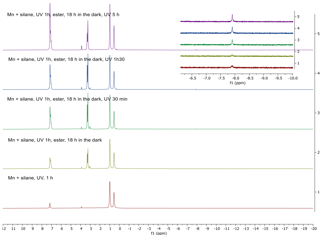
Figure 7. Monitoring over time of the reaction between \text{Mn}_2(\text{CO})_{10} and \text{Et}_3\text{SiH} (1 equiv.).
