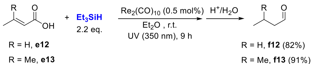
Scheme 18. Re 2 (CO) 10 catalyzed hydrosilylation of aliphatic α,β-unsaturated carboxylic acids to aldehydes.
