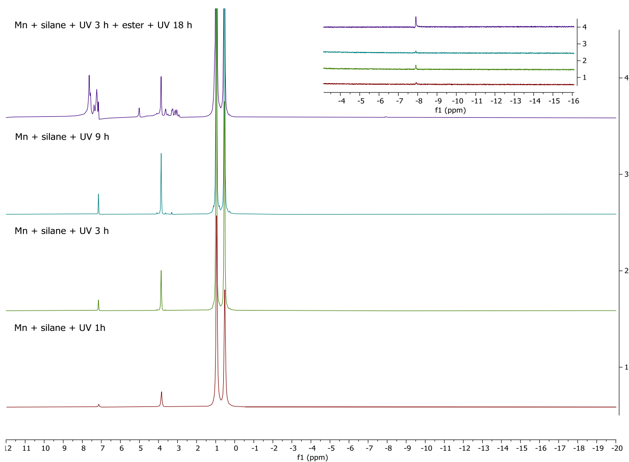
Figure 9. Monitoring over time of the reaction between \text{Mn}_2(\text{CO})_{10} and \text{Et}_3\text{SiH} (10 equiv.).
