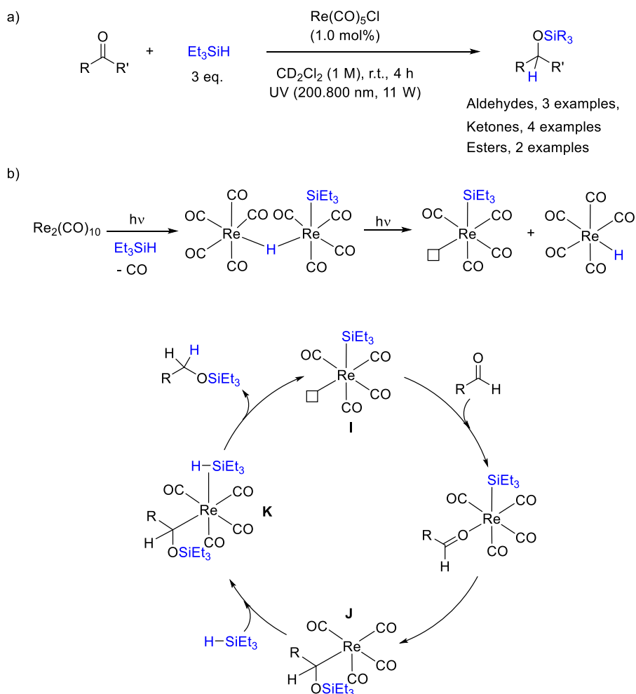
Scheme 14. Catalytic hydrosilylation of carbonyl compounds using \text{Re}(\text{CO})_5\text{Cl} as catalyst.
