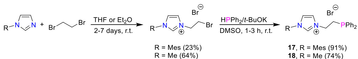
Scheme 14. Two-step synthesis of N-phosphino-imidazolium salts 17 and 18 from corresponding imidazole precursors. [51,52]
