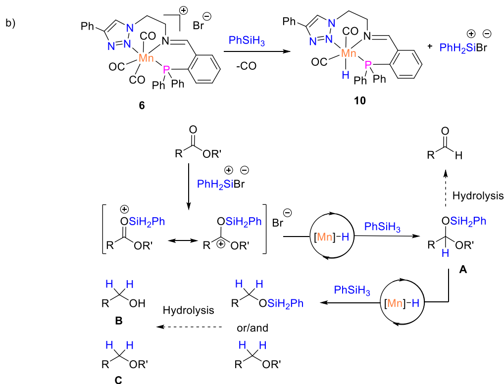
Scheme 7. Hydrosilylation of carboxylic acid derivatives catalyzed by Mn(I) complexes bearing triazole ligands.
