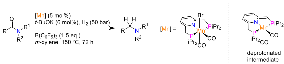
Scheme 7. Mn(I) catalyst featuring a PN- sp^2 P ligand for the hydrogenation of amides into amines.
