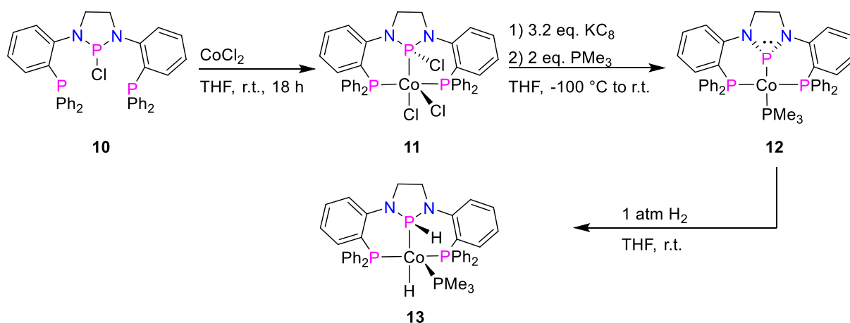
Scheme 7. Synthesis of pincer Co complexes 11 and 12 , and activation of \text{H}_2 bond by complex 12 to form the hydride complex 13 . [29]
