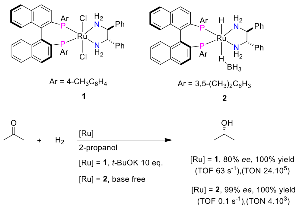
Scheme 3. Highly active chiral Ru–NH complexes for asymmetric hydrogenation of ketones. [13,15]
