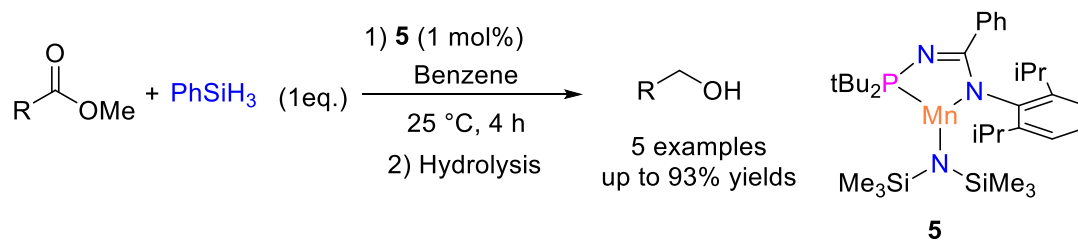
Scheme 6. Manganese complex catalyzed hydrosilylation of methyl benzoate derivatives.
