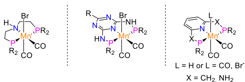
Scheme 1. General representation of Mn(I) pincer-type complexes featuring a PNP ligand.
