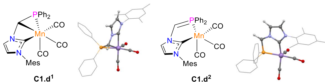
Figure 6. Structures and DFT optimized geometries of complexes C1.d 1 and fac - C1.d 2 (BP86/def2-TZVP, toluene SMD model).
