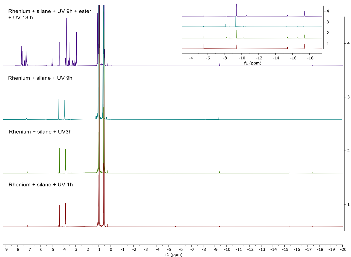
Figure 8. Monitoring over time of the reaction between \text{Re}_2(\text{CO})_{10} and \text{Et}_3\text{SiH} (10 equiv.).
