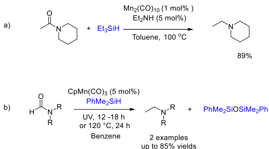
Scheme 9. Manganese-catalyzed reduction of amides with hydrosilanes.
