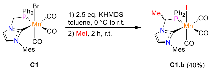
Scheme 34. Synthesis of NHC-phosphine complex C1.b from complex C1 .
