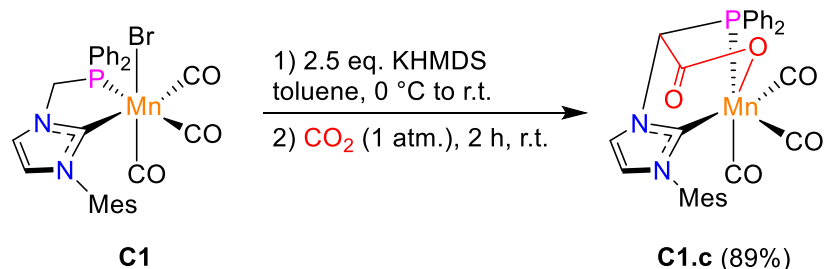
Scheme 35. Synthesis of NHC-phosphine Mn complex C1.c from complex C1 .
