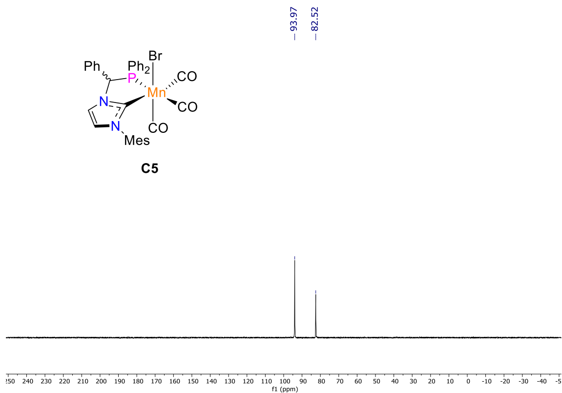
Figure 7. ^{31}\text{P}\{^1\text{H}\} NMR spectrum of Mn complex C5 (162.0 MHz, \text{CDCl}_3 , 25 °C).
