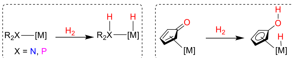
Scheme 2. H 2 activation by non-innocent ligands via metal-ligand cooperation.
