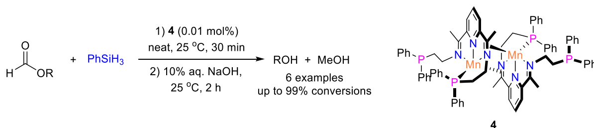
Scheme 5. Manganese-acyl catalyzed hydrosilylation of formates.
