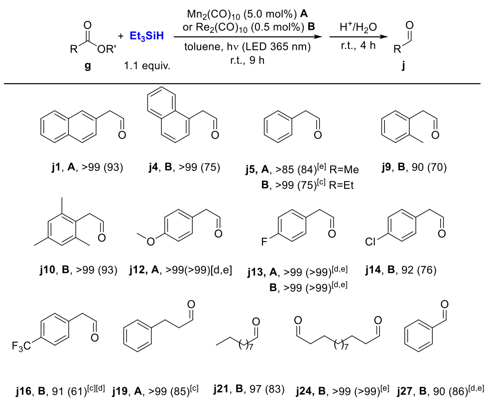
Scheme 23. Scope of the reduction of carboxylic esters g to aldehydes j . [a]
