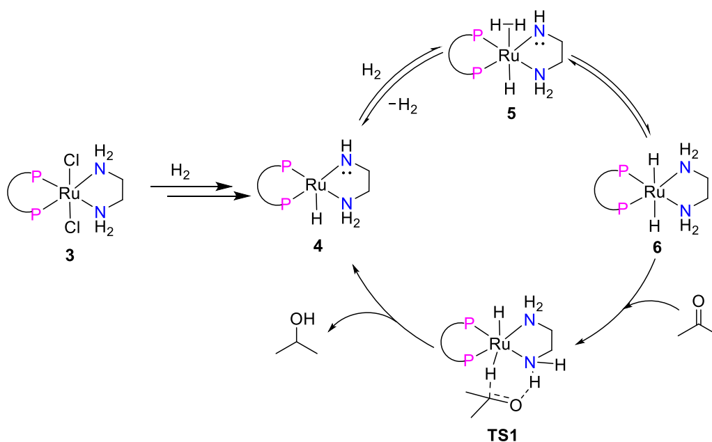
Scheme 4. Proposed mechanism for Ru–NH based-complexes in the catalyzed hydrogenation of ketones. [16,17]
