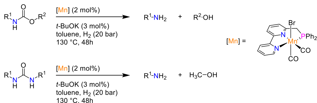
Scheme 13. Mn(I) complex based on a PNsp 2 N ligand for the hydrogenation of carbamates and ureas.
