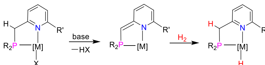
Scheme 8. Aromatization/de-aromatization process in Milstein pincer complexes.
