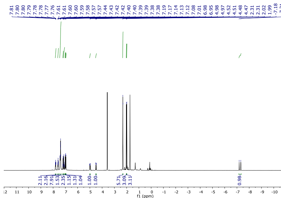
Figure 2. 1 H NMR spectrum of the hydride Mn complex C1.a (400.1 MHz, Tol, 25 °C).
