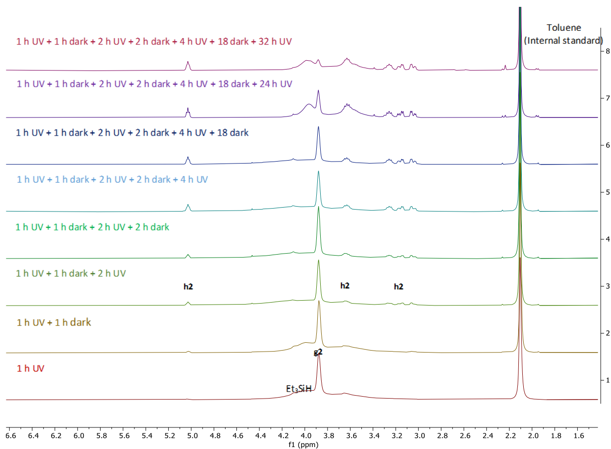
Figure 5. Monitoring over time of the “On-Off” experiment for the reduction of ester g2 with \text{Mn}_2(\text{CO})_{10} as catalyst.
