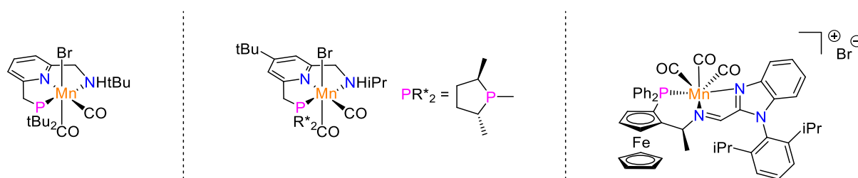
Scheme 12. Mn(I) complexes based on PN-sp 2 N ligand in the chiral and achiral series.
