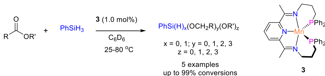
Scheme 4. Hydrosilylation of esters catalyzed by Mn complex 3 .
