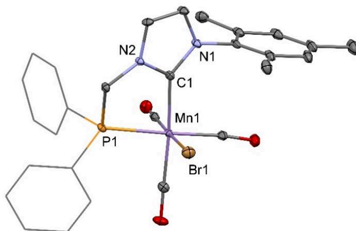
Figure 1. Molecular geometry of complex fac - C1 (30% probability ellipsoids, aryl groups represented as a wireframe for clarity, solvate THF molecule for complex fac - C1 not shown). Selected bond lengths ( \text{\AA} ) and angles ( ^\circ ): Mn1–C1 2.032(2), Mn1–P1 2.3030(7), Mn1–Br1 2.4125(6), C1–Mn1–P1 80.11(7), C1–Mn1–Br1 83.78(6), P1–Mn1–Br1 89.18(2).
