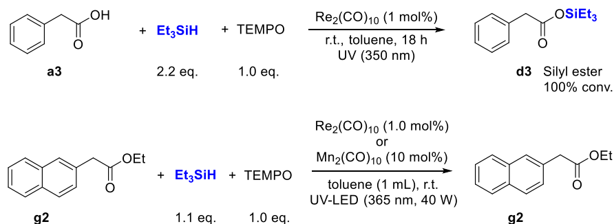
Scheme 24. Reduction of a3 and g2 in the presence of TEMPO.
