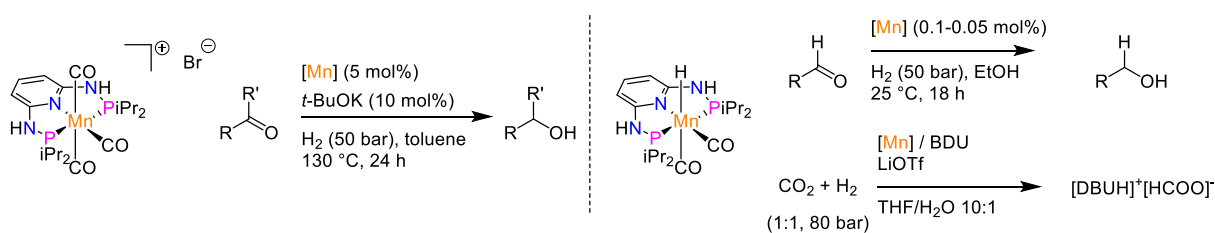
Scheme 6. Mn(I) complexes based on PN 3 P ligands for the hydrogenation of ketones ( left ), and aldehydes or CO 2 ( right ).
