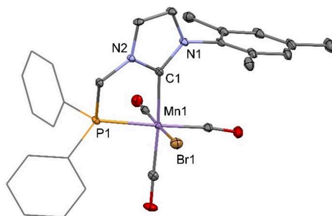
Figure 1. Structure moléculaire du complexe fac - C1 (30% probability ellipsoids, aryl groups represented as a wireframe for clarity). Selected bond lengths (Å) and angles (°): Mn1–C1
