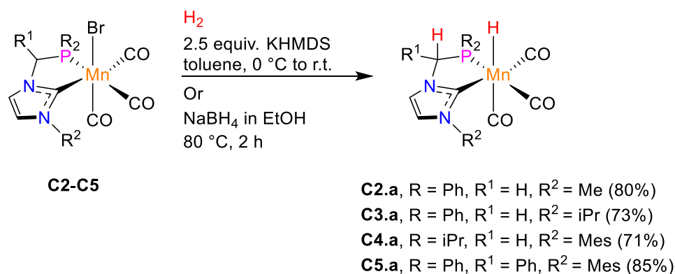
Scheme 44. Synthesis of Mn hydride complexes C2.a-C5.a from their corresponding bromide precursors C2-C5 .
