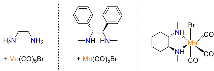
Scheme 16. N-sp 3 ,N-sp 3 ligands involved in hydrogenation-type reactions.
