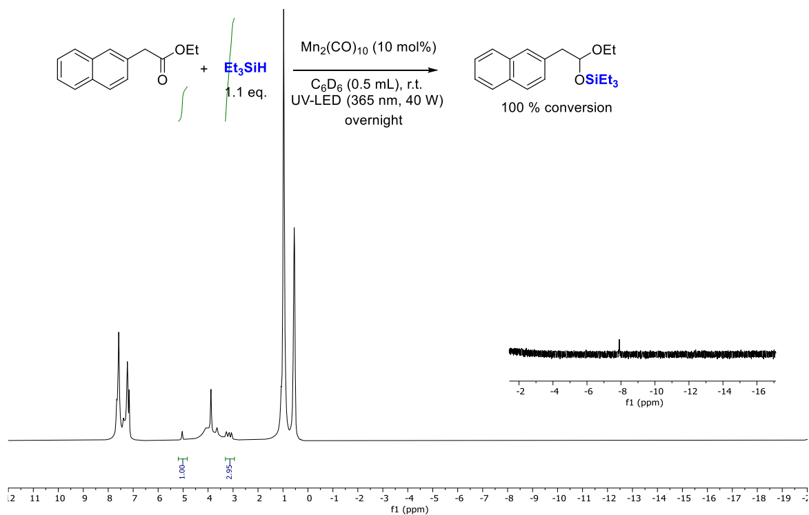
Figure 11. Crude NMR spectra of the catalytic mixture with 10 mol% \text{Mn}_2(\text{CO})_{10} .
