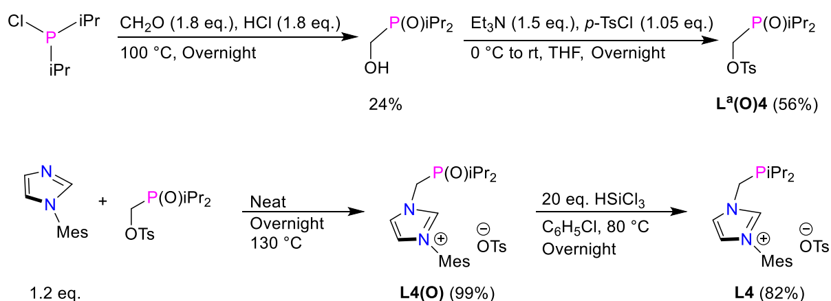
Scheme 41. Synthesis of the N-phosphino-imidazolium salt L4 from diisopropyl(chloro)phosphine.
