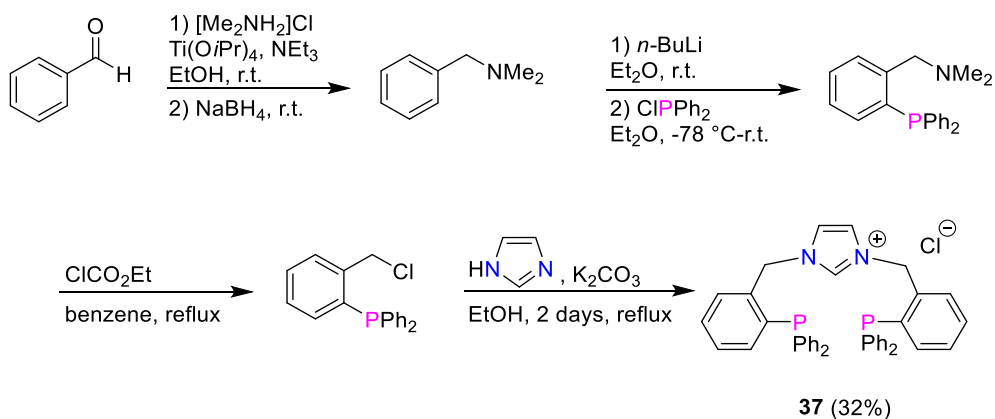
Scheme 26. Synthesis of the NHC core pincer pre-ligand 37 from benzaldehyde. [70]
