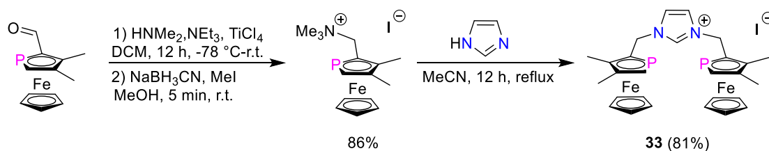
Scheme 24. Synthesis of the tridentate NHC phosphine pincer ligand 33 exhibiting two ferrocenyl side arms. [64]
