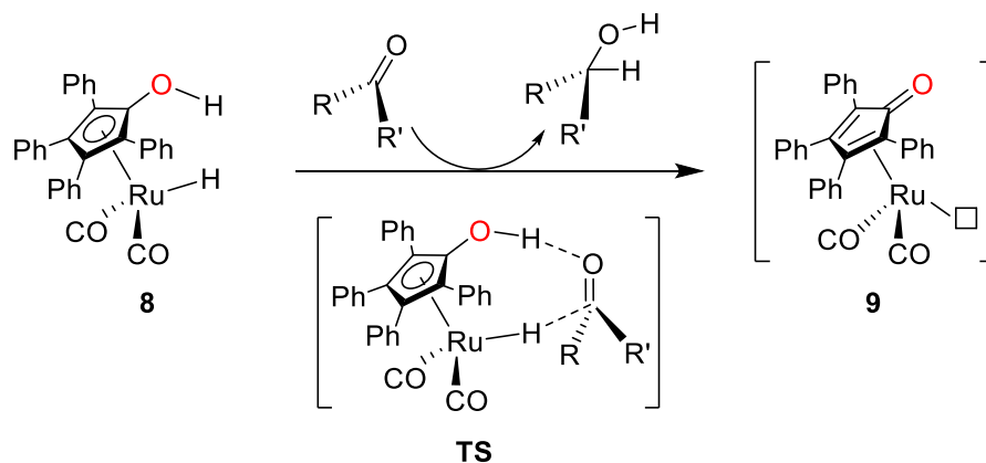
Scheme 6. Proposed mechanism for carbonyl hydrogenation by Shvo catalyst. [26]
