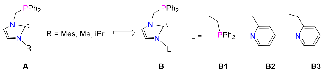
Scheme 50. Representation of previously prepared bidentate NHC-phosphine ligands A , and related targeted tridentate NHC core systems of type B .
