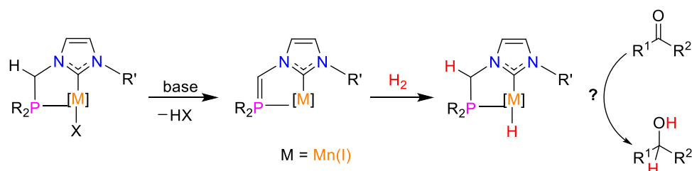
Scheme 11. H 2 activation by non-innocent ligands of NHC-phosphine type via metal-ligand cooperation.
