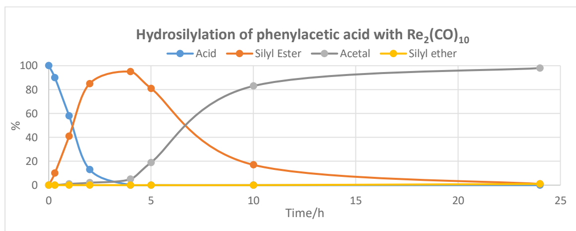
Figure 1. Monitoring over time of the reduction of phenyl acetic acid a3 .
