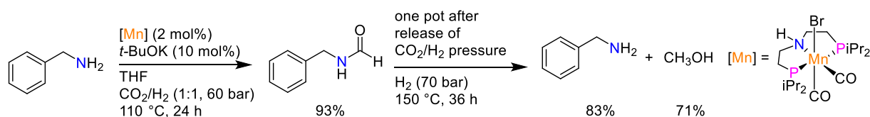
Scheme 3. Mn(I) pincer complex featuring a PN-sp 3 P ligand for the hydrogenation of CO 2 to CH 3 OH.
