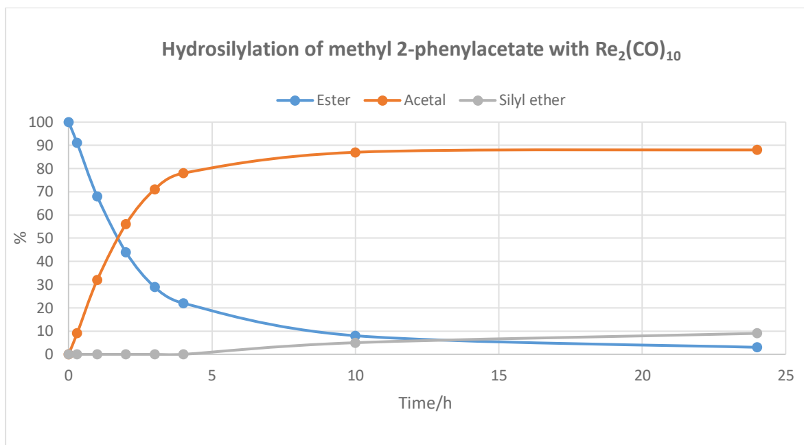
Figure 2. Kinetic monitoring of reaction between 2-phenylacetate g5 and Et 3 SiH catalyzed by Re 2 (CO) 10 .
