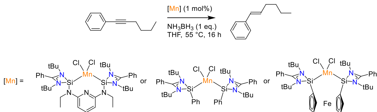
Scheme 24. Mn(II) complexes featuring Si-based ligands for the semi-hydrogenation of alkynes.
