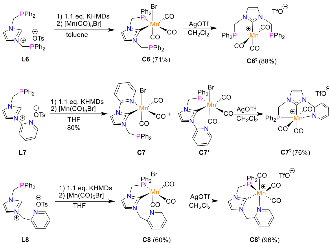
Scheme 52. Syntheses of cationic tridentate NHC core Mn(I) complexes C6 t , C7 t , and C8 t from corresponding PCP L6 and PCN ligand precursors L7 and L8 .
