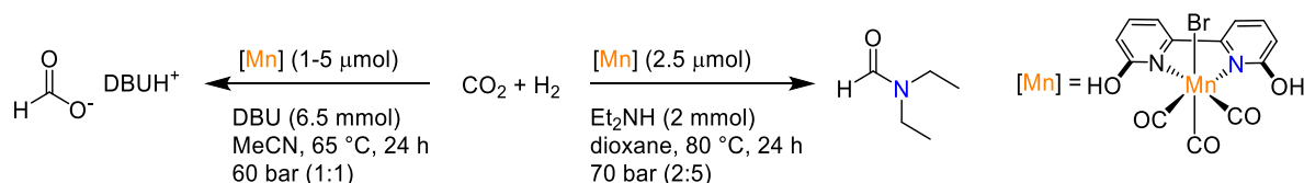
Scheme 17. Mn(I) complex based on a N-sp 2 ,N-sp 2 ligand for the hydrogenation of CO 2 .
