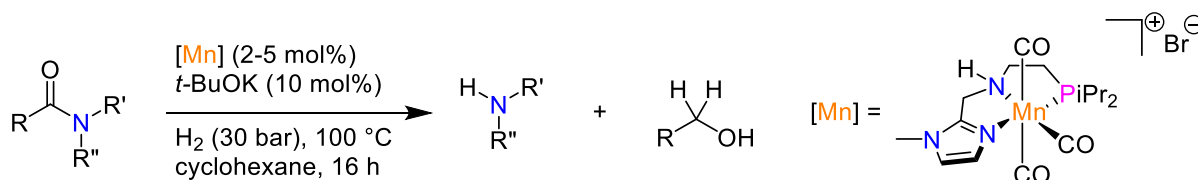
Scheme 9. Mn(I) complex of a PN-sp 3 N ligand for the hydrogenation of amides.
