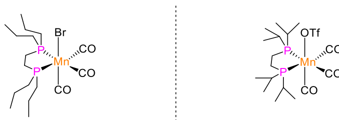
Scheme 19. Mn(I) complexes bearing bidentate PP ligands for hydrogenation reactions.
