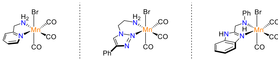
Scheme 18. Mn(I) complexes bearing N-sp 2 ,N-sp 3 ligands for hydrogenation-type reactions.
