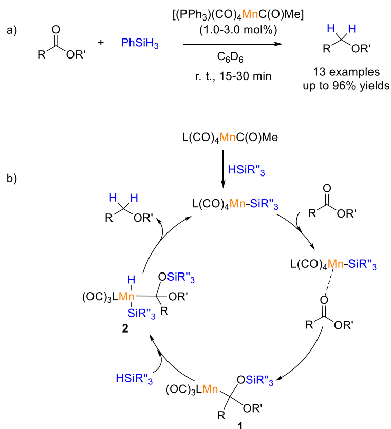
Scheme 3. Manganese-acyl catalyzed hydrosilylation of esters.
