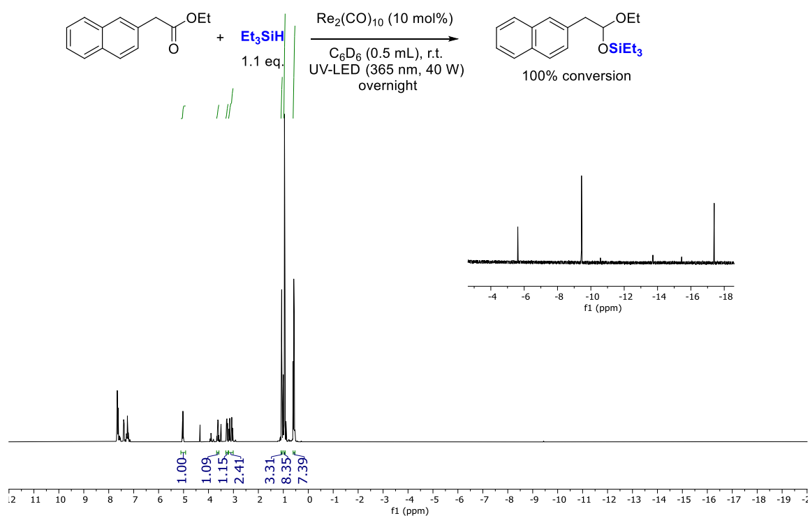
Figure 10. Crude NMR spectra of the catalytic mixture with 10 mol% \text{Re}_2(\text{CO})_{10} .
