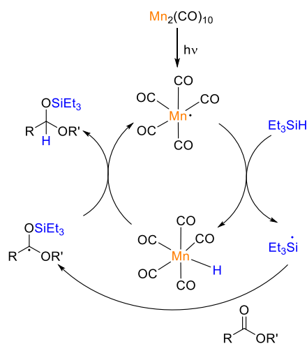
Scheme 25. Proposed catalytic cycle for the hydrosilylation of acids and esters with Mn_2(CO)_{10} .
