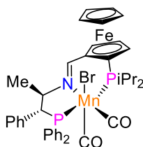
Scheme 8. Mn(I) complex of a chiral PN- sp^2 P ligand for the enantioselective transfer hydrogenation.
