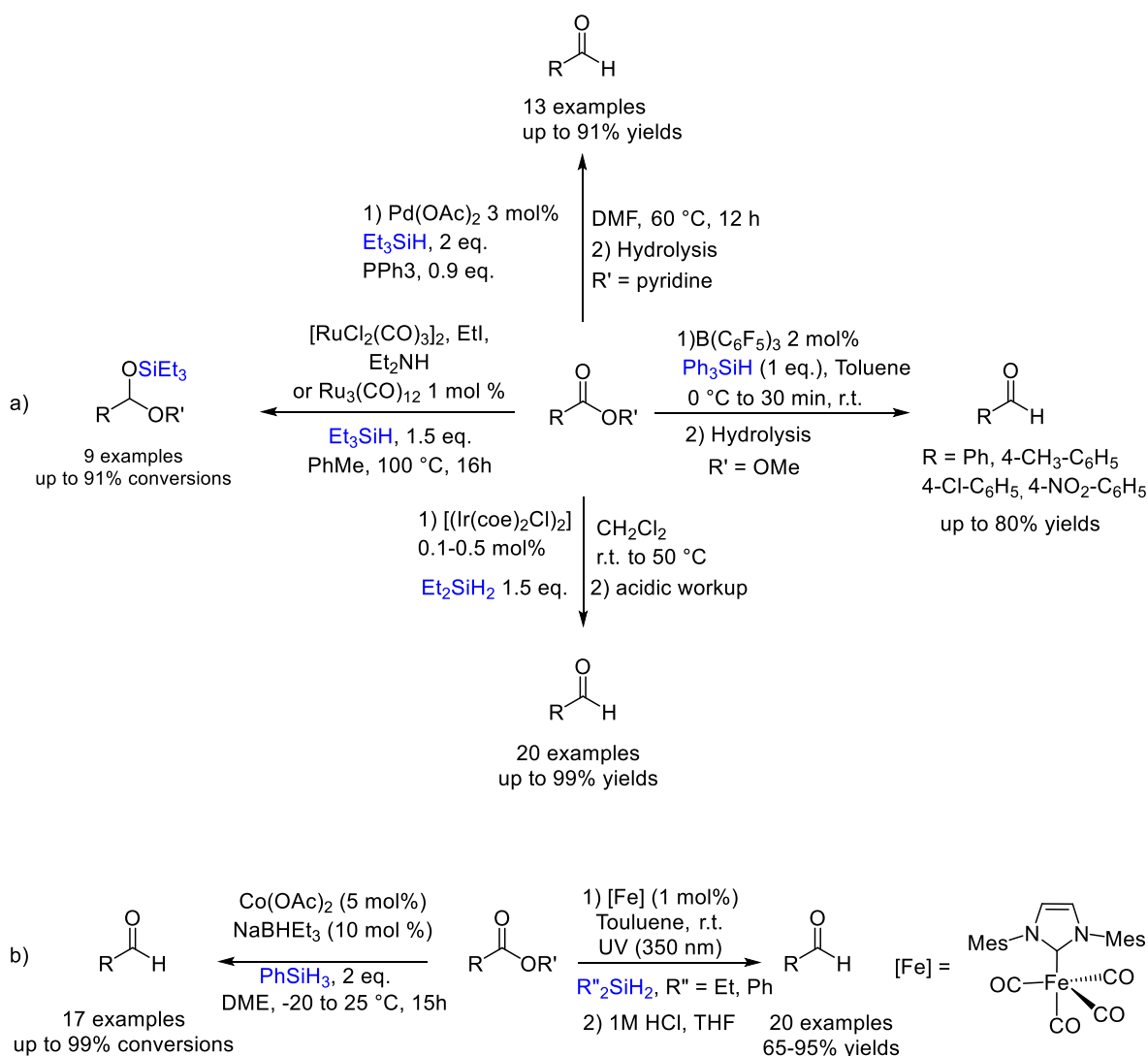
Scheme 1. Hydrodesilylation of esters into aldehydes.
