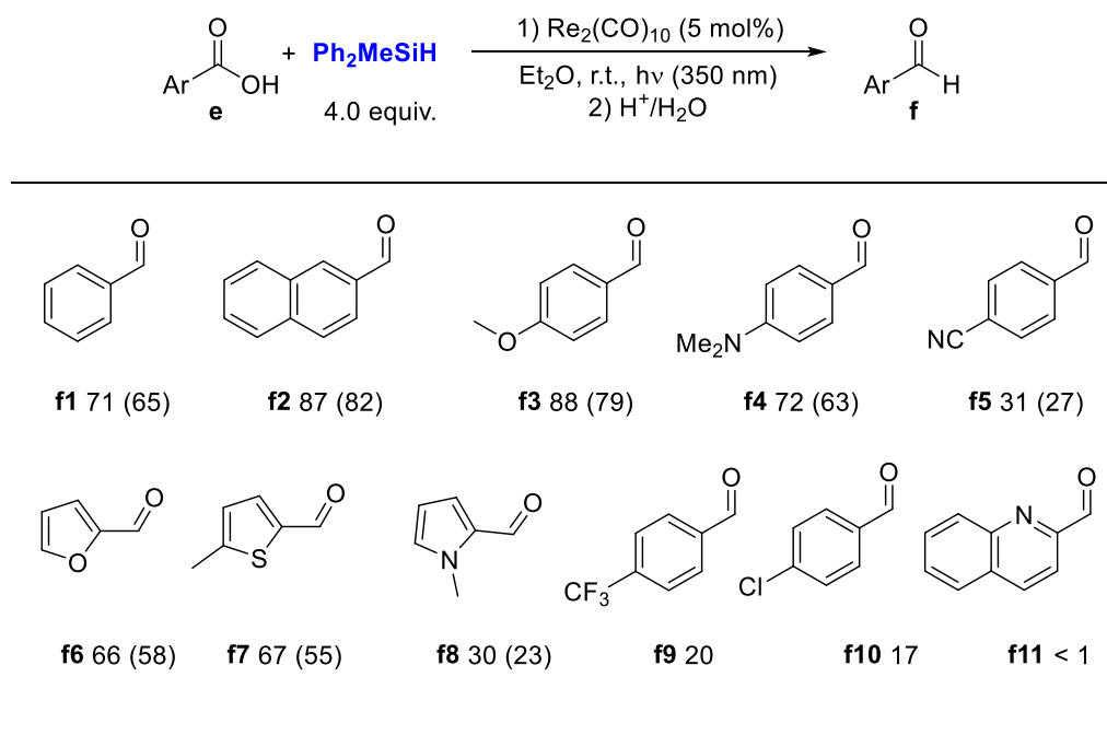
Scheme 17. Scope of the reduction of aromatic carboxylic acids to aldehydes. [a]
