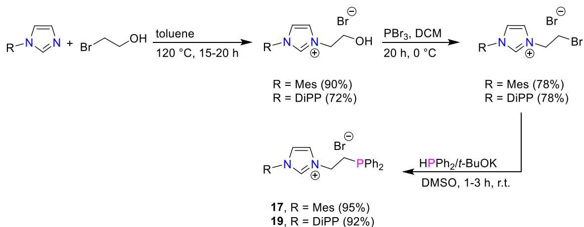
Scheme 15. Synthesis of N-phosphino imidazolium salts 17-19 by an alternative method. [53,54]
