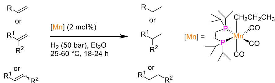
Scheme 20. Mn(I) complex of a bidentate PP ligand for the hydrogenation of alkenes.
