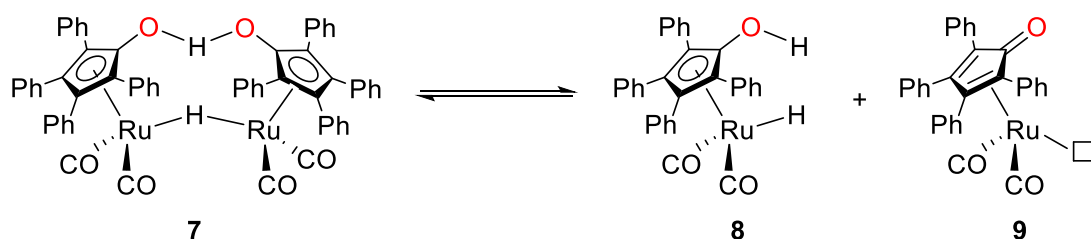
Scheme 5. Shvo's catalyst 7 in equilibrium with its active monomers 8 and 9 . [25]
