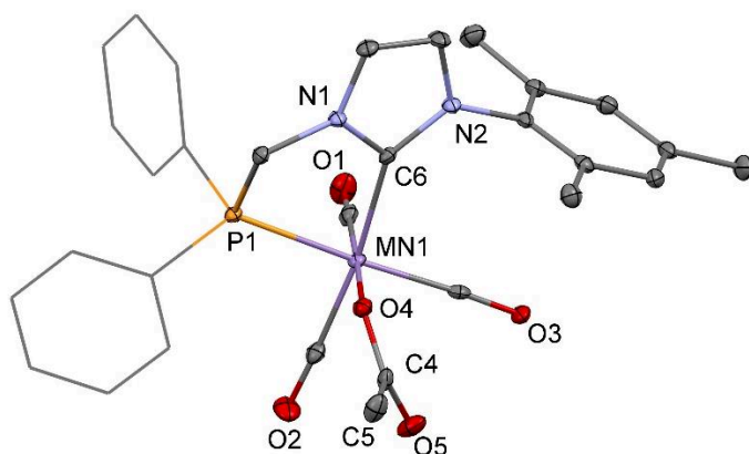
Figure 9. Molecular geometry of complex fac - C1.h (30% probability ellipsoids, aryl groups represented as a wireframe for clarity). Selected bond lengths (Å) and angles (°): Mn1–C6 2.048 (3), Mn1–P1 2.2997 (9), Mn1–O4 2.0623 (18), C6–Mn1–P1 79.10 (7), C6–Mn1–O4 84.07 (9), P1–Mn1–O4 84.58 (5).
