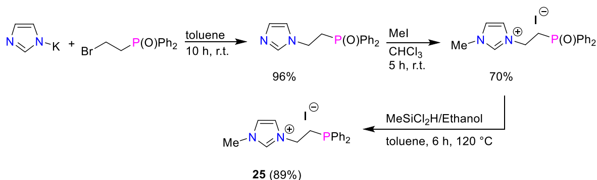
Scheme 19. Synthesis of N-tethered phosphino-imidazolium salt 25 . [58]
