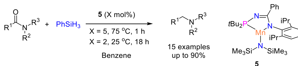
Scheme 10. Manganese complex 5 catalyzed hydrosilylation of amides.
