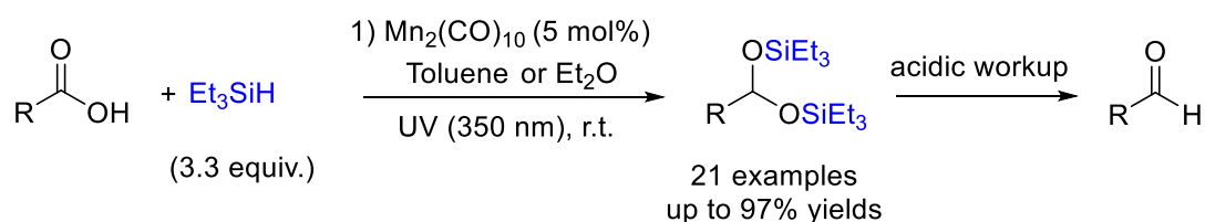
Scheme 11. Manganese carbonyl complex catalyzed hydrosilylation of carboxylic acids.
