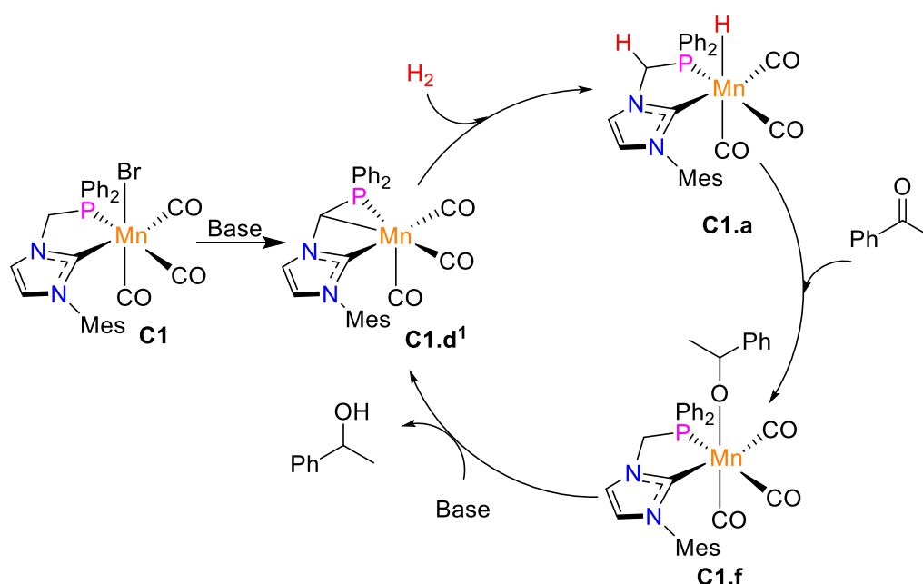
Scheme 45. Proposed mechanism for the catalytic hydrogenation of acetophenone with NHC-phosphine Mn(I) complex C1 .
