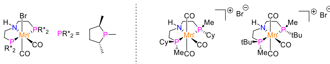
Scheme 4. Mn(I) complexes of chiral PN-sp 3 P ligands involved in enantioselective hydrogenation.
