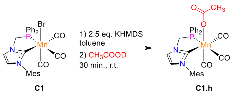
Scheme 49. Deprotonation of the bromide Mn complex C1 followed by the addition of 1 equiv. of deuterated acetic acid.
