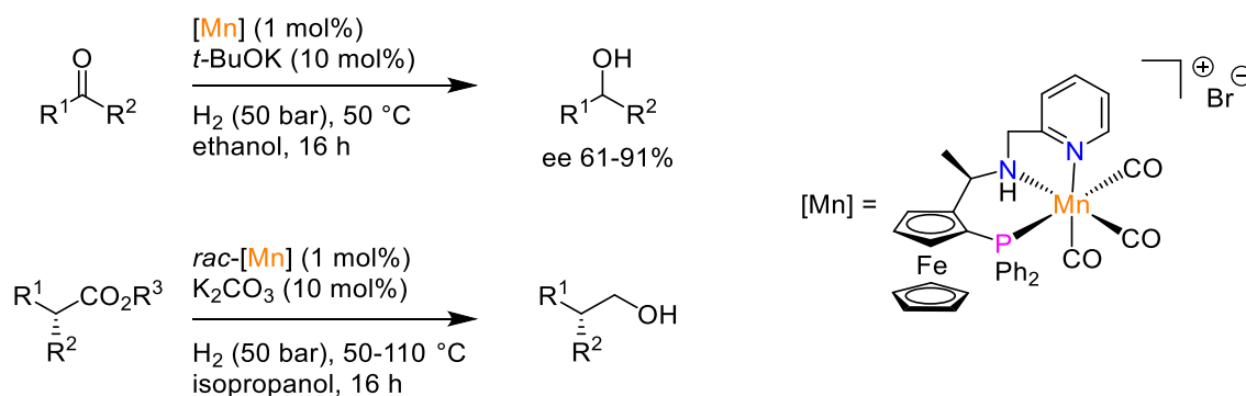
Scheme 11. Mn(I) complex of a chiral PN- sp^3 N ligand for the enantioselective reduction of ketones and \alpha -chiral esters.
