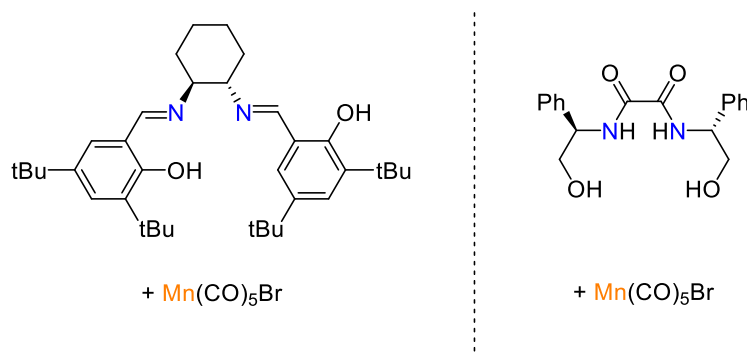
Scheme 25. Polydentate systems combining N- and O- donor atoms for the hydrogenation of ketones.
