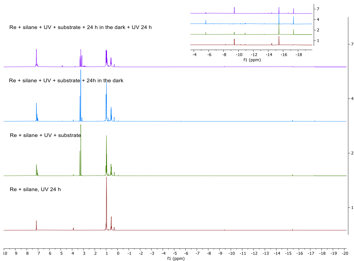
Figure 6. Monitoring over time of the reaction between \text{Re}_2(\text{CO})_{10} and \text{Et}_3\text{SiH} (1 equiv.).
