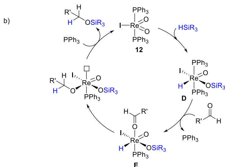
Scheme 12. Rhenium(V)-dioxo complex catalyzed hydrosilylation reaction of ketones and aldehydes.
