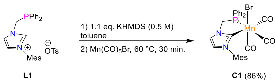
Scheme 31. Synthesis of NHC-phosphine Mn complex C1 from pre-ligand L1 .
