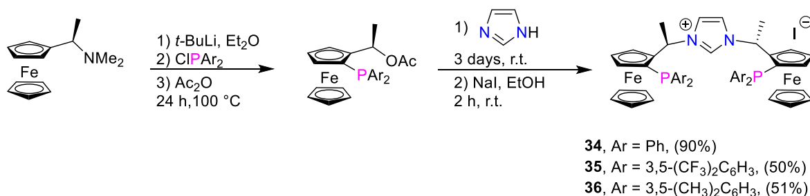
Scheme 25. Synthesis of the tridentate NHC core pincer ligands 34-36 from N,N -dimethyl-1-ferrocenylethylamine. [65-69]
