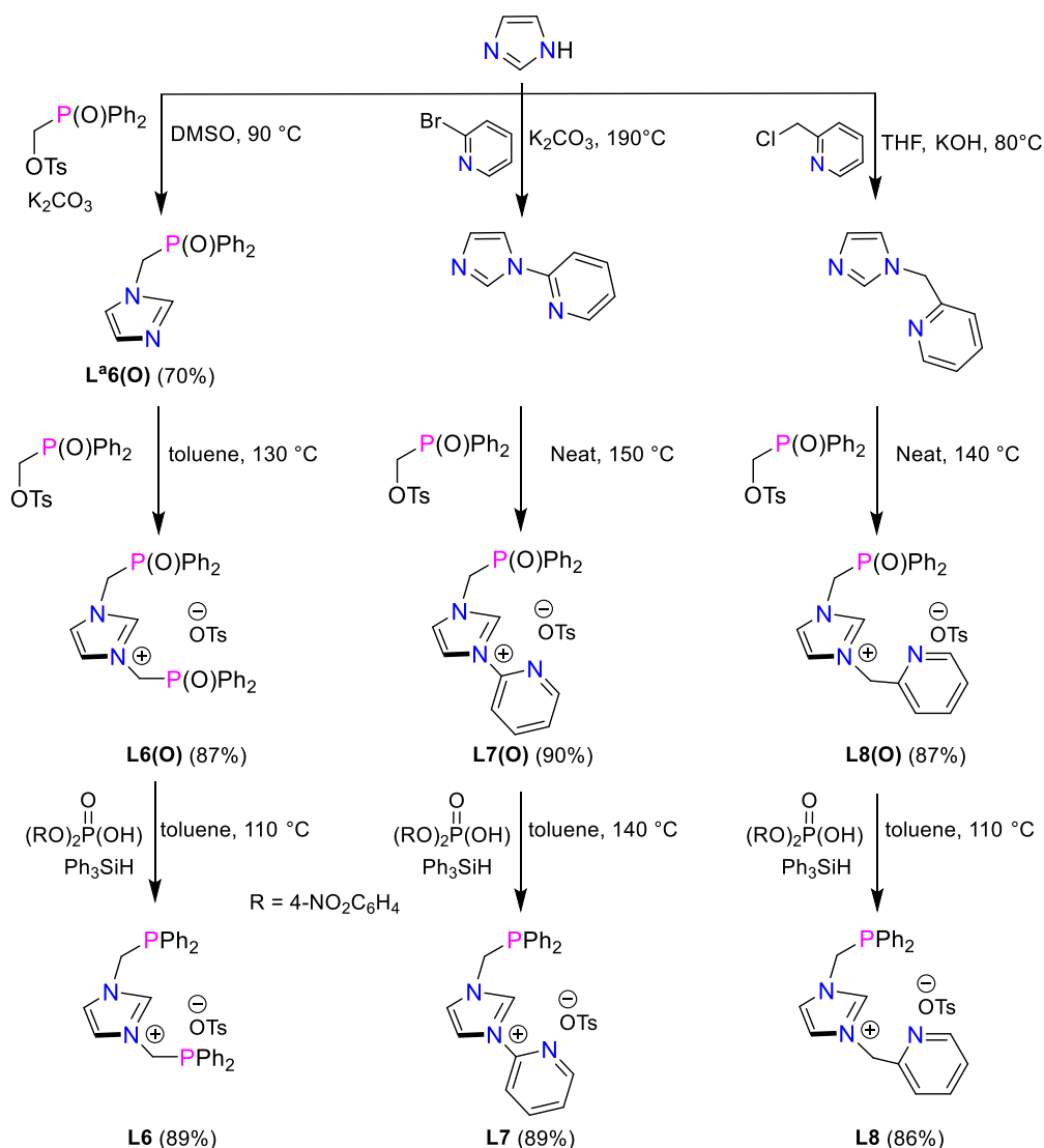
Scheme 51. Preparation of tridentate PCP and PCN pre-ligands L6 , L7 and L8 from 1 H -imidazole.
