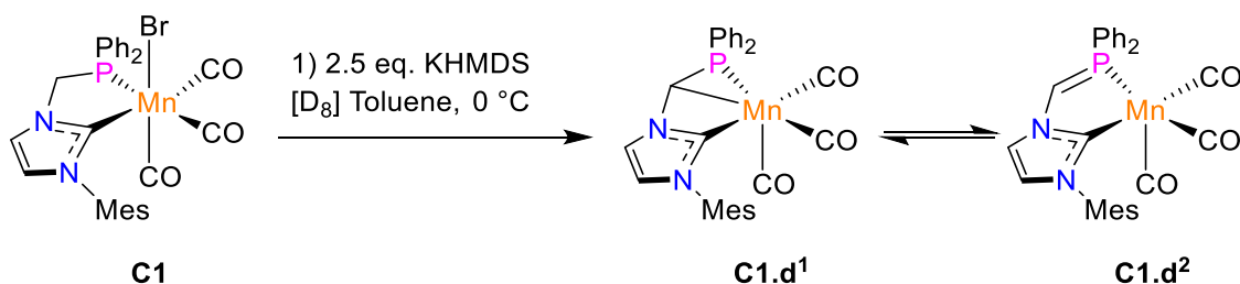
Scheme 36. Deprotonation of complex C1 to characterize the intermediate complex C1.d .
