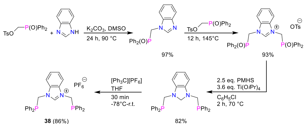
Scheme 27. Synthesis of the NHC core pre-ligand 38 through sequential introduction of the two side arms. [71]
