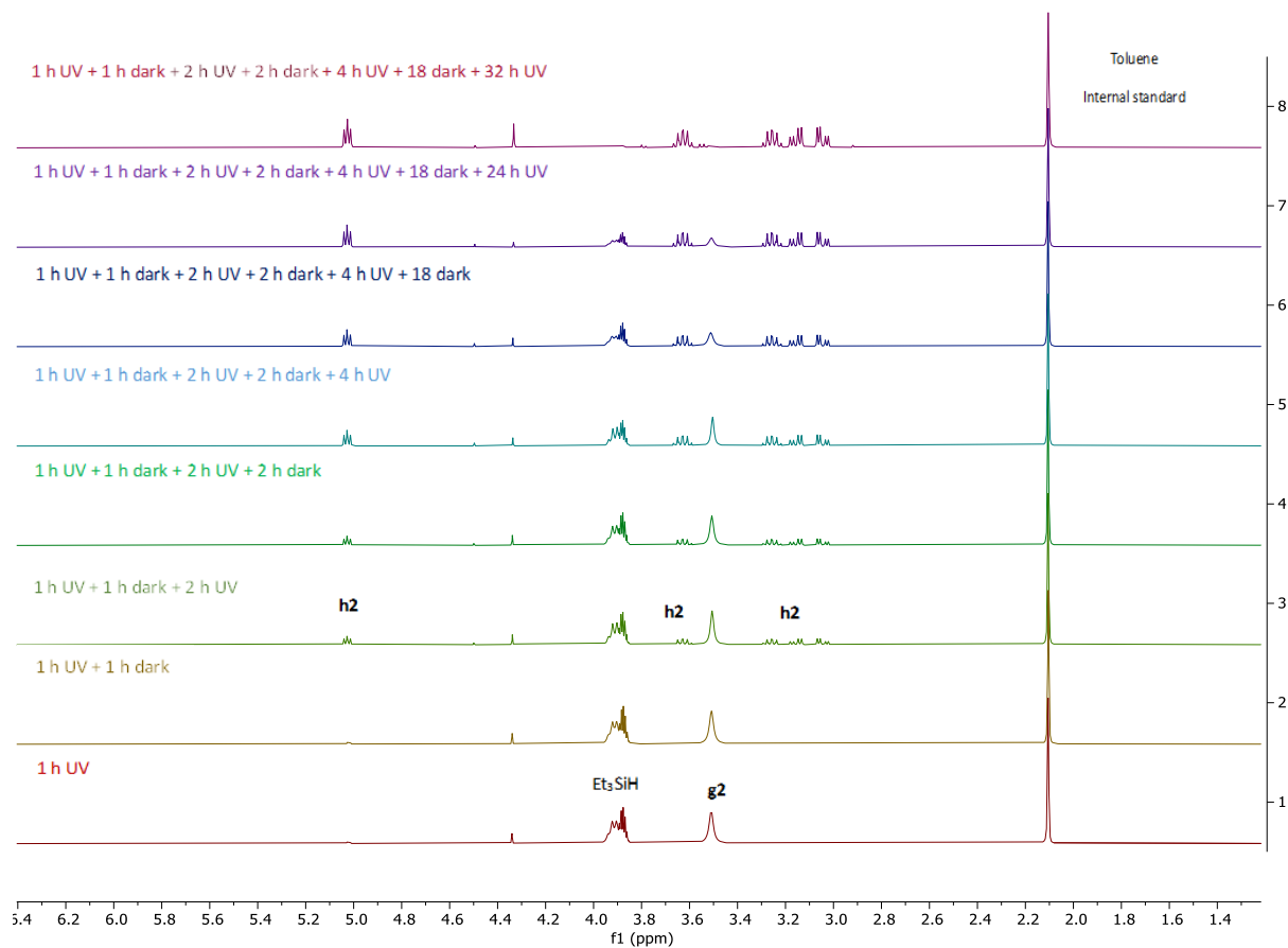
Figure 4. Monitoring over time of the “On-Off” experiment for the reduction of ester g2 with \text{Re}_2(\text{CO})_{10} as catalyst.
