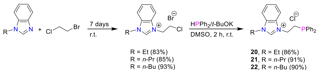
Scheme 16. Synthesis of N-phosphino-benzimidazolium salts 20-22 . [55]
