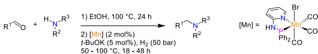
Scheme 22. Mn(I) complex featuring a PN ligand for the reductive amination of aldehydes.
