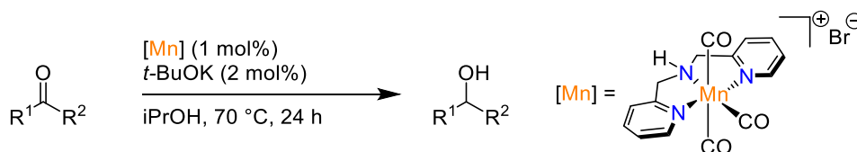
Scheme 14. Mn(I) complex of a NN-sp 3 N pincer ligand for the transfer hydrogenation of ketones.
