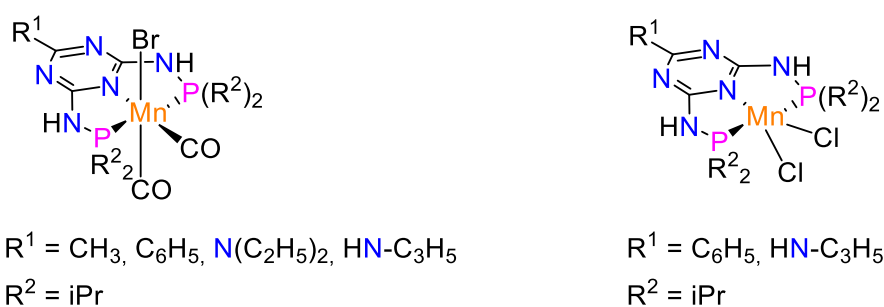
Scheme 5. PN 5 P Mn(I) complexes for the hydrogenation of carbonyl derivatives.
