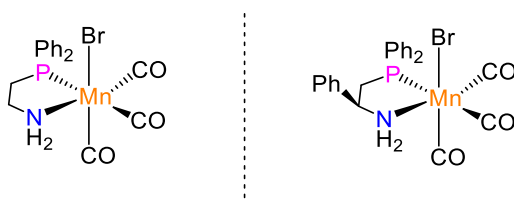
Scheme 21. Mn(I) complexes based on bidentate NP ligands in hydrogenation reactions.
