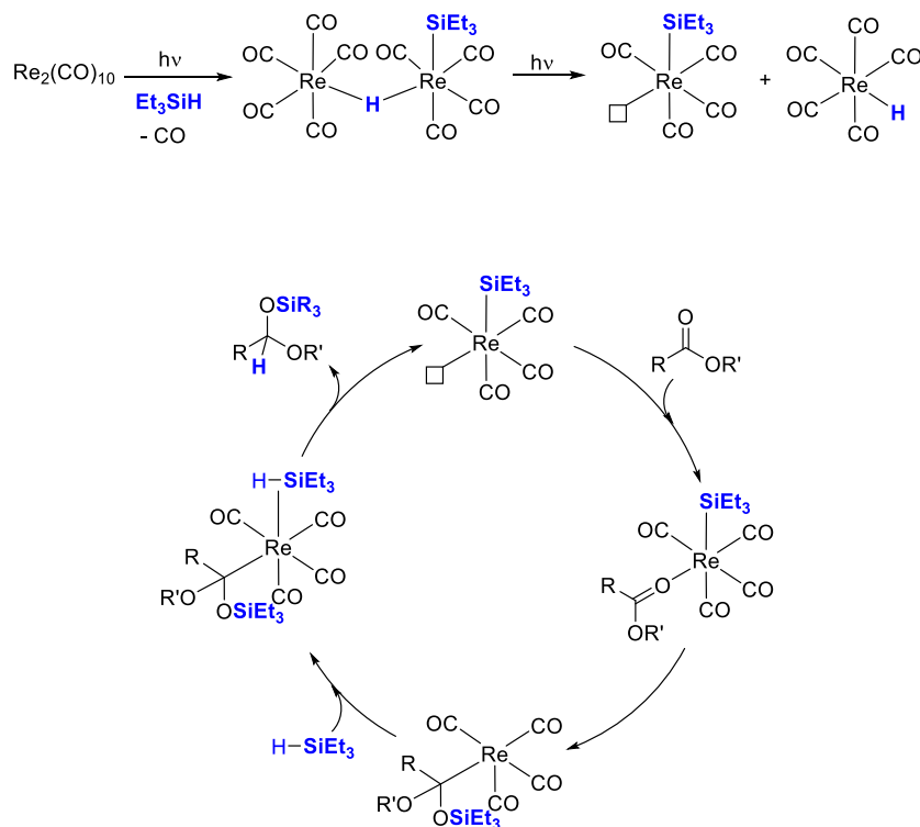
Scheme 26. Proposed catalytic cycle for the hydrosilylation of acids and esters with \text{Re}_2(\text{CO})_{10} .
