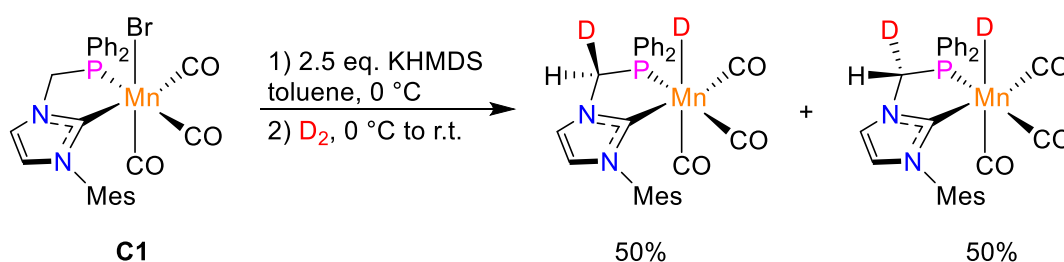
Scheme 33. D_2 activation by NHC-phosphine Mn complex C1 .
