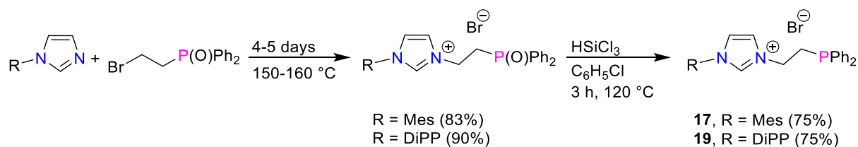
Scheme 18. Synthesis of N-phosphino-imidazolium salts 17 and 19 . [57]
