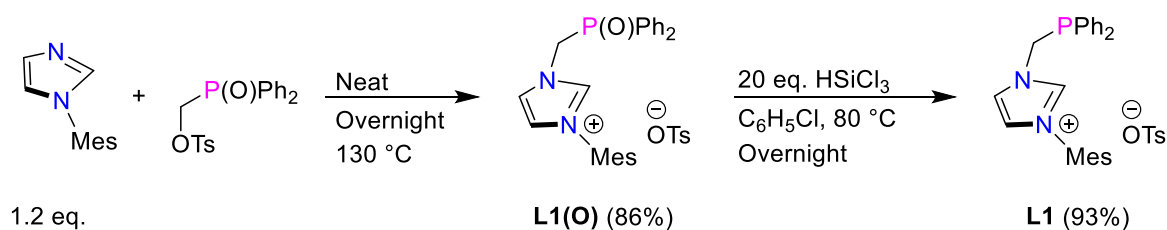
Scheme 30. Synthesis of the N-phosphino-imidazolium salt L1 from 1-mesityl-imidazole.
