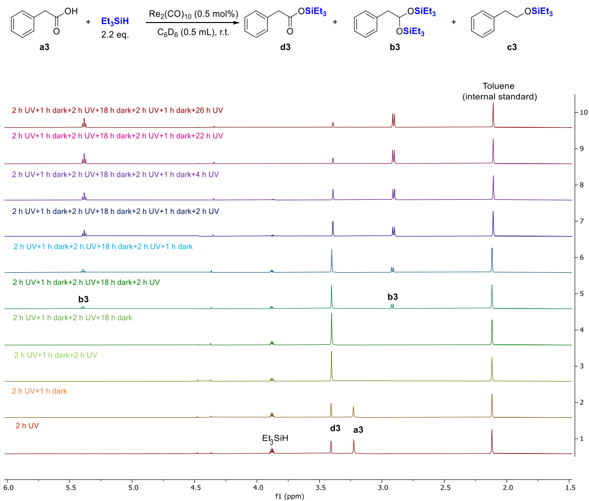
Figure 3. Monitoring over time of the “On-Off” experiment for the reduction of the carboxylic acid a3 .
