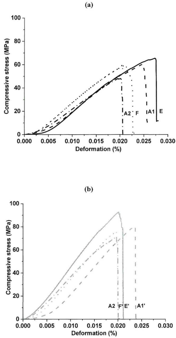
Figure 4: compressive stress value ( \pm 5 MPa) as a function of deformation ( \pm 0.001 %) for (a) (K) formulations and (b) (KNa) geopolymer formulations
