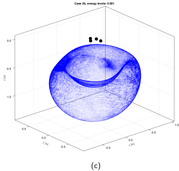
Figure 3.7 – Computed equilibria, simulations around the saddle and connectivity tree for Case 2b. (a): 3D view, computed equilibria and heteroclinic orbits for the pseudo-inverse (solid) and transpose (dashed) controllers. (b): connectivity tree, with the two critical levels highlighted. (c): paving of the energy’s level set at 0.1c_S , with c_S being S ’s energy level.
