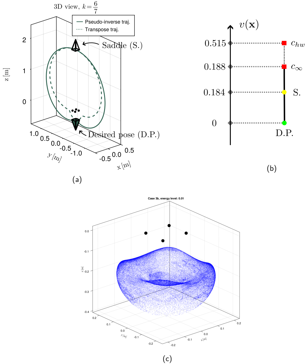
Figure 3.11 – Computed equilibria, simulations around the saddle and connectivity tree for Case 3b. (a): 3D view, computed equilibria and heteroclinic orbits for the pseudo-inverse (solid) and transpose (dashed) controllers. (b): connectivity tree, with the two critical levels highlighted. (c): paving of the energy’s level set at 0.06c_S , with c_S being S ’s energy level.
