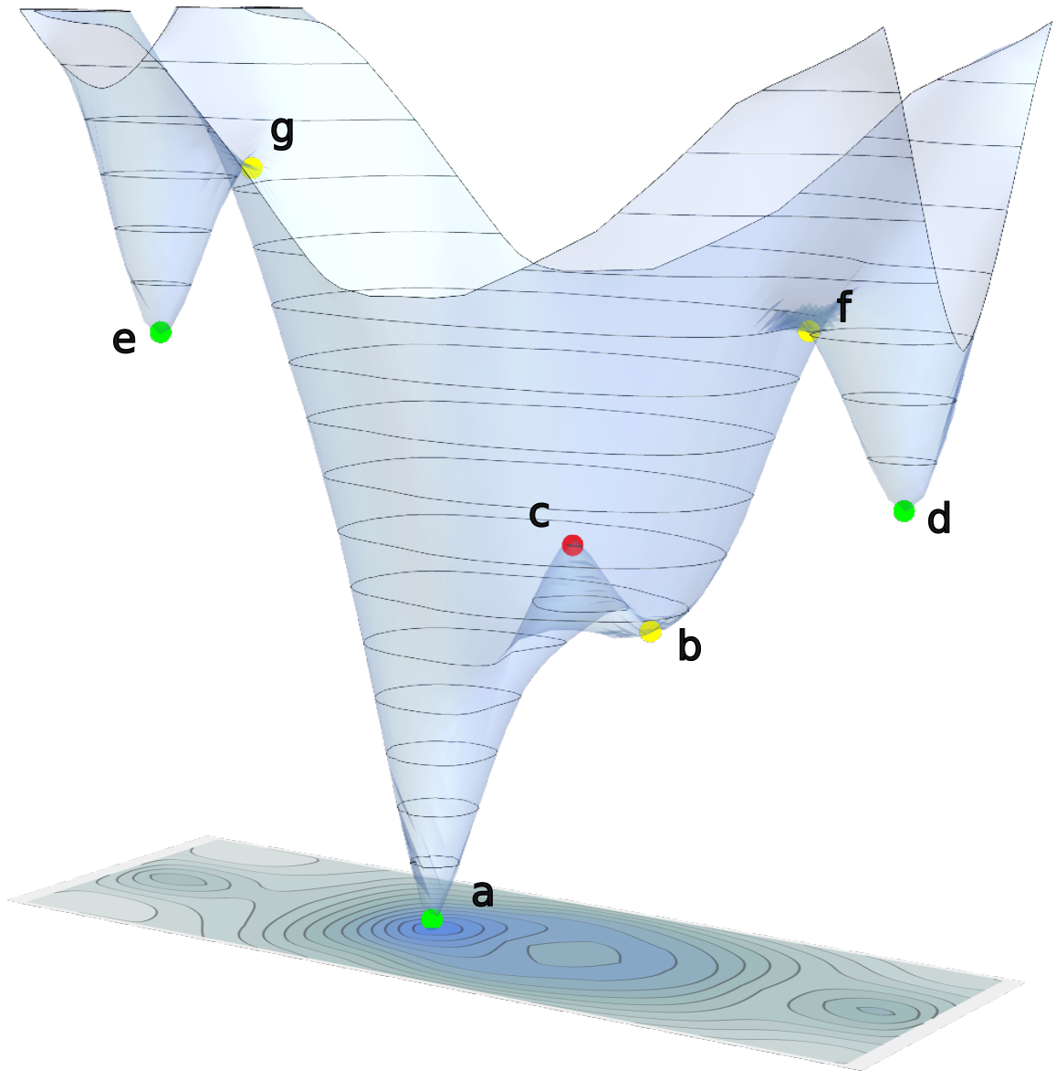
Figure 1.6 – An example of energy function with non-trivial regions of attraction. Highlighted points represent its critical points, where green points are minima, yellow ones are saddles and the red one is a maximum. The letters are ordered according to the energy level.
