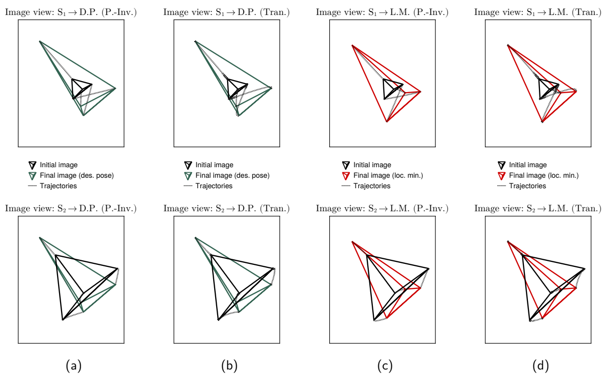
Figure 3.4 – Heteroclinic orbits for Case 1b in image view, for the pseudo-inverse ((a) and (c)) and transposed ((b) and (d)) controllers.
