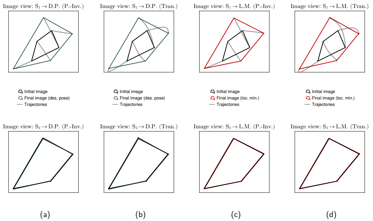
Figure 3.6 – Heteroclinic orbits for Case 2a in image view, for the pseudo-inverse ((a) and (c)) and transpose ((b) and (d)) controllers.
