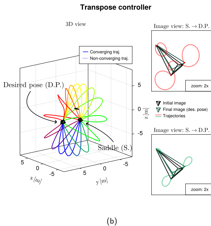
Figure 4.2 – Computed equilibria and simulations around the saddle for Case 1b. (a): computed equilibria and a selection of heteroclinic orbits, both in 3D and image space, for the pseudo-inverse controller. (b): idem for the transpose controller.
