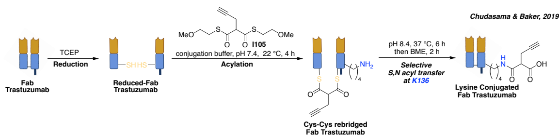
Scheme 24. Lysine site-selective labelling of Fab-Trastuzumab via NCL.
