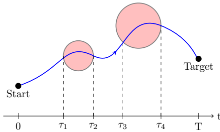
(a) The state x (in blue) traverses two loss control regions (in red) to reach the target.
