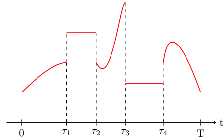
(b) The control u (in red) is permanent on control regions and frozen in loss control regions.
