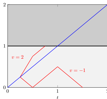
Figure 2.5: Illustration of the counterexample given in Item 2 of Section 2.2.3.
