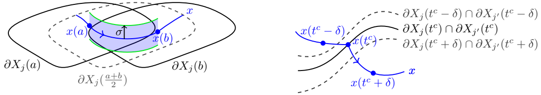
Figure 2.1: Illustrations of Condition (C1) on the left, and of Condition (C2) on the right.
