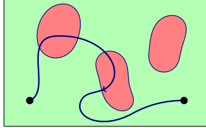
Figure 2: A state visits regions (in red) where permanent controls are not allowed, only constant ones.
