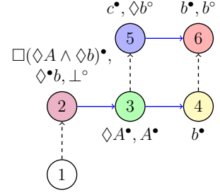
Figure 5.1: On the left: Proof in \text{labS4}_\leq of \square(\diamond A \wedge \diamond b) \supset \perp with A = (c \supset \diamond b) \supset \perp , \Gamma = \{\square(\diamond A \wedge \diamond b), \diamond b\} and \mathfrak{G} = 1 \leq 2, 2R2, 2R3, 3 \leq 3, 2:\Gamma, 3:\perp \implies 2:\perp . On the right: Diagrammatic representation of the top left sequent in the derivation.
