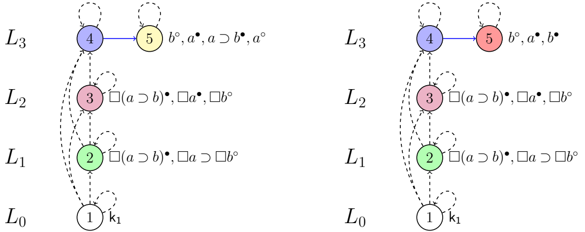
Figure 5.2: Proof search algorithm
