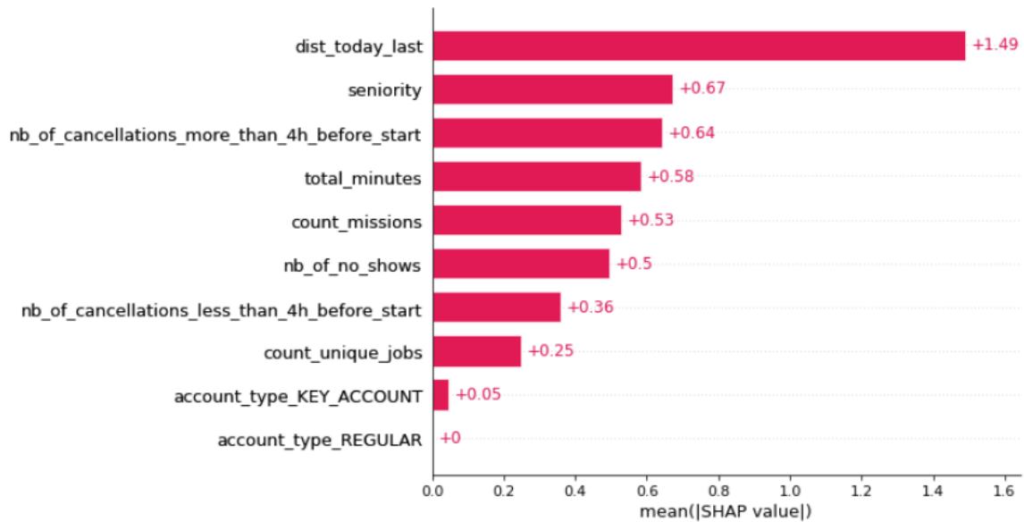
Figure 5.10 : Importance plot
