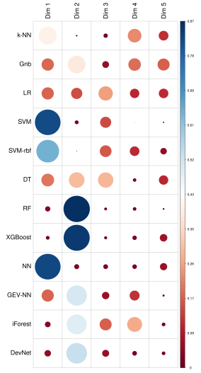
(b) Representation Quality
