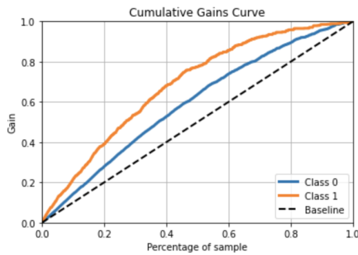
(a) LIFT for XGB
