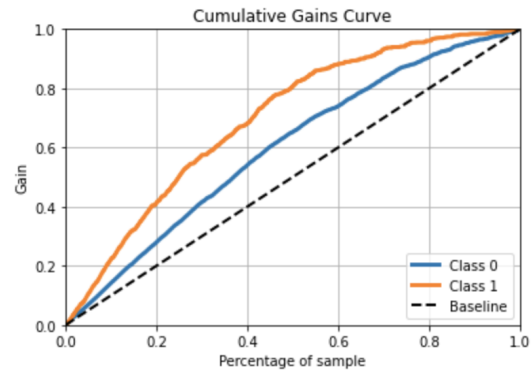
(b) LIFT for LR
