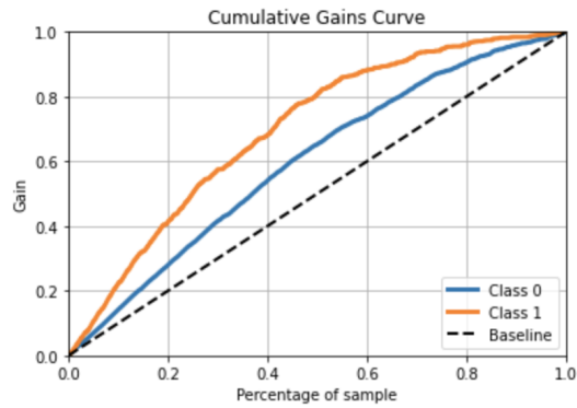
(a) LIFT for RF
