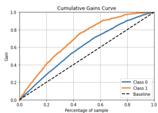
(b) LIFT for Ensemble
