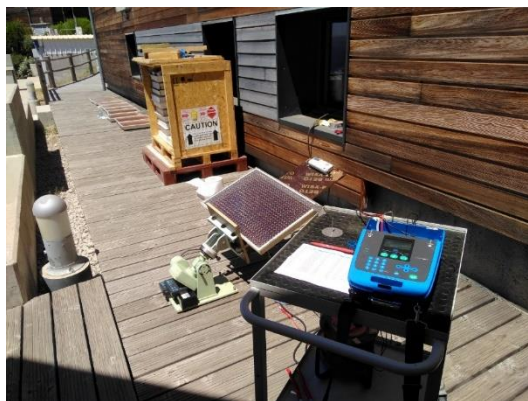
Figure 3-22: I-V curve tracing with the HCPV modules
