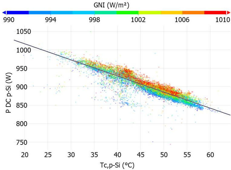
Figure 5-2: Scatter plot with regression line; p-Si
