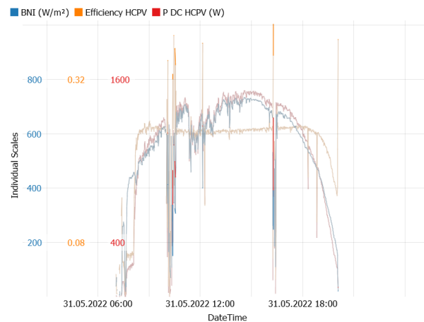
Figure C-33: Time series plot referring to the scatter plot in Fig. C-32
