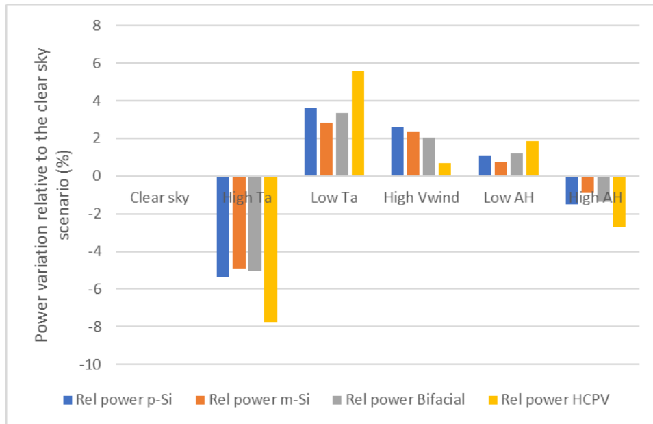
Figure 5-16: Power variations relative to the clear-sky scenario, per scenario and PV technology
