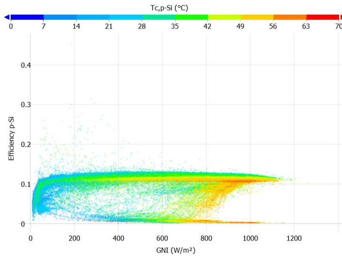
Figure 4-2: p-Si efficiency with basic and power filters
