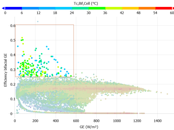
Figure C-19: Selecting high-efficiency sparse data records.
