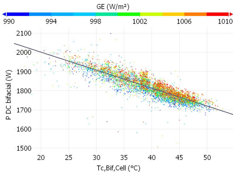
Figure 5-4: Scatter plot with regression line; bifacial
