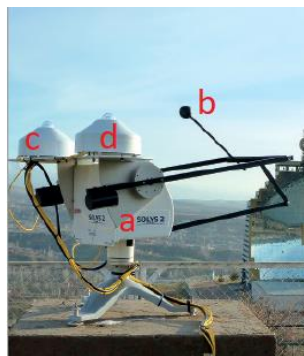
Figure 2-13: Assembly to measure GHI and DHI
