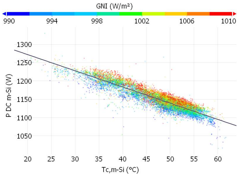
Figure 5-3: Scatter plot with regression line; m-Si
