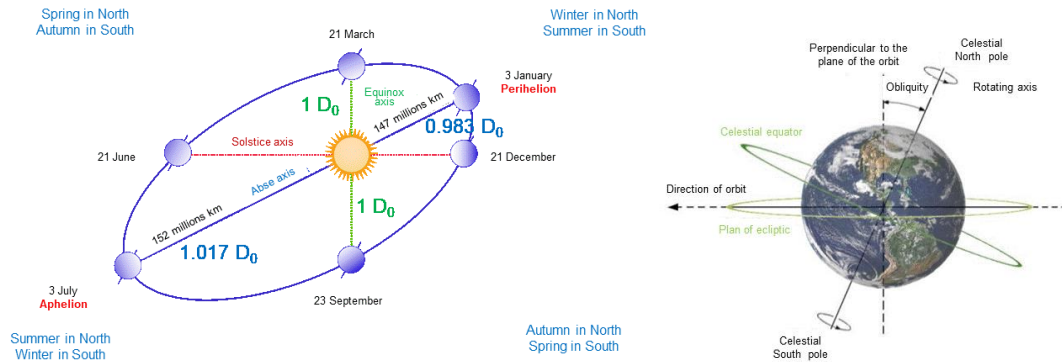
Figure 2-3: Representation of the Earth's orbit around the Sun
