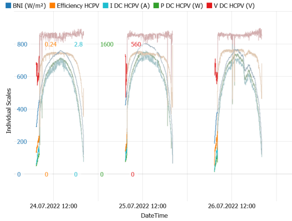
Figure C-35: Time series plot related to the selected points in Fig. C-34
