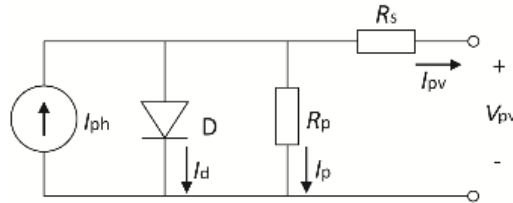
Figure 3-18: Single-diode model of a PV cell
