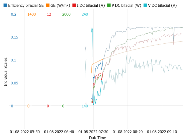
Figure C-25: Zoom-in of Fig. C-24, focusing on the sunrise.
