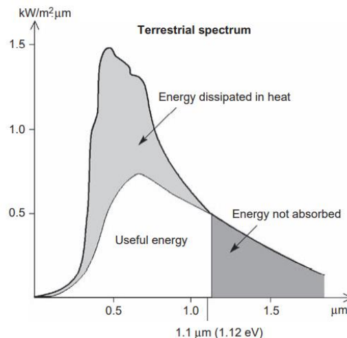
Figure 2-16: Use of the AM0 solar spectrum by crystalline PV
