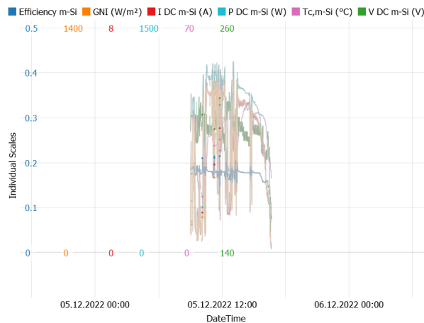
Figure C-13: Time series referring to the scatter plot in Fig. C-12
