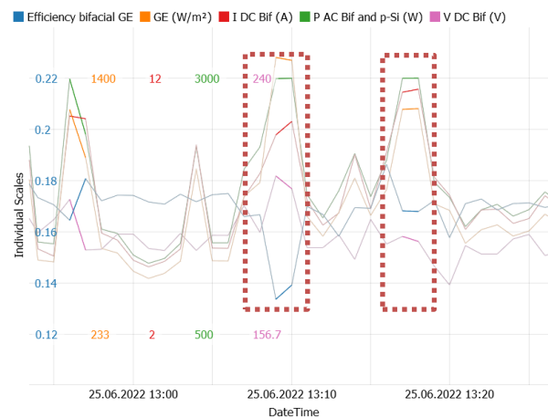
Figure C-27: Time series plot referring to Fig. C-26, showing inverter saturation.
