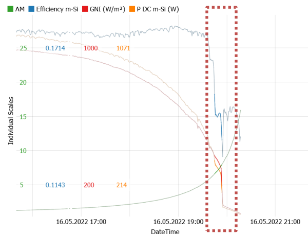
Figure C-18: Time series related to the scatter plot in Fig. C-17
