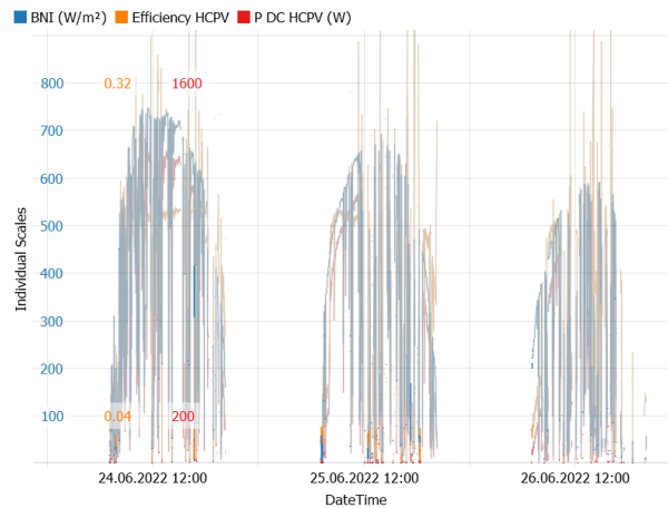
Figure C-31: Time series referring to the scatter plot in Fig. C-30
