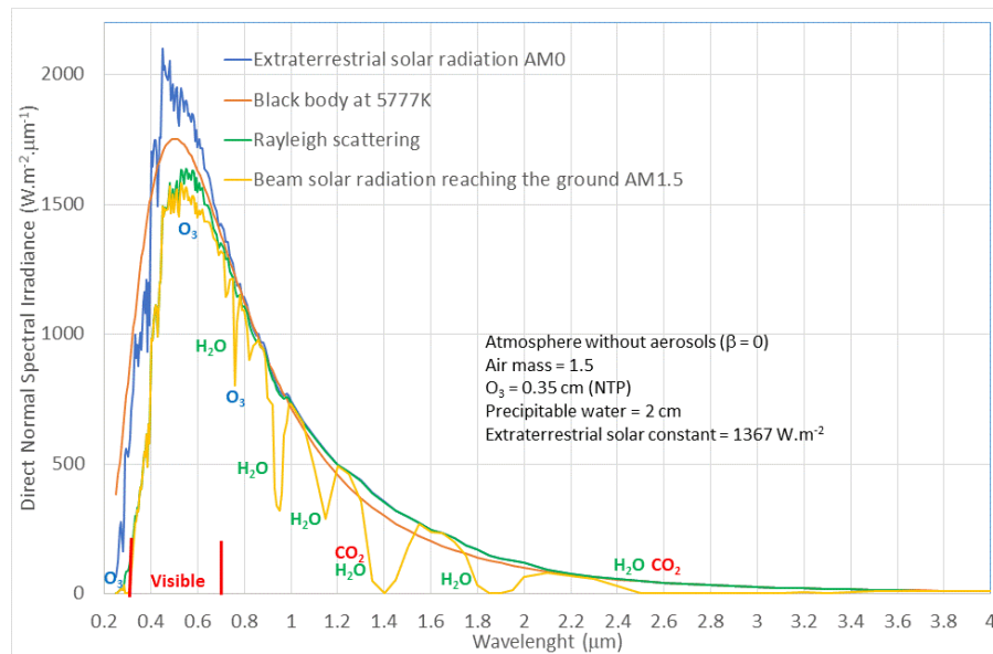
Figure 2-11: Spectral distribution of the solar radiation
