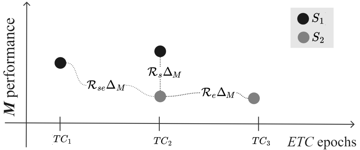
Figure 4.2: \mathcal{R}\Delta_M of systems S_1 and S_2 evaluated in TC_1 , TC_2 and TC_3 , three ETC epochs.
