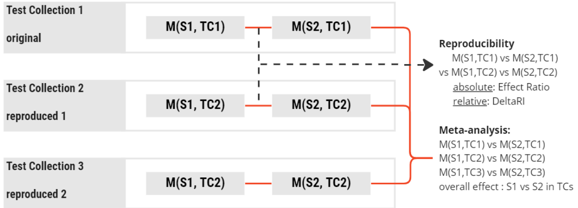
Figure 2.8: Comparison between Effect Ratio, DeltaRI and Meta-analysis.
