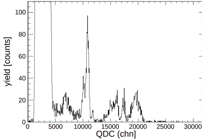
Figure 3.11: QDC spectrum from a strip of the BB10 detector from the PIXEL project.
