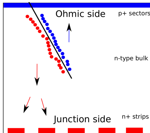
Figure 2.24: Simplified scheme of a polarized silicon particle detector [40].
