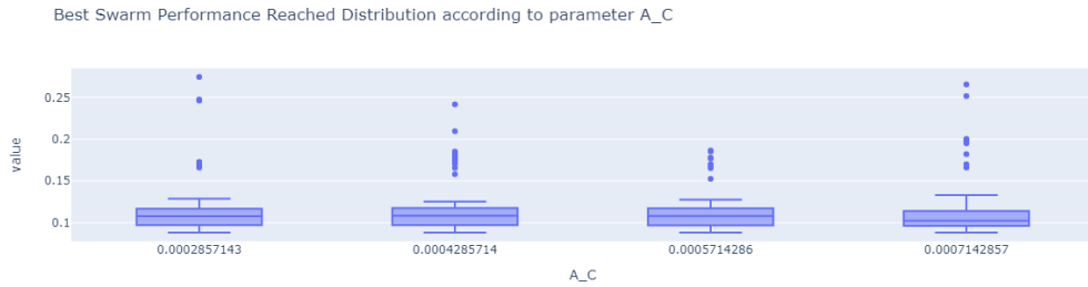
Figure 71: Distribution of the best performances reached according to a_c value
