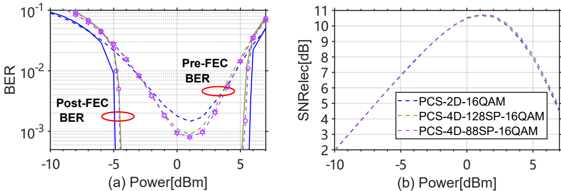
Figure 4.11: Performance over a multi-span link (same PCS schemes as in Fig. 4.9): (a) BER vs launched power/channel. (b) Electrical SNR vs launched power/channel.
