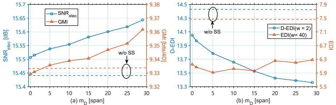
Figure 5.15: Performance analysis of D-SS 1 4 (a): GMI versus m_D at optimal power (4.5 dBm) where m_D is the maximum number of spans used by the dispersion applicer during sequence selection. Gains are maintained even when we reduce the complexity by computing D-EDI over fewer spans. (b): D-EDI and EDI versus m_D . We add the values for ESS without SS by horizontal dashed lines. Same system configuration as in Fig.5.13. D-EDI demonstrates a negative correlation with SNR elec .
