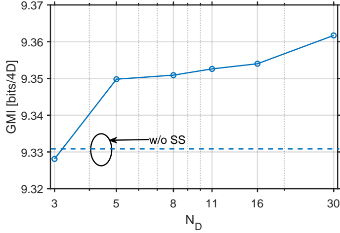
Figure 5.16: GMI versus N_D for D-SS 1 4 , where N_D is the number of EDI calculations required to compute D-EDI, each N_D value represents the following span indices: N_D = 3 \rightarrow [0, 1, 29] ; 5 \rightarrow [0, 1, 9 : 10 : 29] ; 8 \rightarrow [0, 1, 4 : 5 : 29] ; 11 \rightarrow [0, 1, 2 : 3 : 29] ; 16 \rightarrow [0, 1 : 2 : 29] ; 30 \rightarrow [0 : 1 : 29] . We add the values for ESS without SS by horizontal dashed lines. Same system configuration as in Fig. 5.13. Gains are maintained even when we reduce the complexity by computing D-EDI over several spans.
