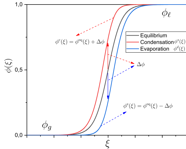
Figure 6.1: Profiles of condensed and evaporated liquid-gas capillary interfaces \phi^c(\xi) \phi^e(\xi) , respectively for \Delta\xi = 1 .
