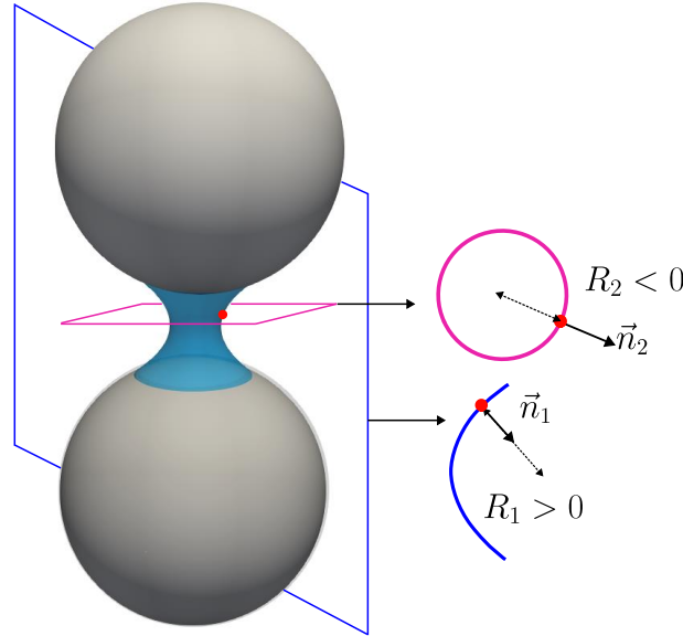
Figure 1.12: Illustration of the signs of curvatures within a typical capillary bridge between two spherical particles.
