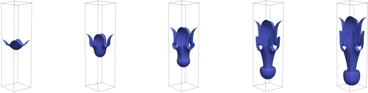
Figure 4.2: Evolution of the interface \phi = 0.5 as a function of the dimensionless time t^* = 1; 2; 3; 4; 4.5 , respectively.
