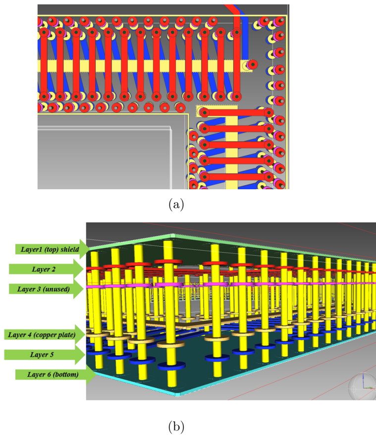
Figure 5.18 – PCB rogowski coil (a) top view (b) cross-section view.
