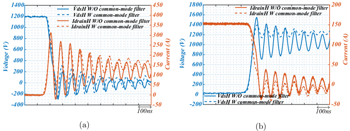
Figure 4.35 – V_{ds} and I_d comparison between the gate driver without (W/O) integrated CM choke and the gate driver with (W) integrated CM choke, -150 A (a) V_{dsH} with I_{dsH} turn-on transition (b) V_{dsH} Vs. I_{dsH} turn-off transition.
