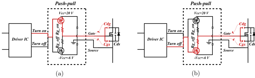
Figure 4.8 – Output stage of gate driver with push-pull (totem-pull) (a) Turn-on transition in push-pull (b) Turn-off transition in push-pull
