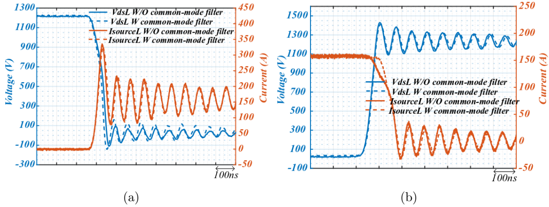
Figure 4.34 – V_{ds} and I_s comparison between the gate driver without (W/O) integrated CM choke and the gate driver with (W) integrated CM choke, Double pulse test in 1200 V, +150 A (a) V_{dsL} Vs. I_{dsL} turn-on transition (b) V_{dsL} Vs. I_{dsL} turn-off transition.
