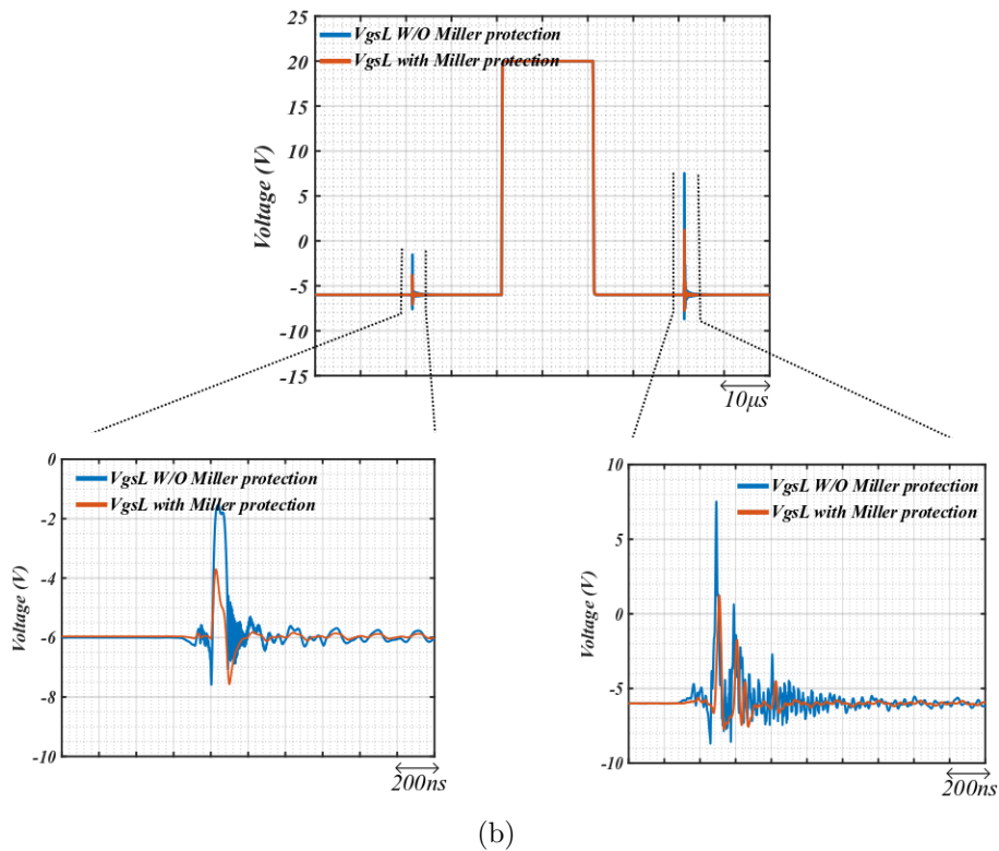
Figure 4.12 – Simulation results of comparison between the gate driver with (W) with Miller clamp integrated circuit and without (W/O) Miller clamp integrated circuit, double pulse test, 500 V (a) V_{gsH} (synchronous switch, soft switching condition) in +150 A (b) V_{gsL} (synchronous switch, soft switching condition) in -150 A.
