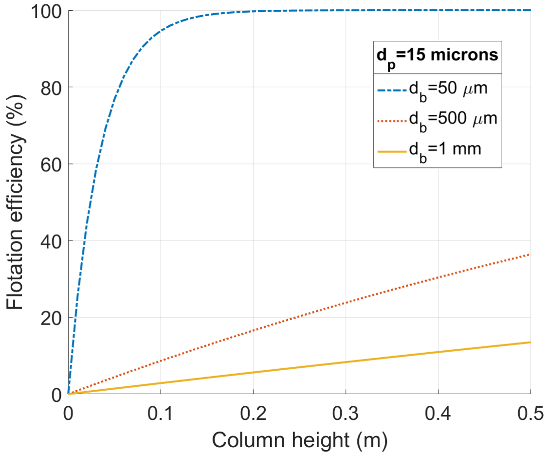
Figure 5.9: Effect of the bubble size on flotation efficiency for a 15\mu\text{m} droplet in a water at 1 \text{ Cp} in co-current configuration
