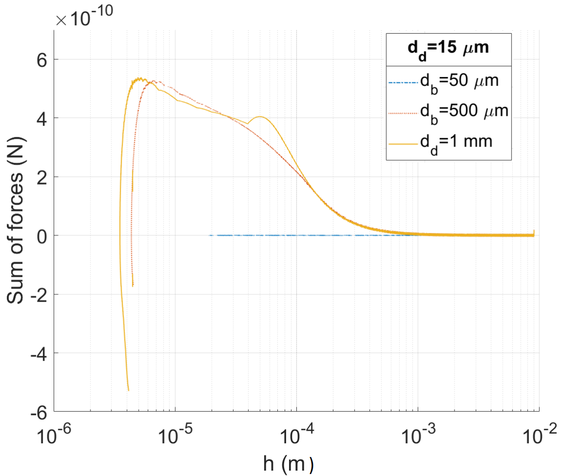
Figure 4.6: Evolution of the sum of the forces acting on a droplet of d_d = 15\mu m in a water at 1 for 3 bubble diameter
