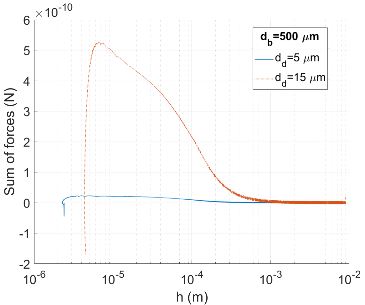
Figure 4.7: Evolution of the sum of the forces acting on a droplet for a bubble of d_b = 500\mu\text{m} in a water at 1 Cp for 2 droplet diameters
