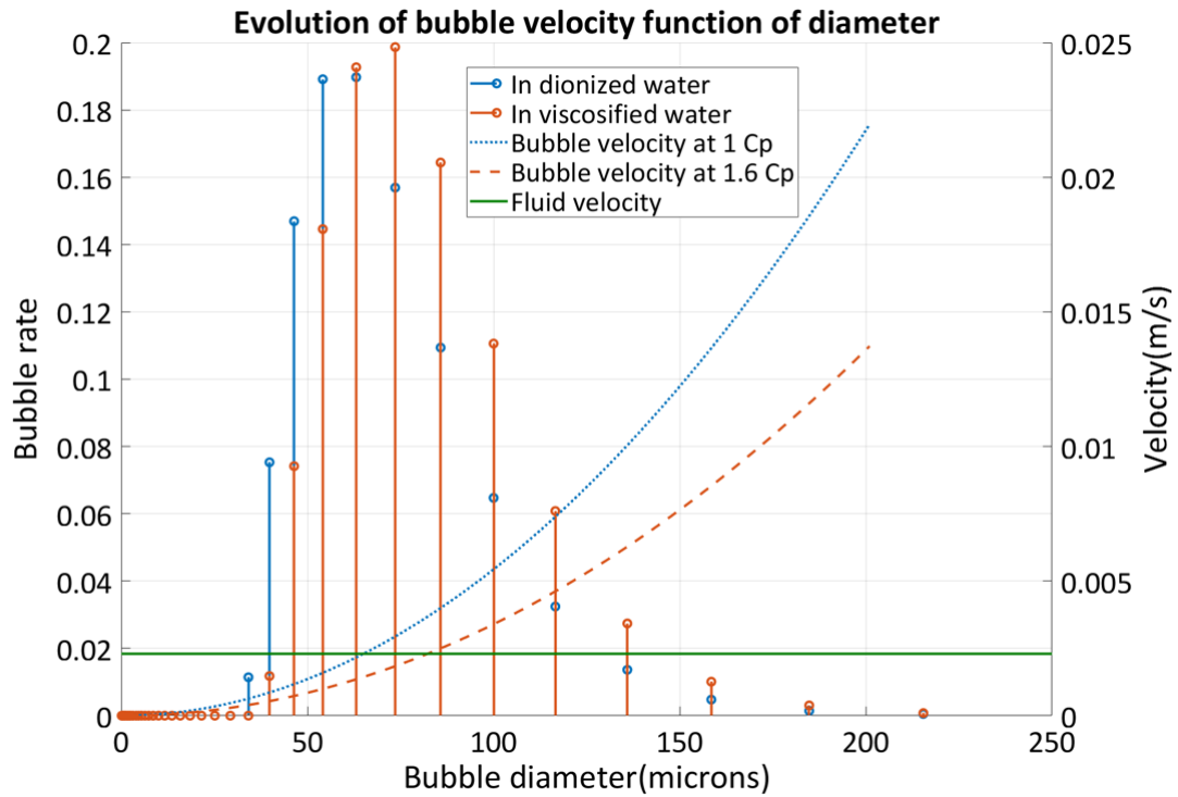
Figure 5.12: Evolution of bubble rising velocity function of their diameter in per-mutated and viscosified water with the bubble distribution in each kind of water
