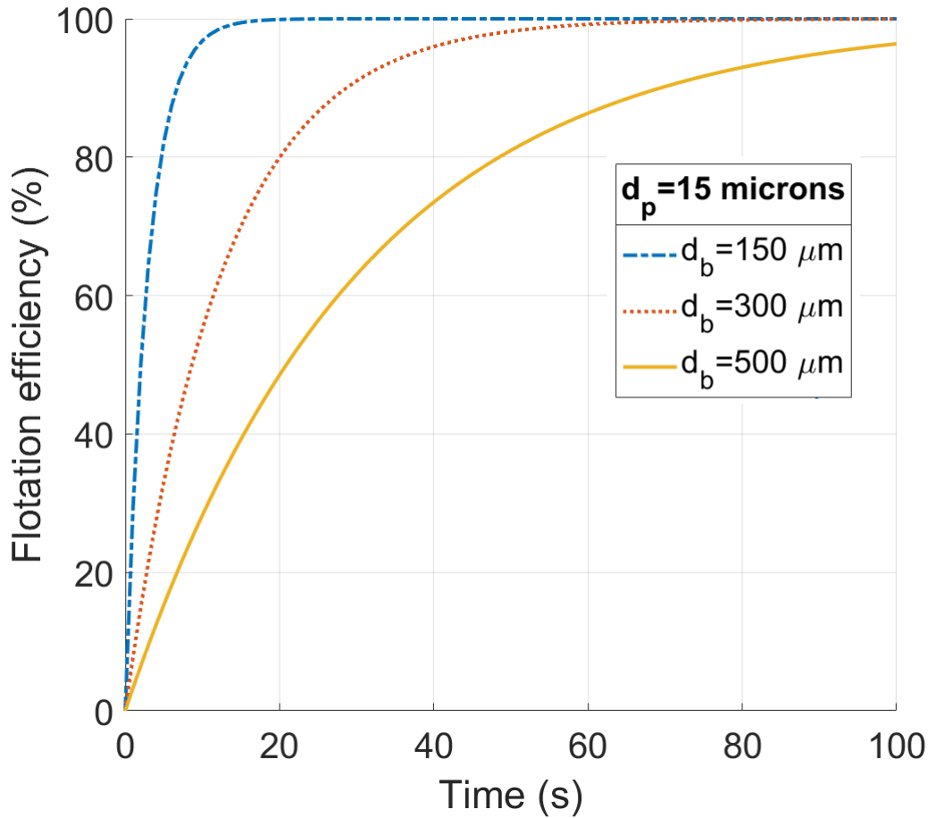
Figure 5.5: Effect of the bubble size on flotation efficiency for a 15\mu\text{m} droplet and water viscosity at 1 Cp in batch configuration
