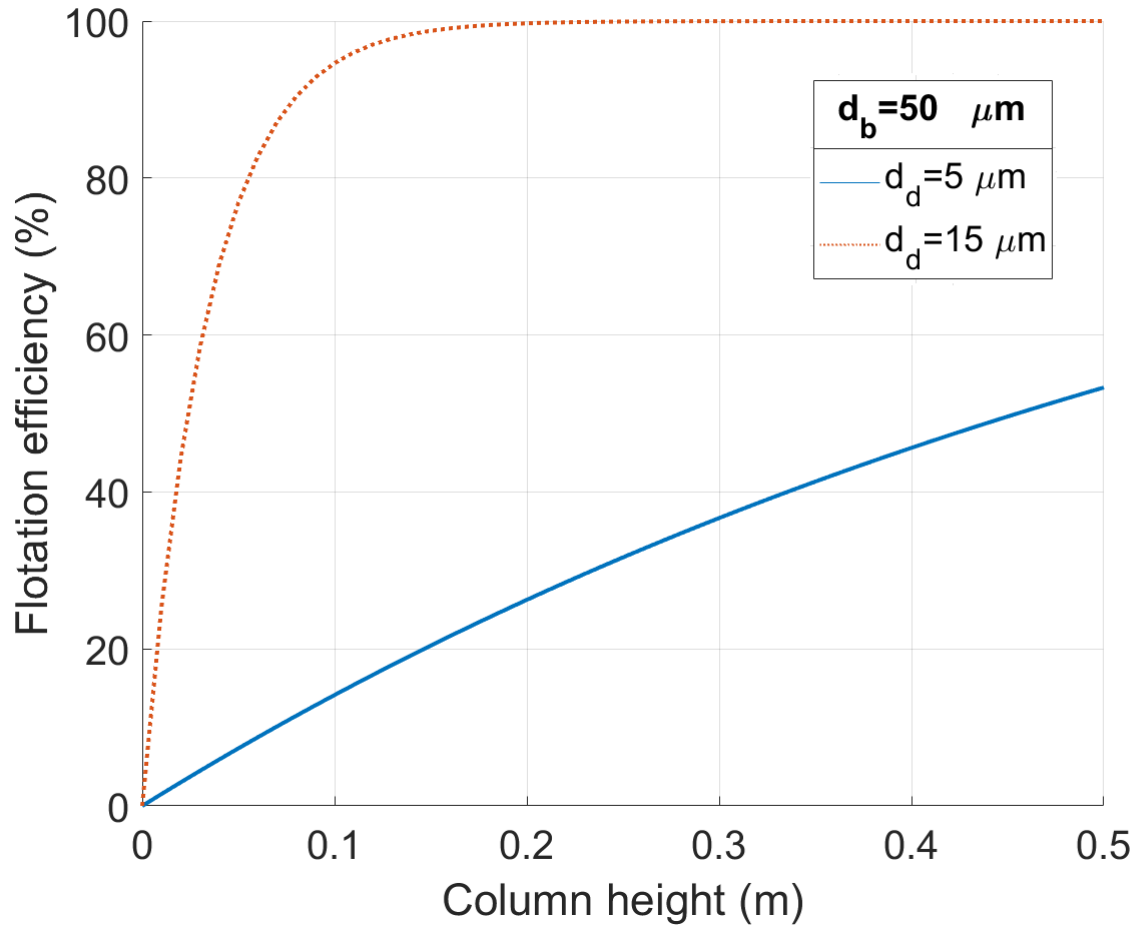
Figure 5.10: Effect of the droplet size on flotation efficiency for a 50\mu\text{m} bubble in a water at 1 Cp in co-current configuration
