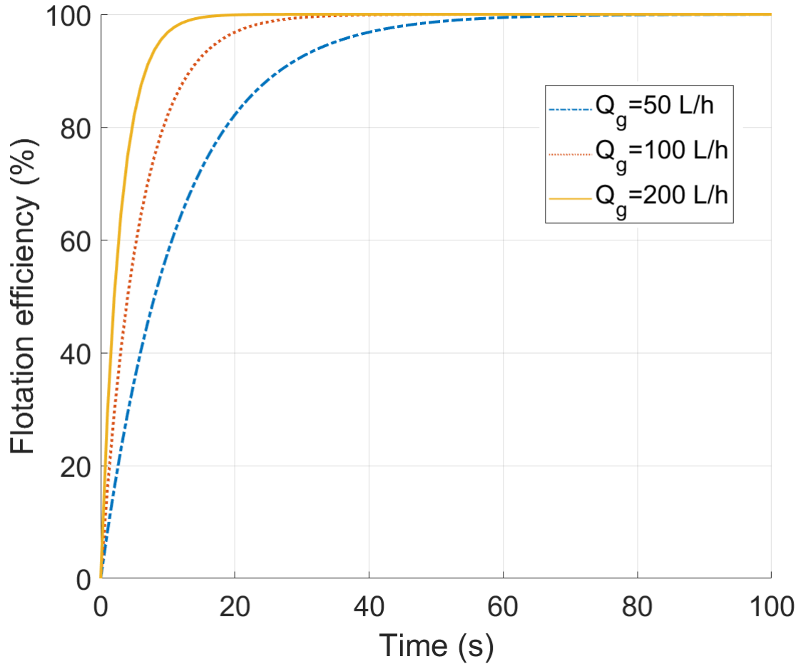
Figure 5.7: Effect of the gas flow rate on flotation efficiency for a 15\mu\text{m} droplet & a 150\mu\text{m} bubble in batch configuration ( Q_g = 50\text{L/h} \Rightarrow \alpha = 0.1027 ; Q_g = 100\text{L/h} \Rightarrow \alpha = 0.2054 ; Q_g = 200\text{L/h} \Rightarrow \alpha = 0.4109 )
