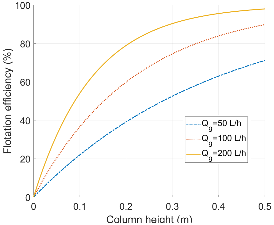
Figure 5.11: Effect of the gas hold up on flotation efficiency for a 15\mu\text{m} droplet & a 100\mu\text{m} bubble in co-current configuration ( Q_g = 50\text{L/h} \Rightarrow \alpha = 0.038 ; Q_g = 100\text{L/h} \Rightarrow \alpha = 0.0748 ; Q_g = 200\text{L/h} \Rightarrow \alpha = 0.1391 )
