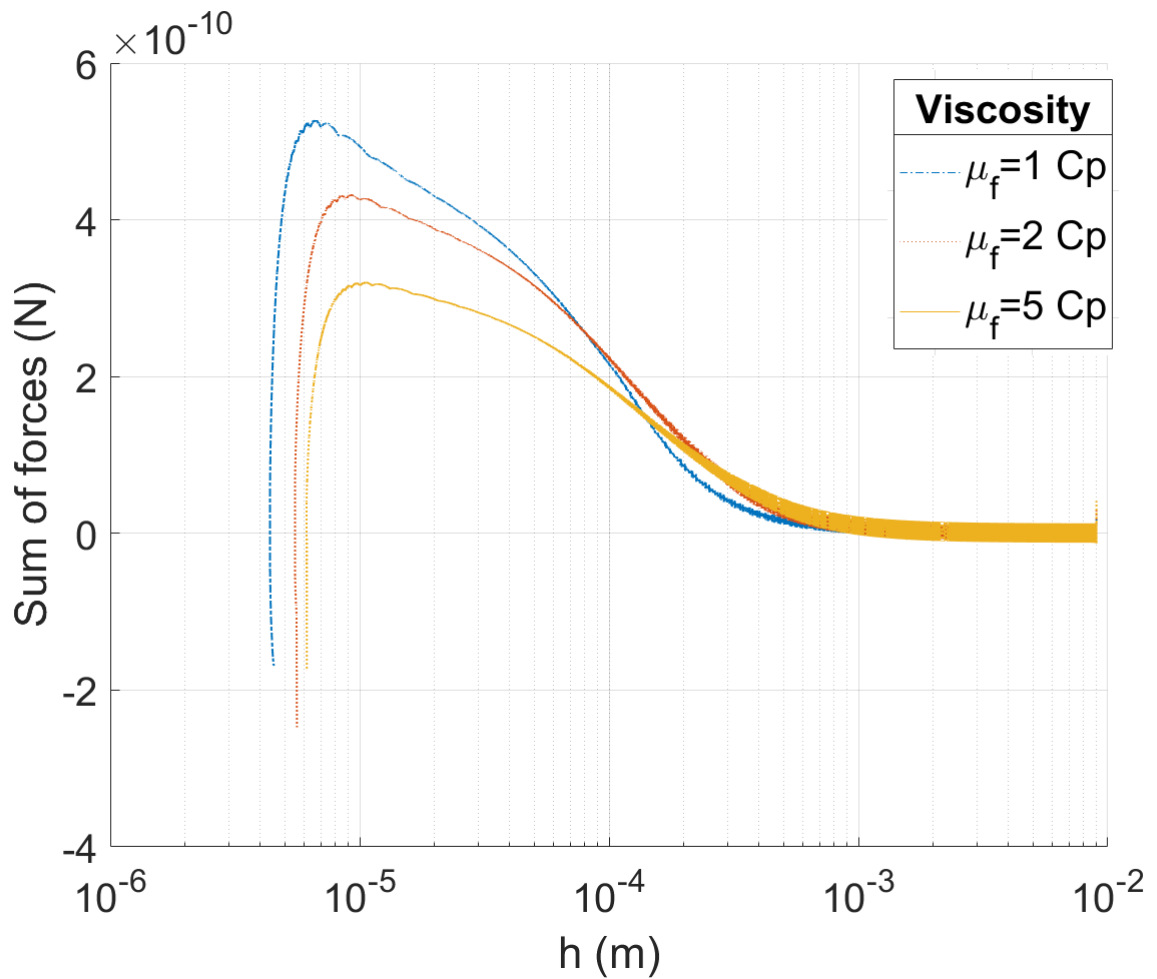
Figure 4.8: Evolution of the sum of the forces acting on a droplet for d_b = 500\mu m & d_d = 15\mu m in a water at 1, 2 & 5 Cp
