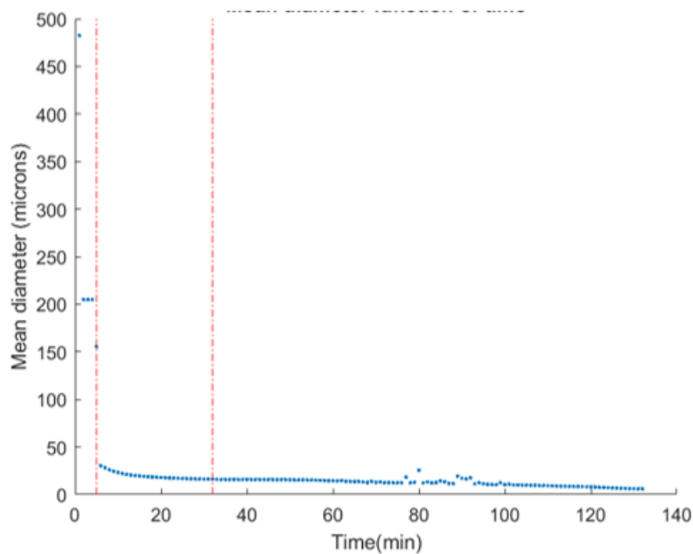
Figure 2.25: Evolution of the droplets mean diameter function of the emulsion resting time
