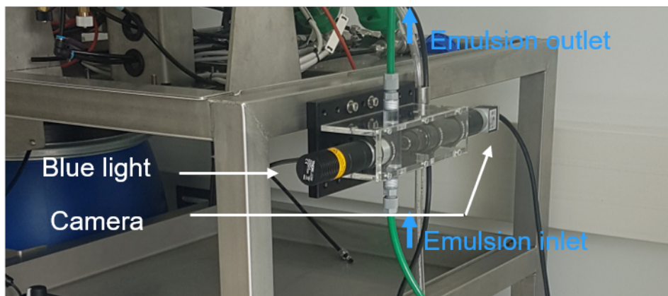
Figure 2.16: Dropsizer device
