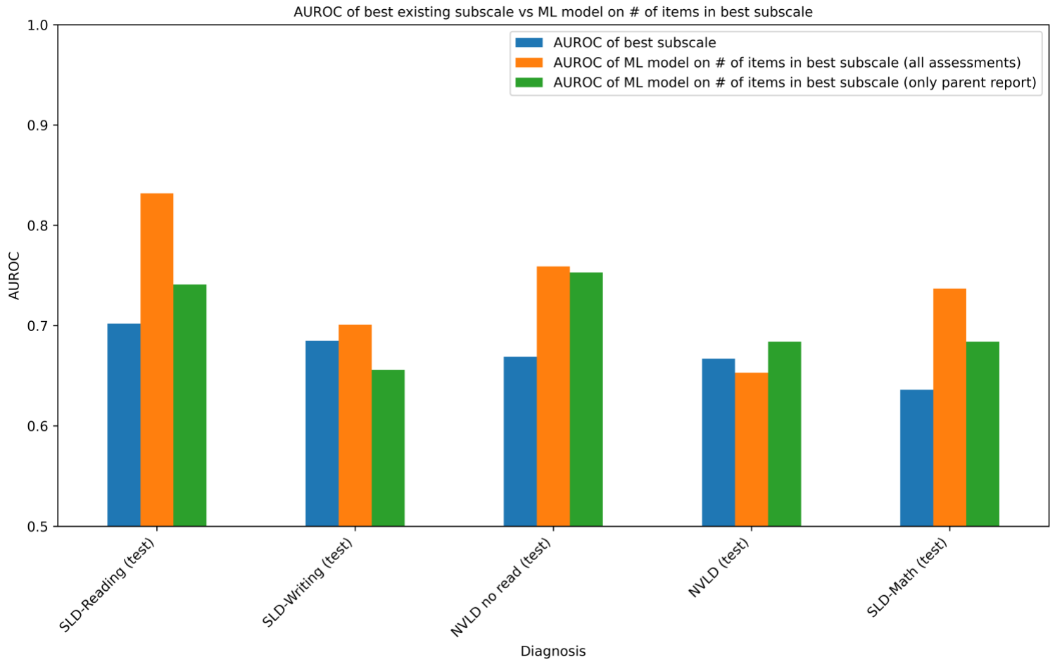
Figure 35. Comparison of the predictive performance of machine learning models using all assessments and only parent-report assessments, and the performance of the best subscale (learning diagnoses).
