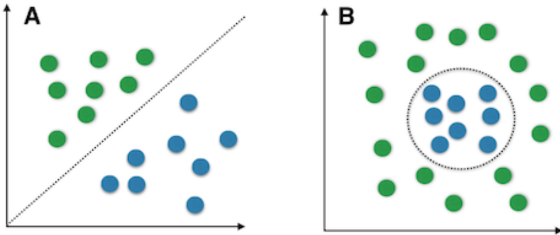
Figure 4: Two simplified examples of binary classification problems with two features, presented as scatter plots with each training example plotted on a 2-dimensional plane, where each dimension corresponds to one feature (reproduced from Activation Functions and Optimizers for Deep Learning Models | Exxact Blog (2019)).
