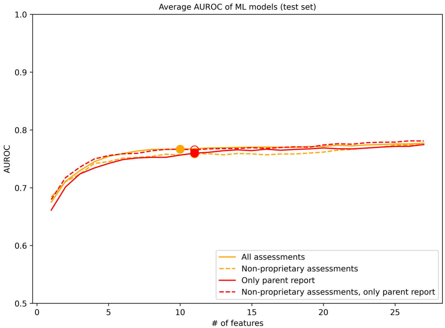
Figure 38. Average performance saturation for the models using different input assessments subsets. The highlighted marker represents the recommended number of features.
