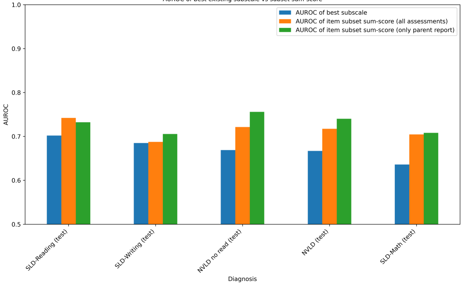
AUROC of best existing subscale vs subset sum-score
