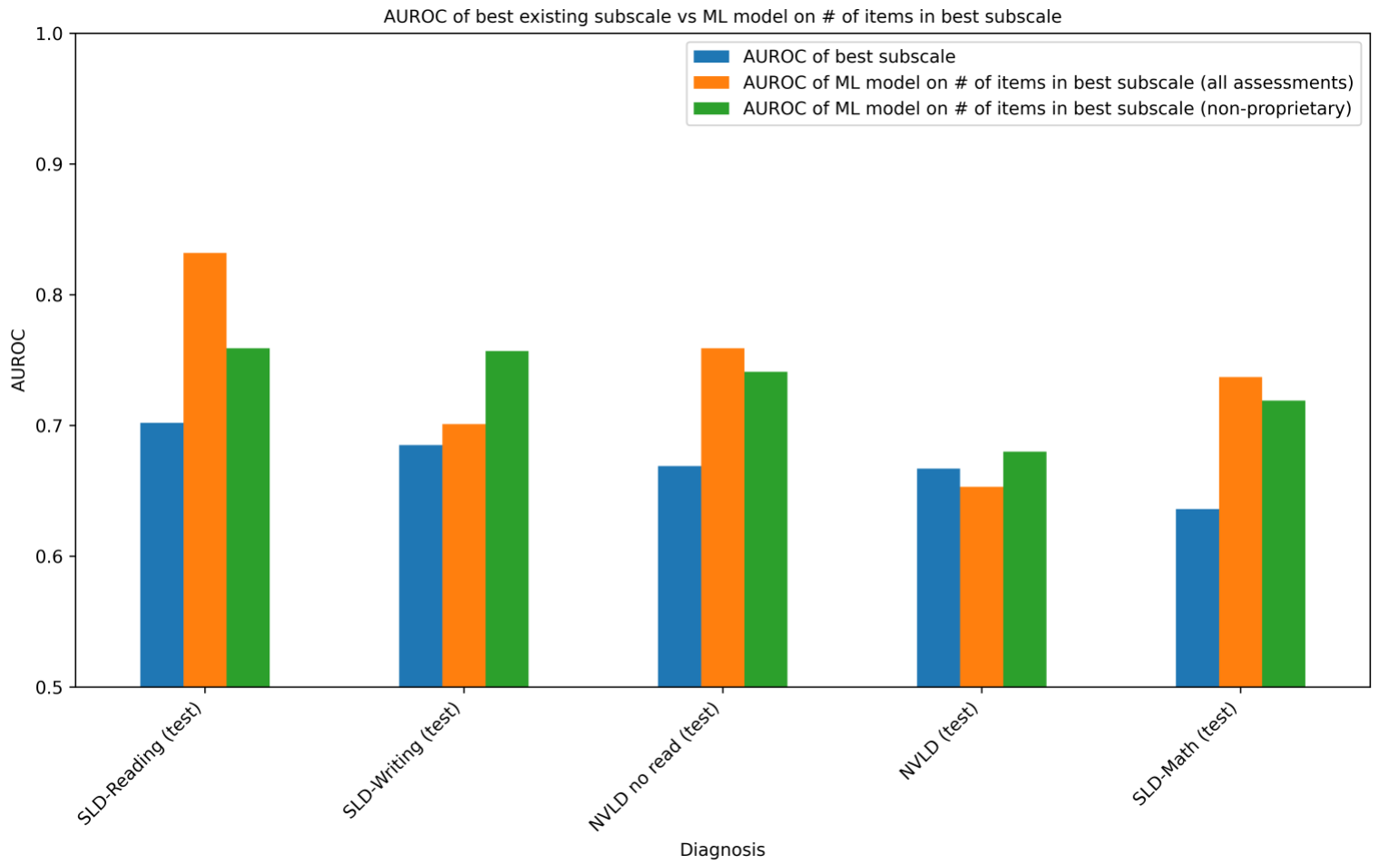
Figure 31. Comparison of the predictive performance of machine learning models using all assessments and only non-proprietary assessments, and the performance of the best subscale (learning diagnoses).
