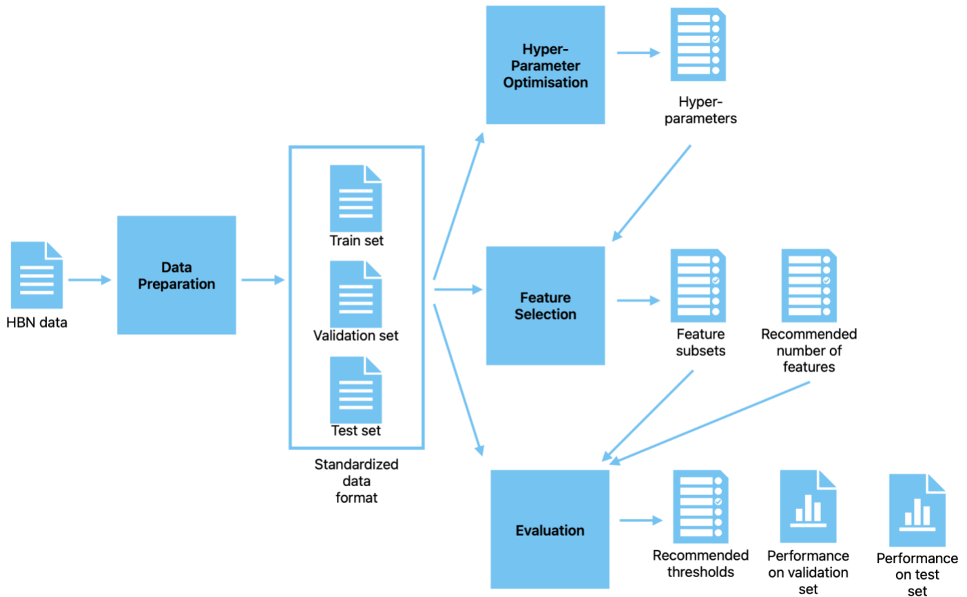
Figure 8: Overview of the framework.
