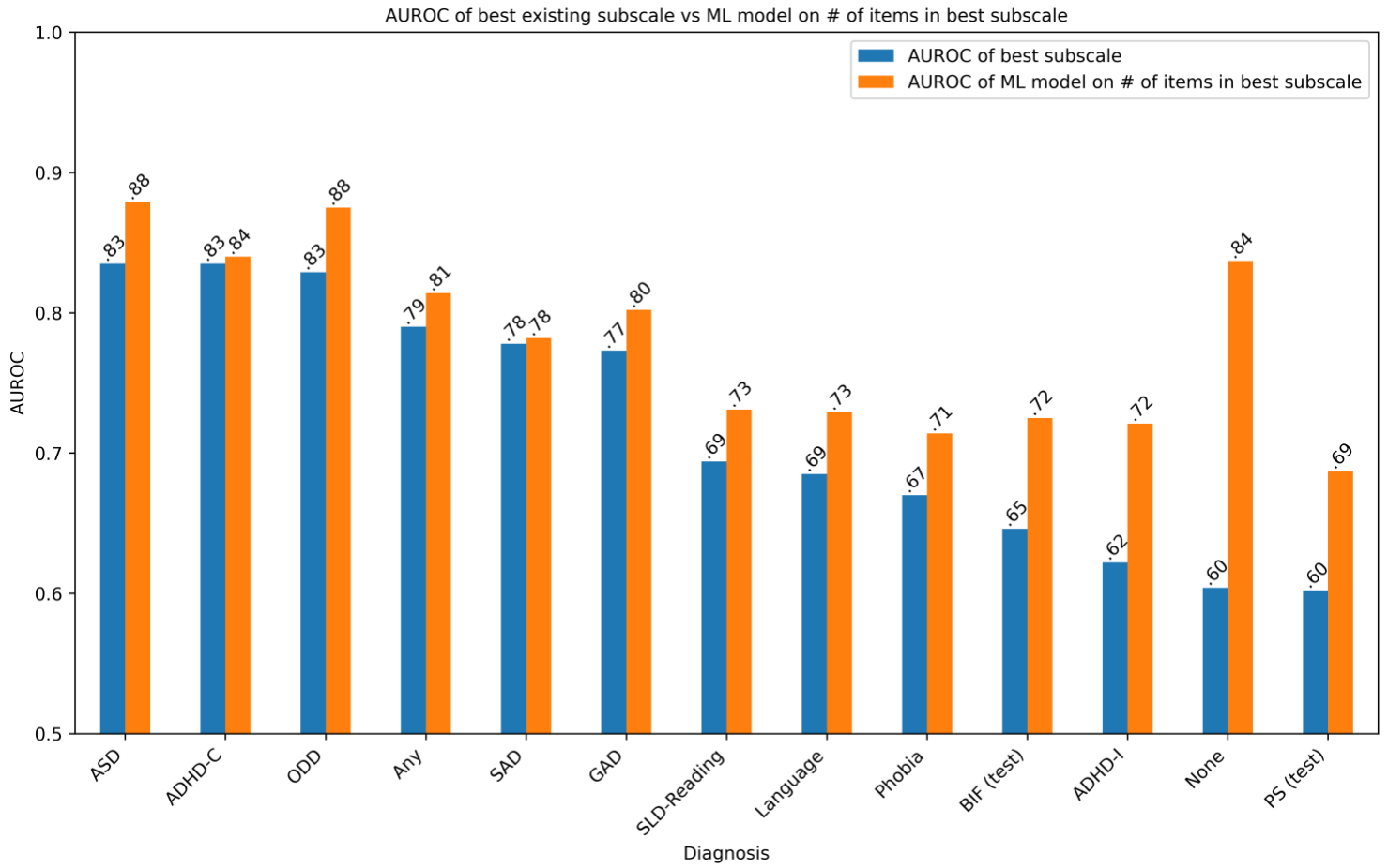
Figure 10: Comparison of the classification performance of machine learning models to the performance of the best subscale (non-learning diagnoses).
