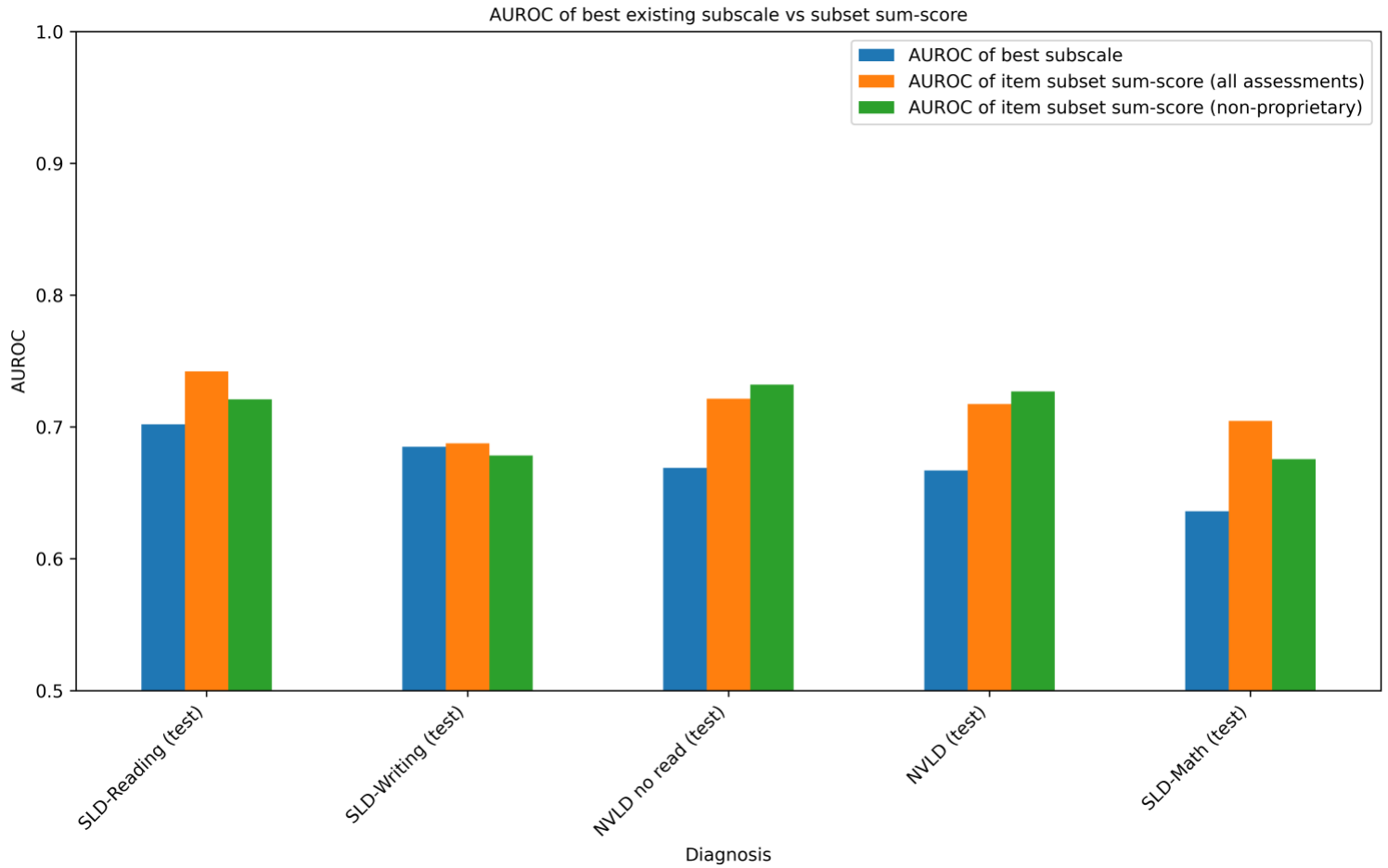
Figure 33. Comparison of the predictive performance of the sum-scores of identified item subsets using all assessments and only non-proprietary assessments, and the performance of the best subscale (learning diagnoses).
