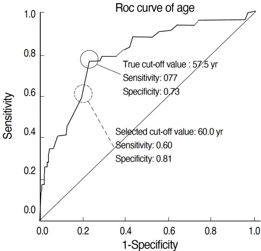
Figure 3: Use of ROC curve to determine the cut-off value of age as a predictor prioritizing higher specificity value ("Selected cut-off value") despite another cutoff resulting in a higher overall performance ("True cut-off value") (reproduced from Kwon et al. (2009))
