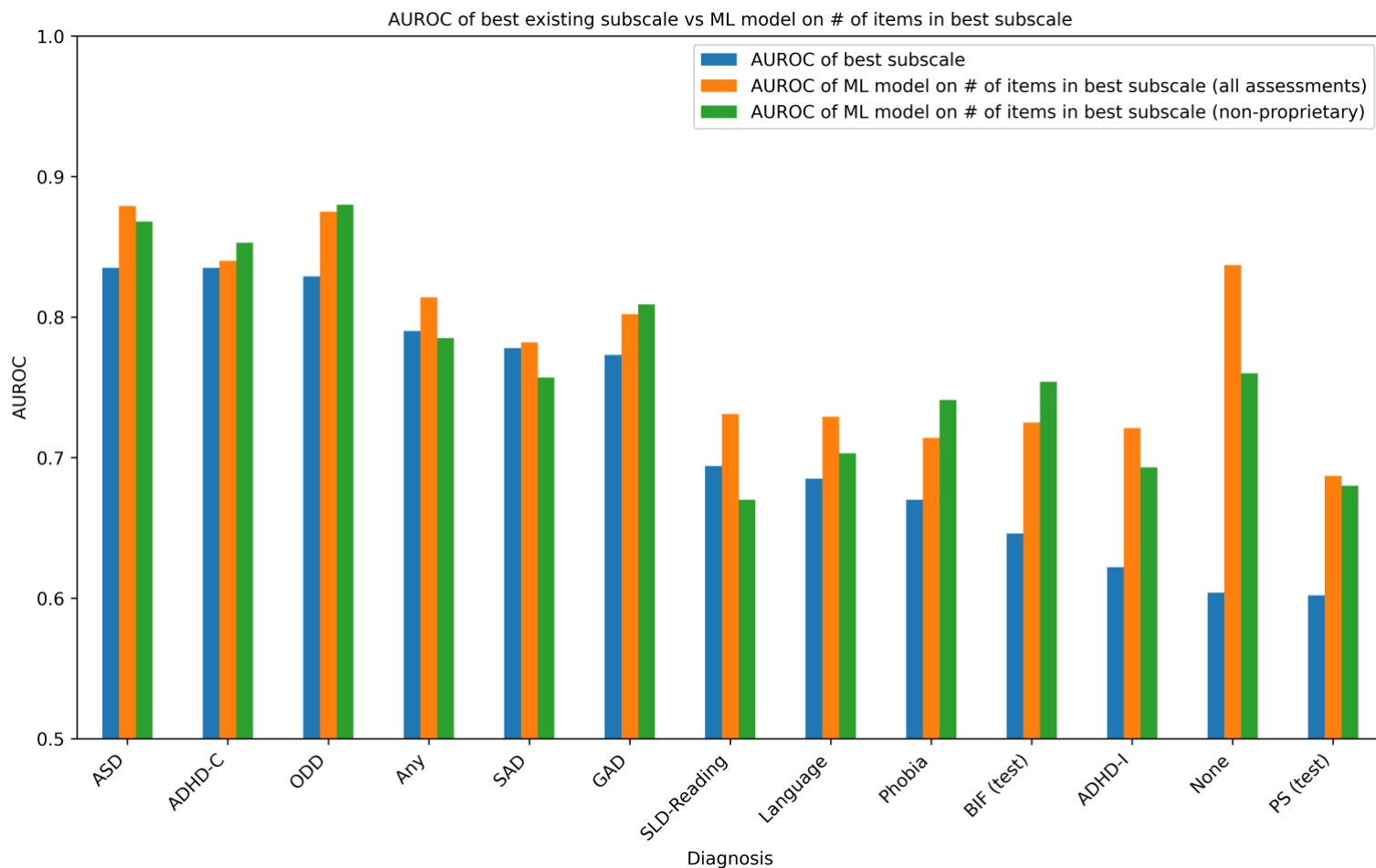
Figure 30. Comparison of the predictive performance of machine learning models using all assessments and only non-proprietary assessments, and the performance of the best subscale (non-learning diagnoses).
