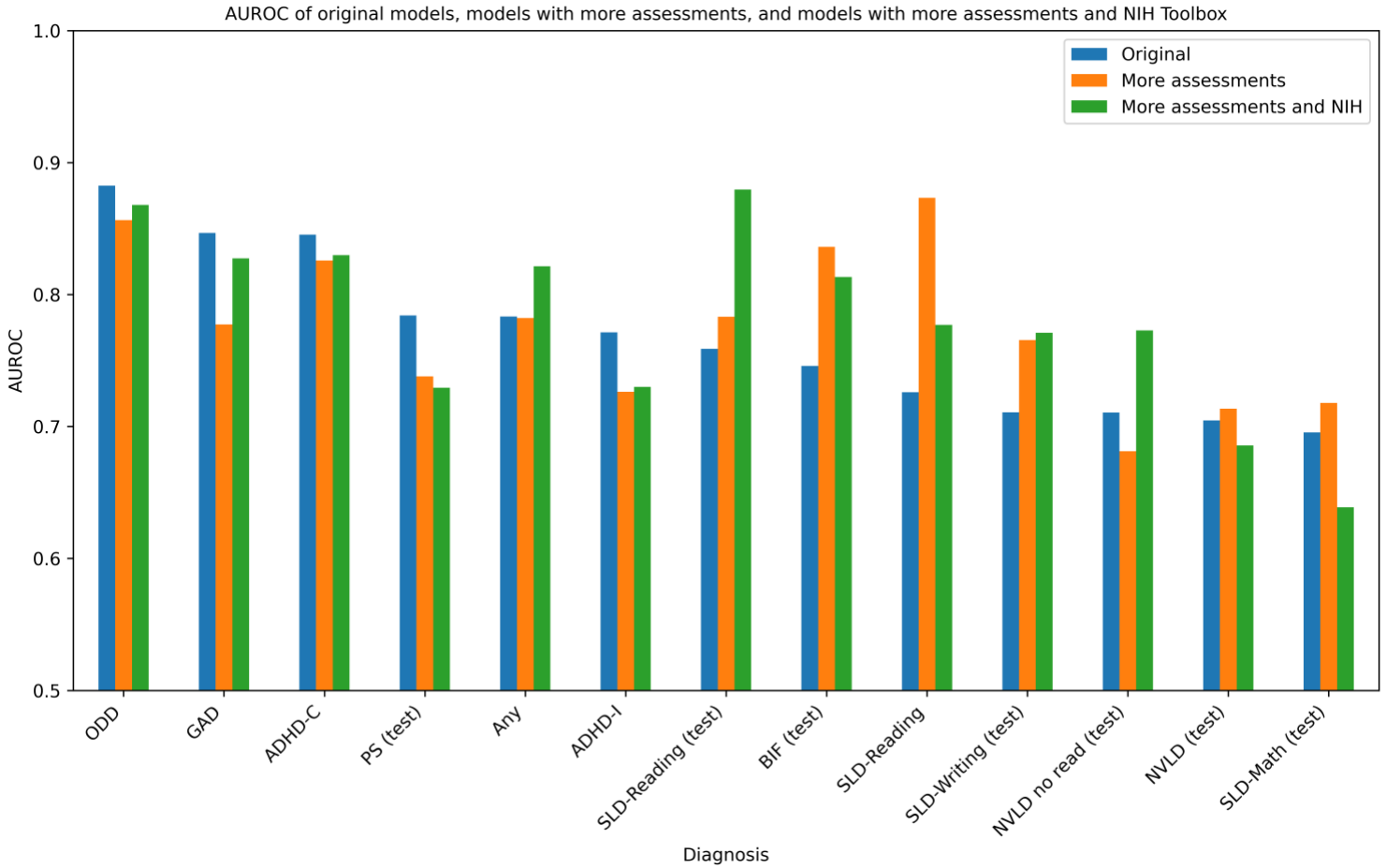
Figure 15: Comparison between the performance of the original models, models using additional self- and parent-report questionnaires, and models using both additional questionnaires and the NIH scores.
