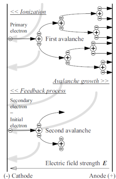
Figure 1.4. Schema of the Townsend mechanism [22].
