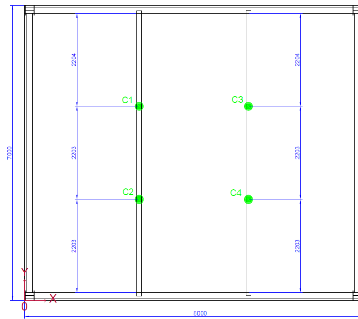
(c) Location of measuring points (dimensions in mm)
