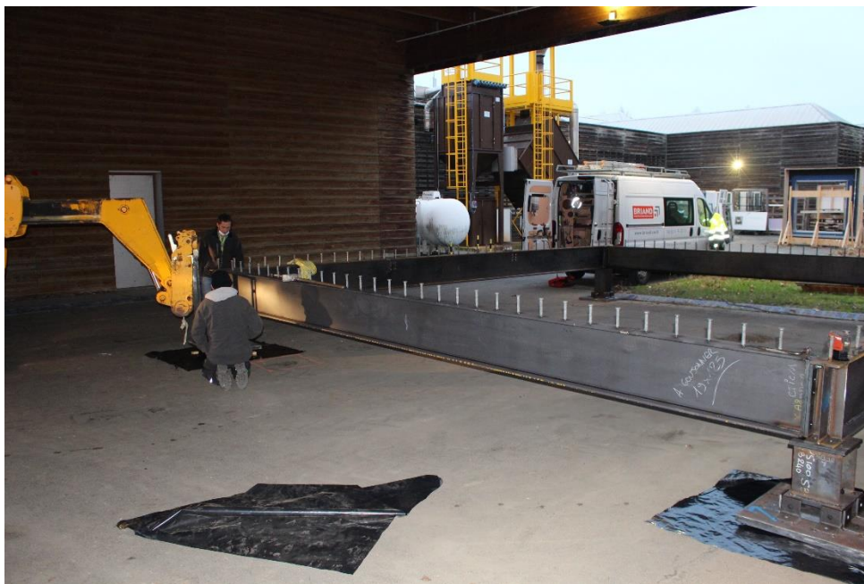
Figure A.6: Shear connectors welded to beams
