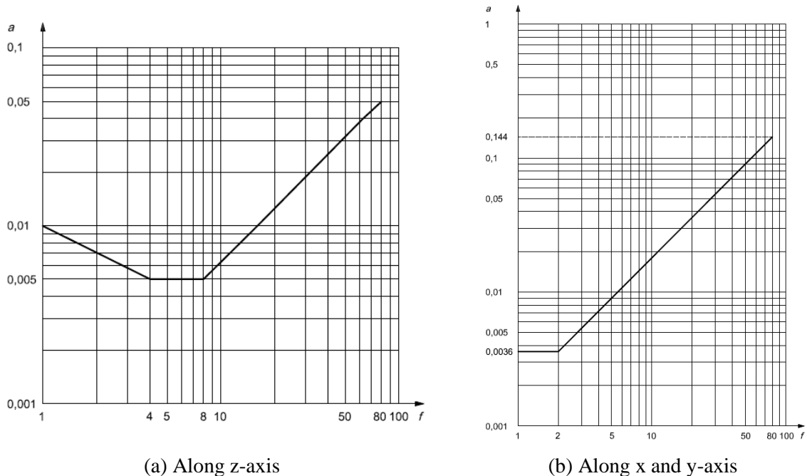
Figure 2.6: Basic acceptability curves from ISO 10137 [45]
