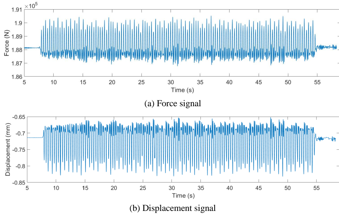
Figure 4.9: Example of raw test records for “skipping 2” activity
