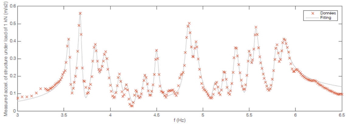
Figure 5.7: Multi-mode FRF for Setup 1 and frequency band between 3 and 6.5Hz [24]
