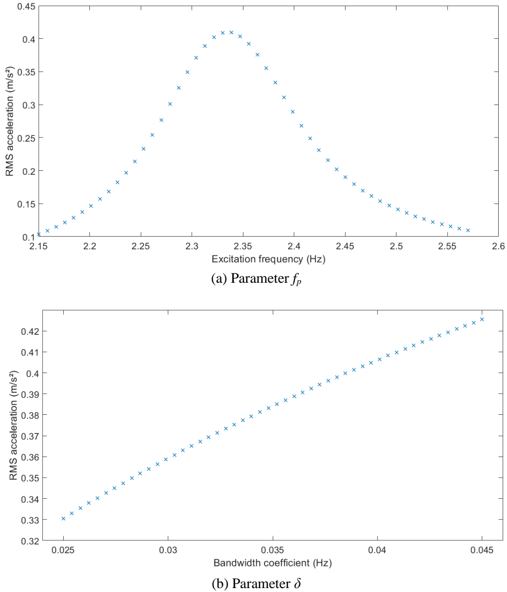
Figure 6.1: Variation of RMS acceleration against PSD load model parameters
