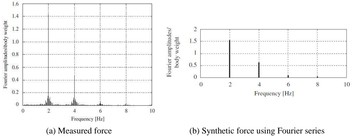
Figure 4.3: Illustration of jumping loads in the frequency domain [71]
