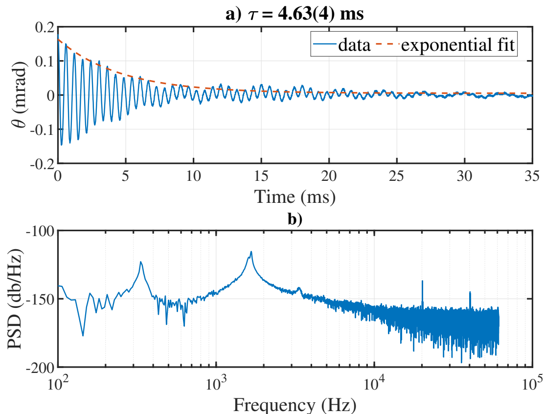
Figure 3.17: Angular evolution after a short driving time at constant speed and an abrupt stop when the motor reached the target angle. a) Damped oscillation of the angle, where we subtracted the mean value for clarity. The angular position has been directly reconstructing using the calibrated 4-quadrant b) Associated PSD.
