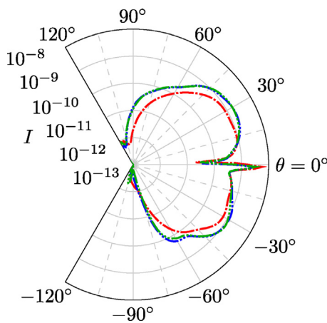
Fig. 14. Variations of acoustic intensity at r = 200\delta_\omega from the vortex pairings as a function of the polar angle \theta for — \Delta y_0 = 0.4\delta_\omega , — \Delta y_0 = 0.2\delta_\omega and — \Delta y_0 = 0.1\delta_\omega .
