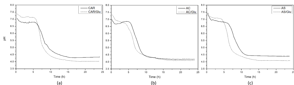
Figure X-1. Acidification kinetics of S. thermophilus (ST) in protein extracts obtained from different pea cultivars CAR (a), AC (b), AS (c) without glucose (solid line) and in presence of glucose 1% (short dot line).
