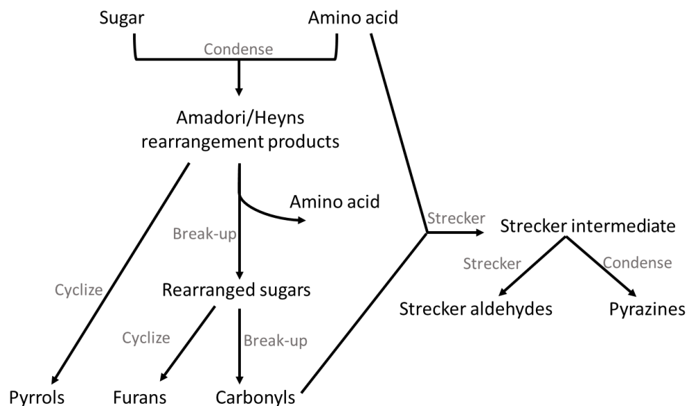
Figure I-7. Schematic of flavor formation by Maillard reaction (modified from Jousse et al. (2002))
