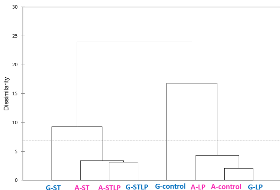
Figure VI-5. Agglomerative hierarchical clustering (AHC) of odour active compounds (OACs) in pea protein albumin (A) and globulin (G) obtained by control or with fermentation by S. thermophilus (ST) and Lb. plantarum (LP) or their co-culture (STLP). The volatile compounds with DF (detection frequency) of 45% and higher were considered.
