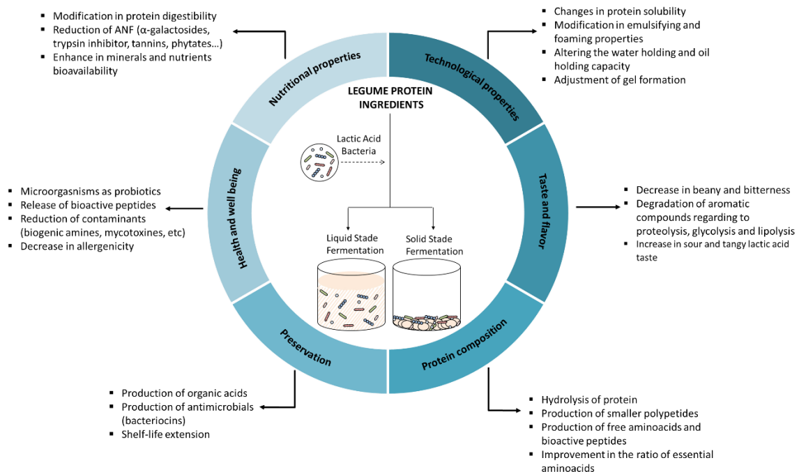
Figure I-10. Schematic depicting the effects of lactic acid fermentation on legume protein (adapted from Emkani et al. (2022)).
