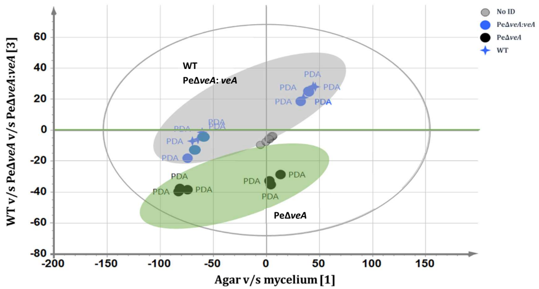
Figure S1. Principal Component Analysis (PCA) of the data obtained from the mass spectra. The strain effect. The strains showed a significant effect when comparing the null mutant PeΔveA strain versus WT or the complemented strain. The strains grew in PDA medium.
