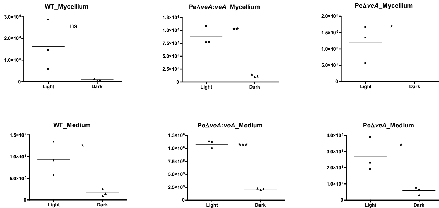
Figure S3b. Effect light. The graphs show the comparison of the relative abundance of clavicipitic acid produced under light or dark conditions by the WT strain and the null mutant strain PeΔveA in MEA for 5 days at 25 °C.
