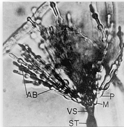
Figure 6. Morphological appearance of the null mutant \Delta abaA strain. The null mutant \Delta abaA strain produces normal conidiophore stalks (ST) and vesicles (VS), but metulae (M) and phialides (P) are abnormal and form abacus (AB) structures instead of conidia (C) (Adams et al. 1998).
