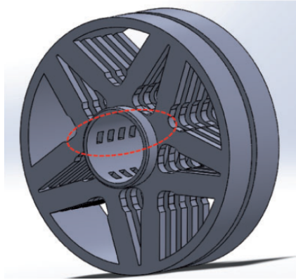
Figure 1.9: Geometrical lightweight gear: Spokes configuration
