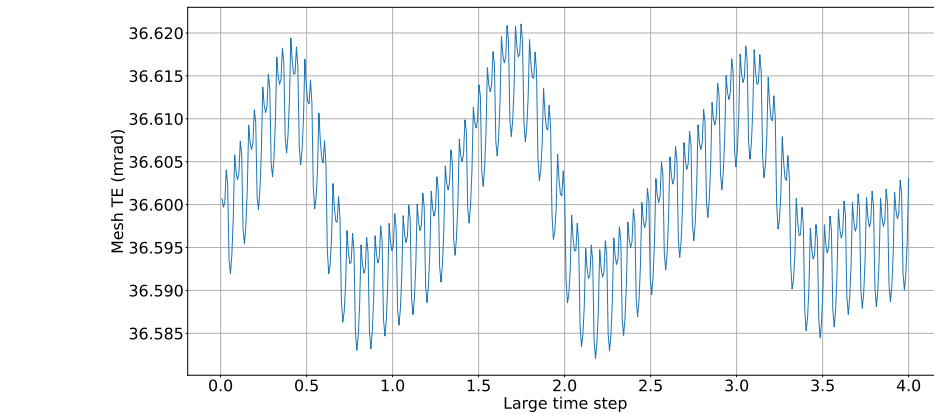
(a) Gear 1
