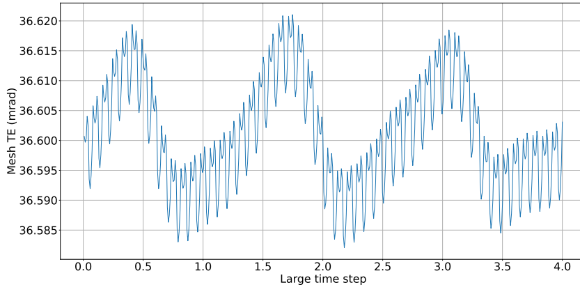
(a) Gear 1
