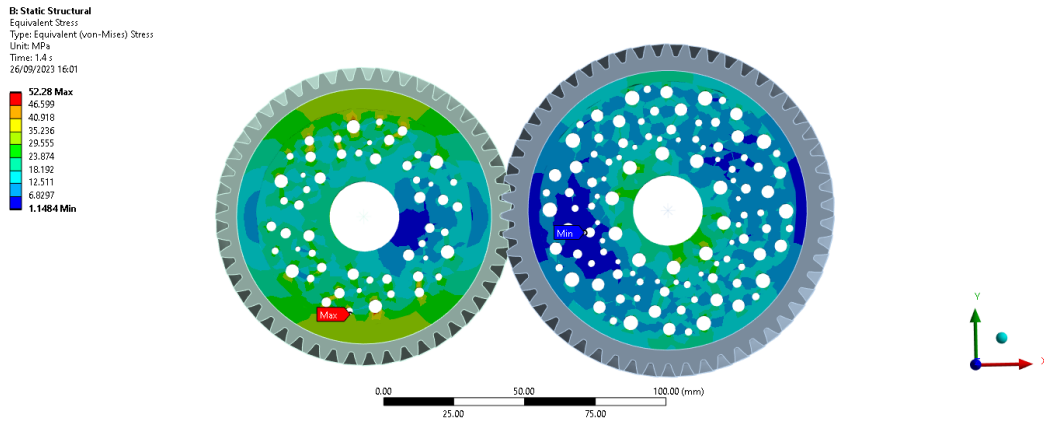
Figure 5.10: Visualization of the Von Mises stress distributions.
