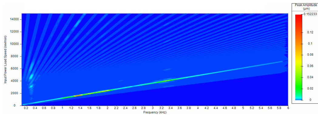
(a) Gear 1
