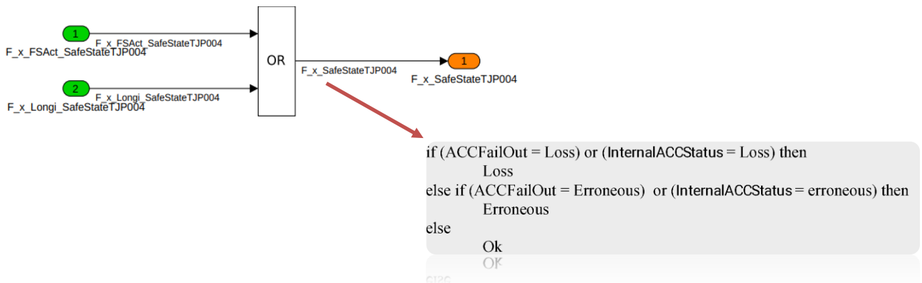
Figure 31. Transition from Simulink logics to AltaRica assertions
