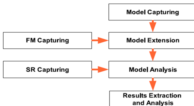
Figure 9. 4 xSAP Methodology [62]
