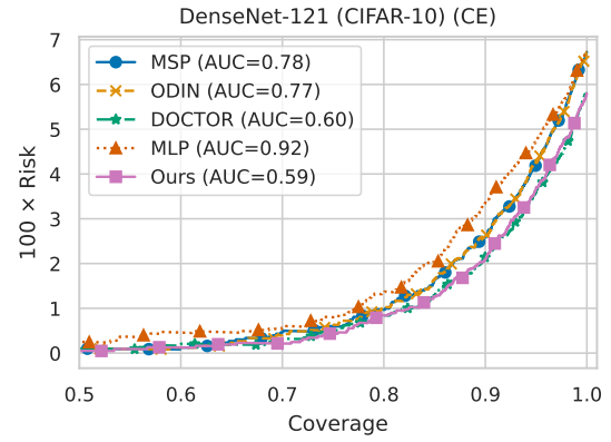
(b) DenseNet-121 RC curve.
