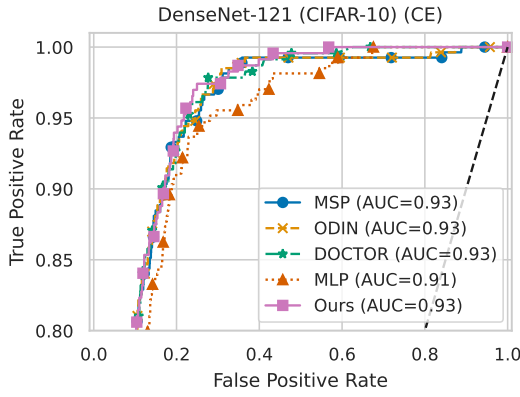
(a) DenseNet-121 ROC curve.
