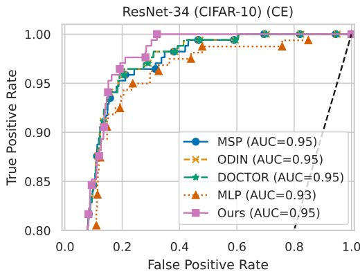
(c) ResNet-34 ROC curve.
