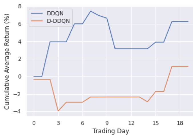
Fig. 2.15 Cumulative average returns from DRL approach with return reward function in training period
