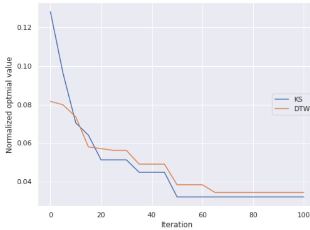
Fig. 3.2 Comparison of convergence rate
