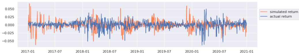
Fig. 3.7 Simulation of returns.
