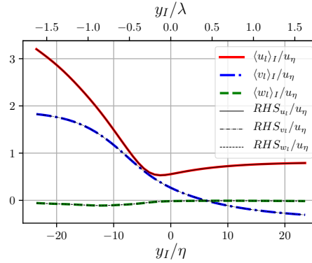
Fig. 4.6 TNTI-averaged profiles of \langle u_i \rangle_I , \langle v_i \rangle_I and \langle w_i \rangle_I and sum of the terms in the eqs. 4.15 for the IES of \omega_{th}^2/\omega_{ref}^2 = 10^{-3} at t/T_{ref} = 50 in PJ4-LV simulation.
