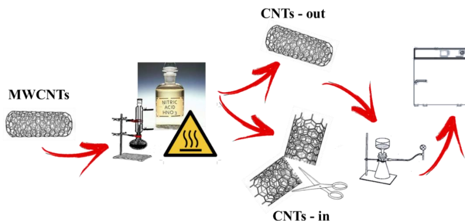
Figure 1. Scheme of pretreatment of CNTs.
