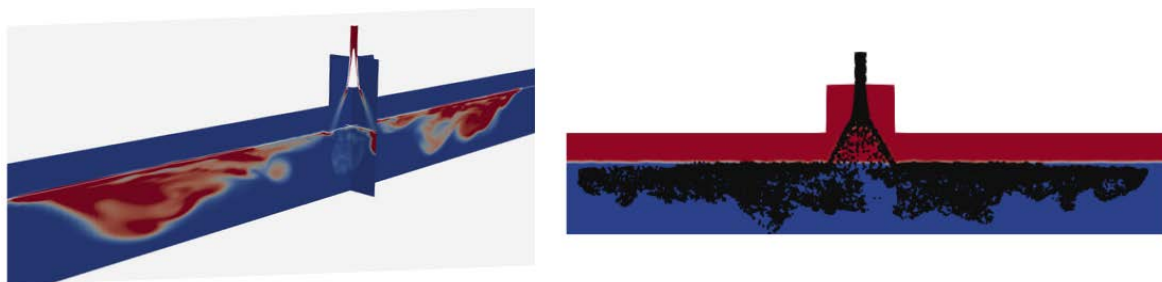
Figure 1.10: Differences in modelling between multifluid (left) and multifluid-Lagrangian tracking (right) methods for liquid-gas-solid flows. Cases presented in chapter 5.
