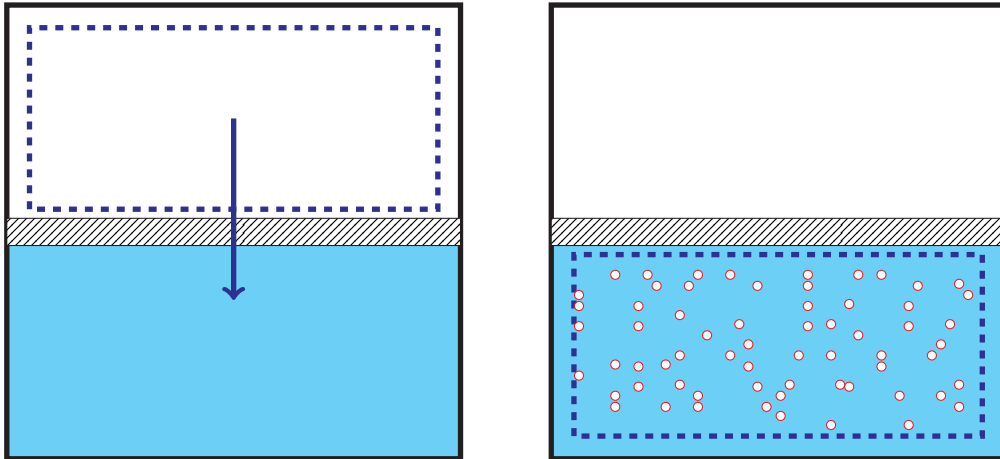
Figure 4.9: Sketch showing the idea behind the third inclusion model. A buffer region separates the continuous air from dispersed air. In that region liquid turbulent eddies breakup air structures until they reach Hinze's scale. Dispersed air exits the buffer region with that size.
