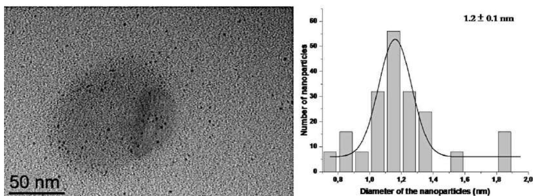
Figure 24: TEM image of \text{Ru}_1\text{Cu}_1/\text{PVP} after catalysis in 1-PrOH (scale bar 50 nm) together with the respective size histogram.
