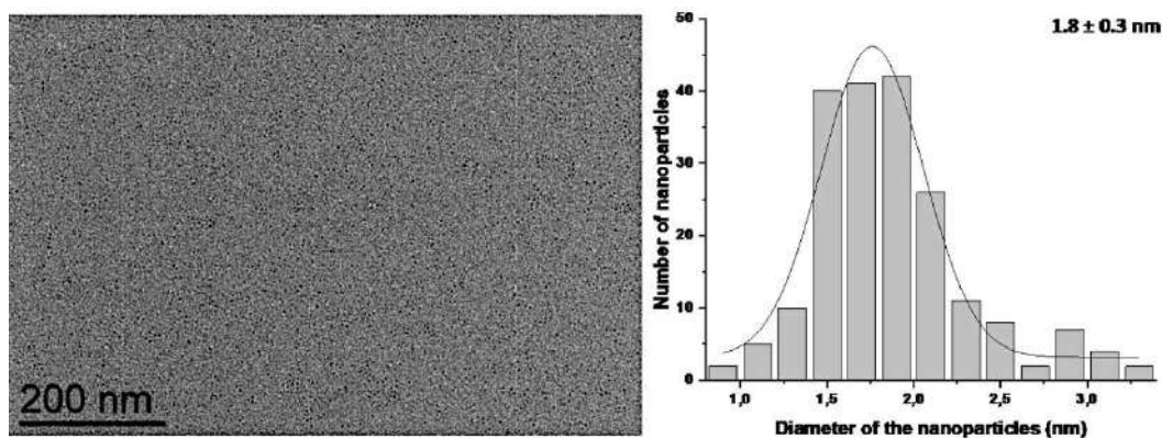
Figure 37: TEM image of RuNi/AdCOOH NPs (scale bar 200 nm) together with the respective size histogram.
