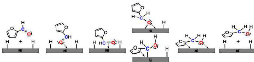
Figure 19: Simplified energy profile for the FF hydrogenation on a \text{Ni}_{38}\text{H}_{35} NP in THF.
