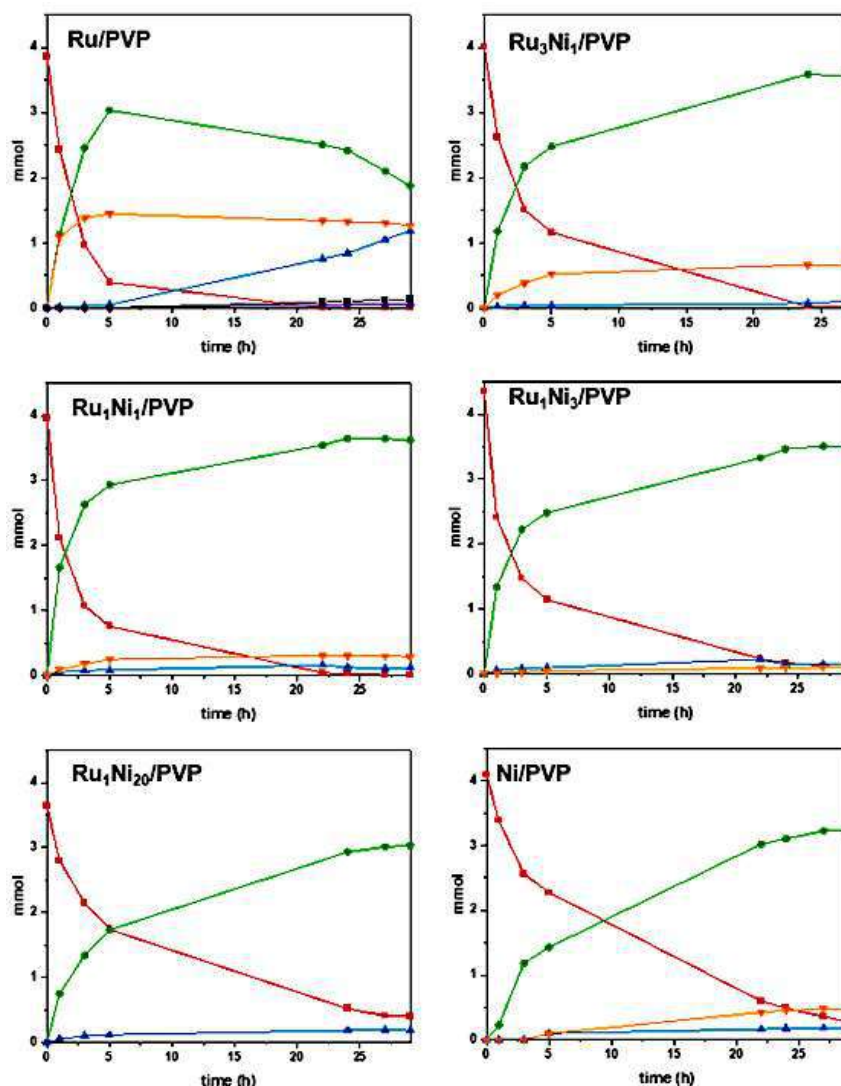
Figure 3: Time-concentration curves for the selective hydrogenation of FF in 1-PrOH on all the catalysts (red square dots, FF; green circle dots, HF; blue triangle dots, HMTHF; orange inversed triangle dots, acetal).
