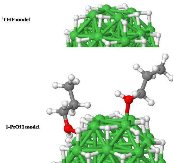
Figure 16: Ni 38 H 35 models used to investigate the hydrogenation reactions in THF (top) and in 1-PrOH (bottom). The lower part of the models is not shown for the sake of clarity.
