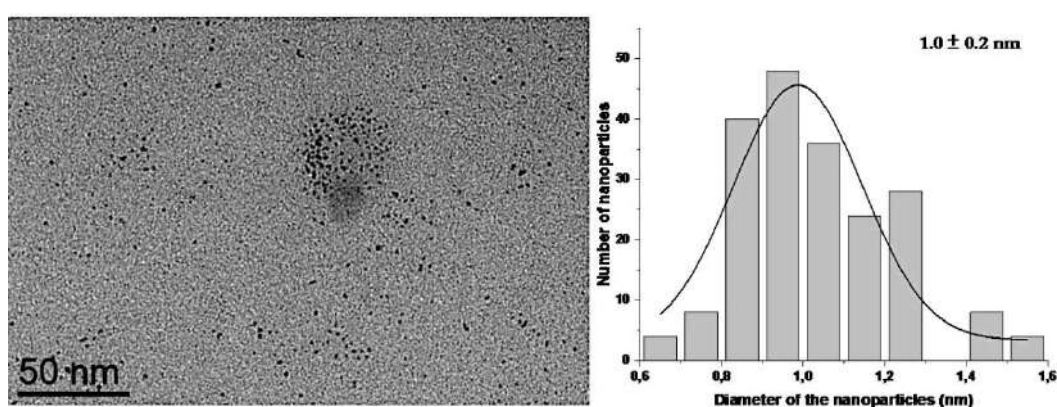
Figure 25: TEM image of \text{Ru}_1\text{Cu}_2/\text{PVP} after catalysis in 1-PrOH (scale bar 50 nm) together with the respective size histogram.
