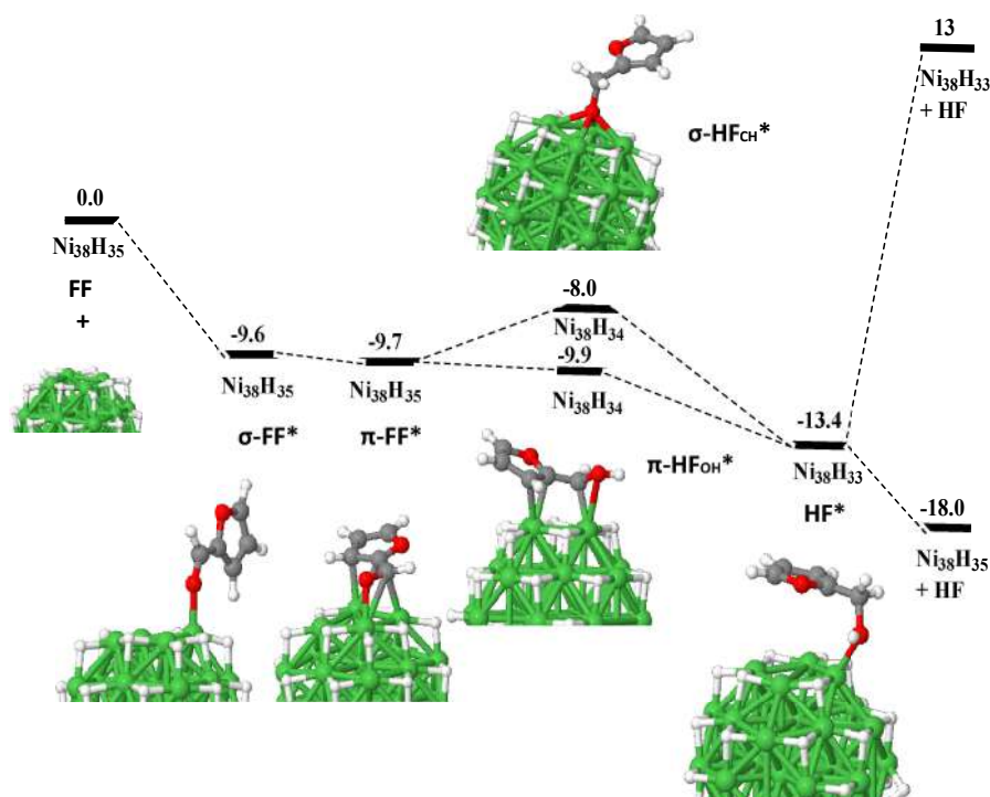
Figure 18: Energy profile for the FF hydrogenation on a \text{Ni}_{38}\text{H}_{35} NP in THF. Energies are given in \text{kcal}\cdot\text{mol}^{-1} .
