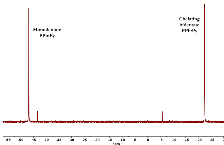
Figure 19: ^{31}\text{P}\{^1\text{H}\} NMR in THF- d 8 of [\text{Ru}(\eta^4\text{-C}_8\text{H}_{12})(\kappa^2\text{-PPh}_2\text{Py})(\text{PPh}_2\text{Py})] .
