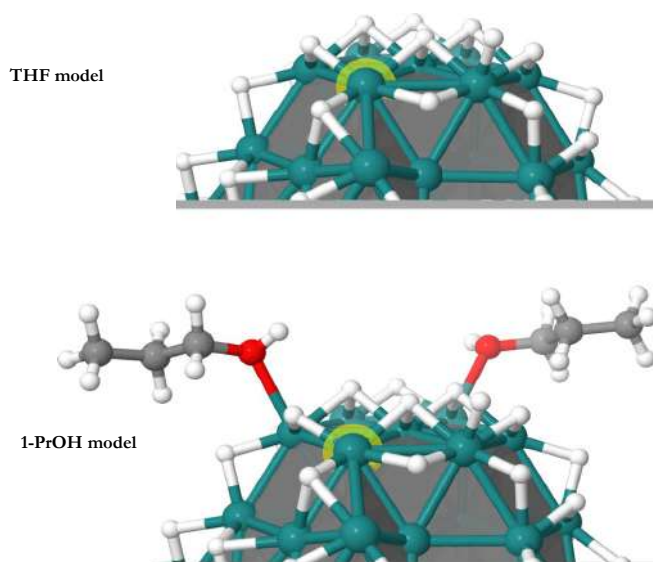
Figure 3: \text{Ru}_{55}\text{H}_{70} models used to investigate the hydrogenation reactions in THF (top) and in 1-PrOH (bottom). The considered active site is highlighted with a yellow halo. The lower part of the models is not shown for the sake of clarity.
