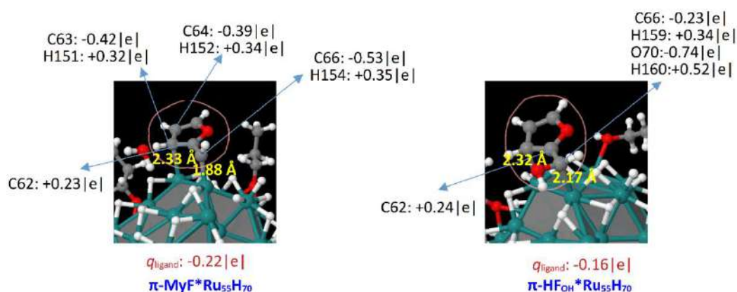
Figure 14: Comparison between \pi\text{-MyF*Ru}_{55}\text{H}_{70} and \pi\text{-HF}_{\text{OH}}\text{*Ru}_{55}\text{H}_{70} of selected geometry parameters and charges. \pi\text{-MyF*Ru}_{55}\text{H}_{70} is a dimetallacycle intermediate found on the acetal formation pathway. A vibrational analysis confirmed that it is a minimum on the potential energy surface. See also Figure 11, main text. The short Ru-C methylene (sp 2 ) bond length in this intermediate and the negative charge on the methyne fragment both suggest a kind of Ru=C double bond.
