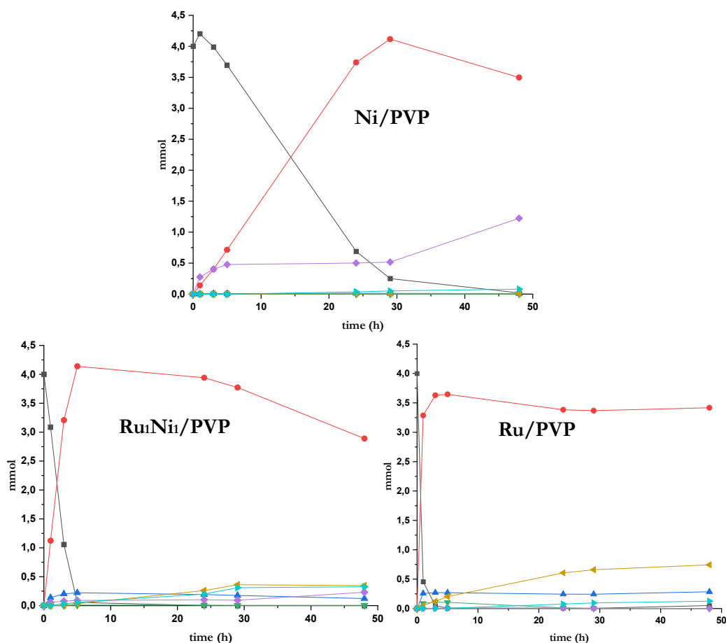
Figure 29: Time-concentration curves for the selective hydrogenation of QN in 1-PrOH at 150 °C (black square dots, QN; red circle dots, 1-THQ; blue triangle dots, 5-THQ; green inversed triangle dots, DHQ; violet twisted square dots, N.D.; brown twisted triangle dots, DHPQ; light blue twisted triangle dots, 1-THPQ).
