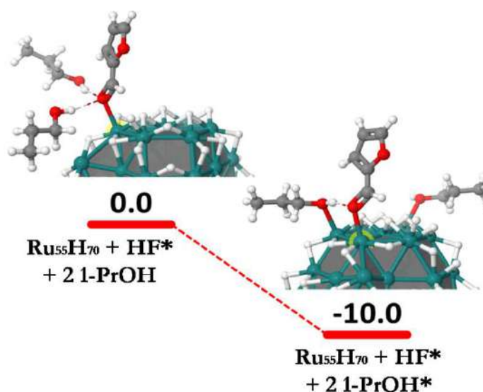
Figure 9: Possible adsorption modes of two 1-PrOH molecules on a \text{Ru}_{55}\text{H}_{70} NP. Energies are given in \text{kcal}\cdot\text{mol}^{-1} .
