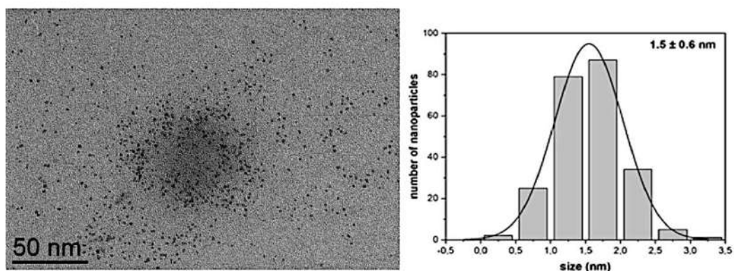
Figure 16: TEM image of Ru 1 Ni 3 /PVP after catalysis in 1-PrOH (scale bar 50 nm) together with the respective size histogram.
