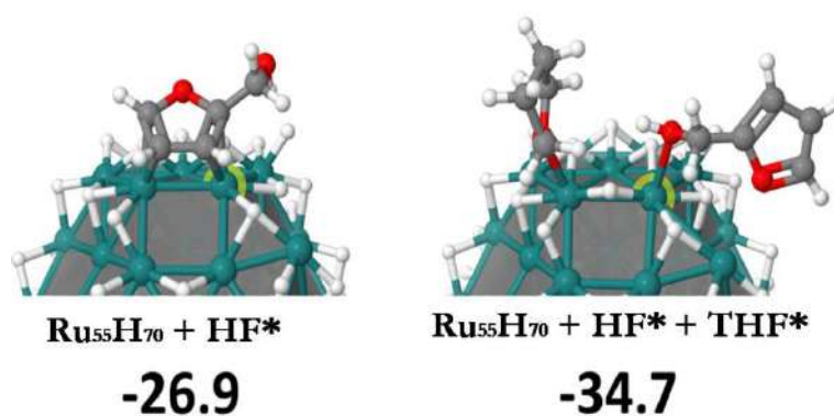
Figure 8: Possible species involved in the HF furanyl cycle hydrogenation, following the reaction of Scheme 13. Energies are given in \text{kcal}\cdot\text{mol}^{-1} .
