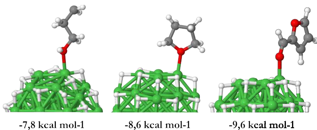
Figure 17: Adsorption energies on a \text{Ni}_{138}\text{H}_{35} NP in \text{kcal mol}^{-1} of 1-PrOH, THF and FF (from left to right).
