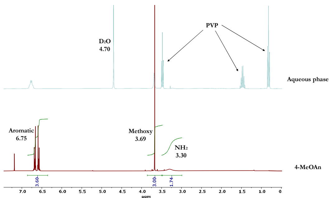
Figure 2: 1 H NMR spectra of the substrate 4-MeOAn in CDCl 3 (bottom) and of the D 2 O reaction mixture (top), after the reaction of 0.25 mmol of 4-MeOAn at 80 °C on Ru/PVP NPs in 1.5 mL of D 2 O.
