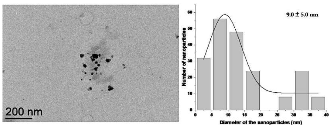
Figure 26: TEM image of \text{Cu}/\text{PVP} after catalysis in 1-PrOH (scale bar 200 nm) together with the respective size histogram.
