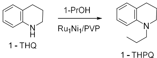
Scheme 3: Simplified reaction scheme of the condensation reaction between 1-THQ and 1-PrOH on \text{Ru}_1\text{Ni}_1/\text{PVP} catalyst, forming 1-THPQ.
