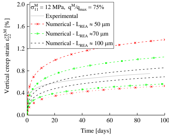
Figure 6-16 Variability of clay rock mechanical creep response due to different characteristic sizes of the mesostructure during biaxial creep test under a constant deviatoric stress level of q^M/q_{max} = 75\% .
