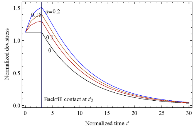
Figure 3-11 Profiles of normalized deviatoric stress at r' = 1.1 with different values of dilation parameter \alpha .
