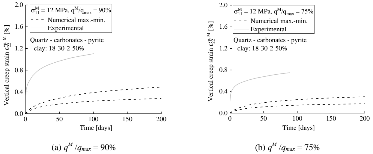
Figure 6-20 Variability of clay rock mechanical creep response at mesoscale during biaxial creep tests considering viscoelastic clay aggregate contacts under two deviatoric stress levels of q^M/q_{max} = (a) 90% and (b) 75%.
