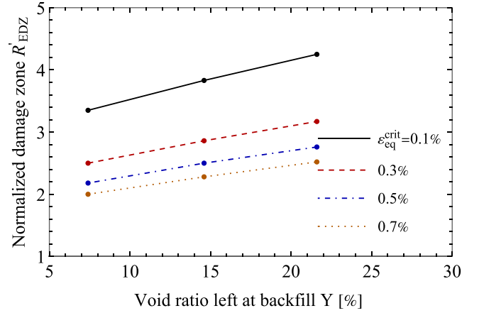
Figure 3-28 Profile of R'_{EDZ} versus Y with different threshold values of strain criterion.
