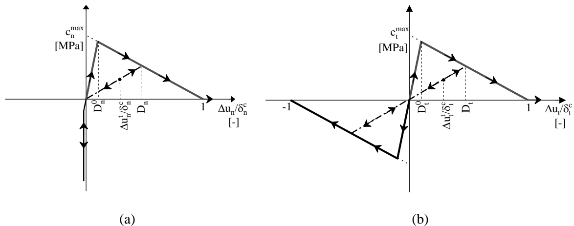
Figure 7-1 Damageable cohesive interface model in (a) normal direction; and (b) tangential direction.
