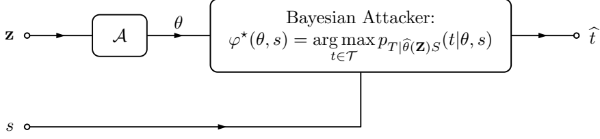
Figure 2.1: Schematic of the Bayesian attacker. The Bayesian attacker achieves the upper bound shown in Theorem 1, but needs to be able to evaluate the conditional distribution p_{T|\widehat{\theta}(\mathbf{Z})_S} . The observations required for the attack are the side-information s and model parameters \theta .
