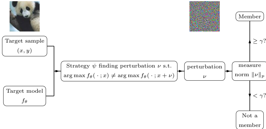
Figure 2.3: Schematic of the Adversarial Distance method for membership inference. A target sample and target model are taken as input. A perturbation is computed using an adversarial attack strategy, such that the model changes its original prediction. The magnitude of the perturbation is computed and compared to a threshold. Based on this comparison, the attacker predicts if the sample belongs to the training set of the target model or not.
