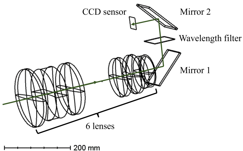
Figure 1.10: 3-dimensional representation generated with Zemax of the image acquisition system with 6 lens, two mirrors, one wavelength filter and a CCD sensor.
