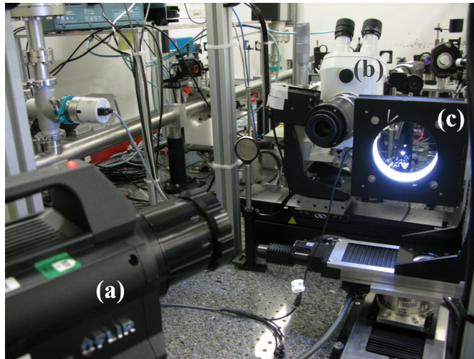
Figure A.1: Laser damage set-up MELBA with (a) a FLIR X6570sc thermal camera, (b) the visible light image acquisition system and (c) the fused silica sample in its support with the lighting system on.
