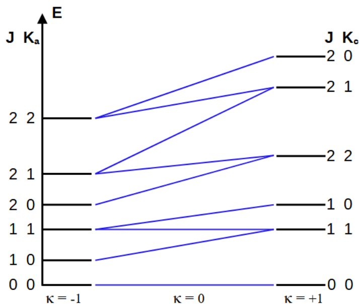
Figure 2.1: Representation of the rotational energy levels of an asymmetric-top molecule with respect to Ray's asymmetry parameter: the left side displays the J K_a values, while the right side shows the J K_c values, each associated with their respective vertical axes.
