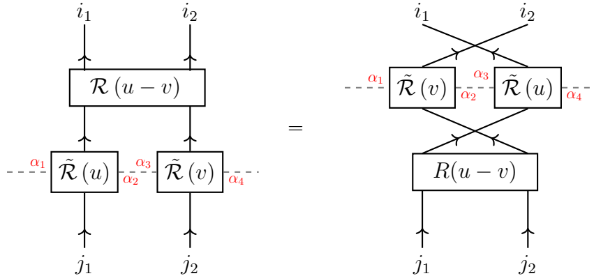
Figure B.1: This is the diagrammatical representation of (B.1.14). The gray dashed line represents the auxiliary space, and ( \alpha )'s govern the operator contraction with the auxiliary space. The black straight lines are the representation of the physical spaces, which are labeled by (i,j), and ( k )'s govern the contraction of the operators with the physical space.
