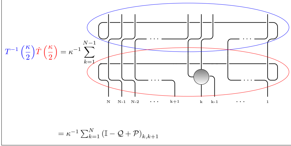
Figure III.1: This is a diagrammatic description of the non-twisted Hamiltonian of a spin chain with SO(2r) symmetry. This follows exactly like the non-twisted diagram description of the Hamiltonian of the GL(n) case up to a difference in the derivative of R'(\kappa/2) = (\kappa\mathbb{I} + \mathcal{P} - \mathcal{Q}) , which is represented as the shaded circle, and for the rest of the lines, R(\kappa/2) = \mathcal{P} .
