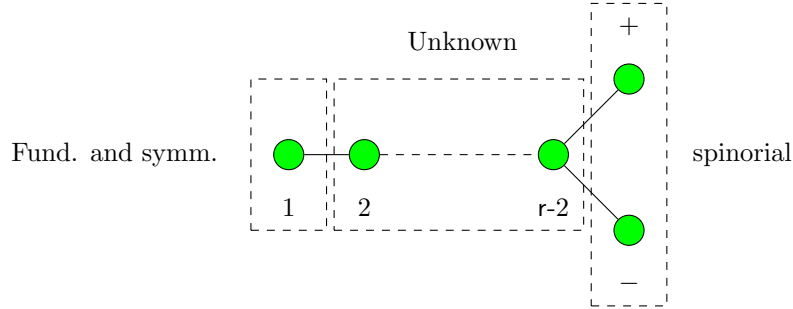
Figure III.2: SO(2r) Dynkin diagram. We are distinguishing the diagonal into three parts if we know the R -matrix of the symmetry proposed by the nodes of the diagram.
