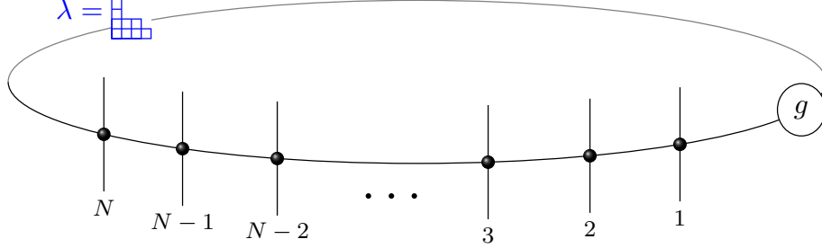
Figure II.3: A graphical description of a T -operators with a general representation \lambda in the auxiliary space. The R -matrix are represented as small black balls and multiplied along the auxiliary space. whereas the set of vertical lines physical space relabels the Hilbert space, these spaces are defined in the fundamental representation \lambda = \square .
