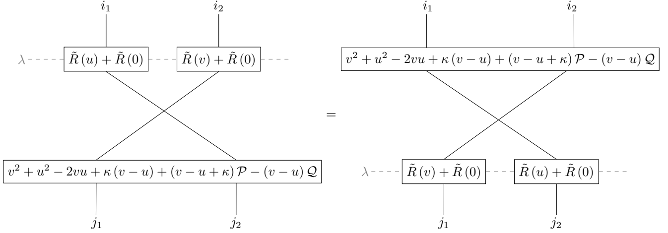
Figure III.5: A diagrammatic representation of Yang-Baxter equation with SO(2r) symmetry. It read exactly like Fig(B.3) up to the definition of the R -matrix (III.1.8).
