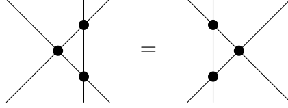
Figure II.2: The diagrammatic representation of the Yang-Baxter equation (II.1.1a)
