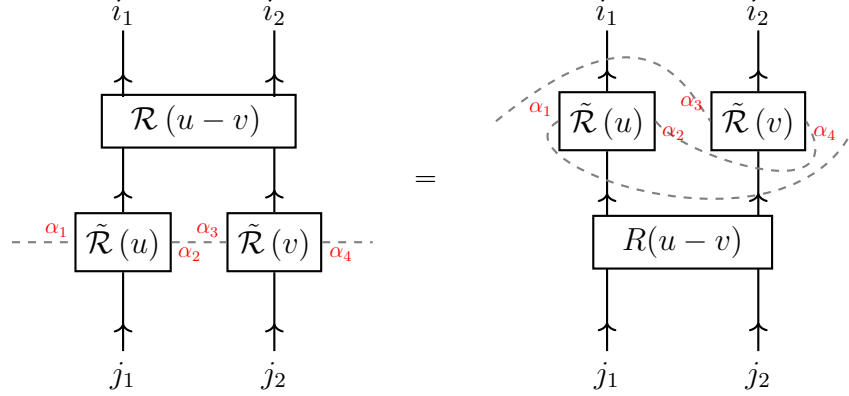
Figure B.2: This is the diagrammatical result of swapping the operators on left hand side of Fig(B.1). The difference between the auxiliary space on both sides of the diagram is due to the swapping of the two operators in the physical space and keeping the same contraction with the auxiliary space.
