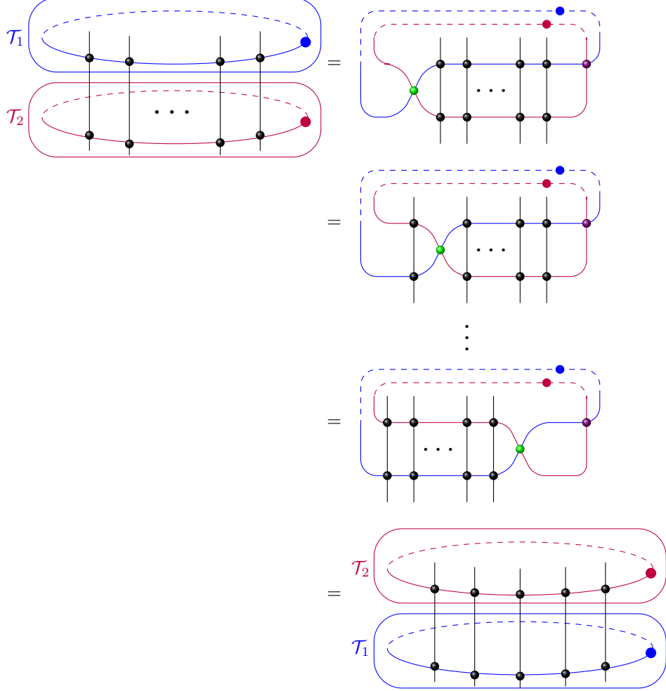
Figure II.1: This is a rough graphical description of the commutation relation between the so-called T -operators. The first part of this diagram represents two operators, \mathcal{T}_1 and \mathcal{T}_2 represented as two ellipses with vertical lines crossing each ellipse. Then, using the famous Yang-Baxter equation, one can show the commutativity between T -operators.
