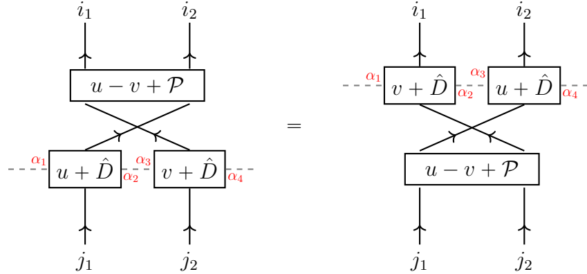
Figure B.3: A diagrammatical representation of (B.1.14) after replacing the operators with their \hat{D} . Notice that we are ommiting the identity operator \mathbb{I}
