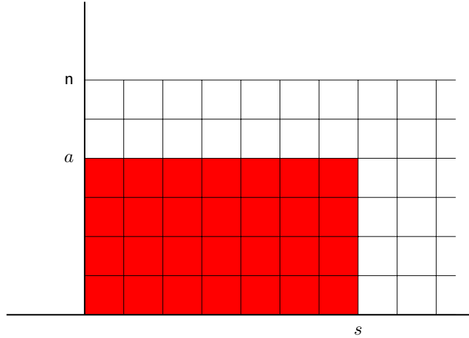
A rectangular Young diagram (\lambda = (7, 7, 7, 7, 0, 0, \dots)) .
