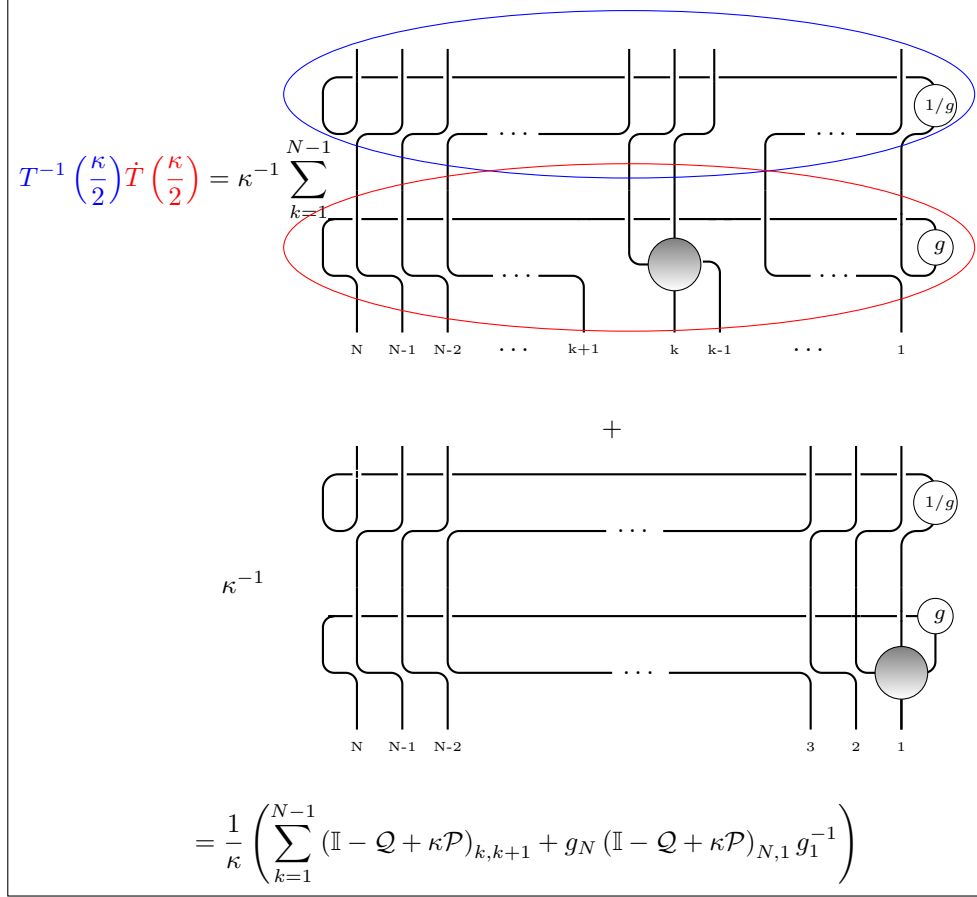
Figure III.3: This is a diagrammatic description of the twisted Hamiltonian of SO(2r) spin chains. The first part of the diagram follows as Fig(III.1), which means the lines connecting the twists cancel out. For the second part of the diagram, we have the twist connected to R'(u) \Big|_{u=\frac{\kappa}{2}} = (\kappa \mathbb{I} + \mathcal{P} - \mathcal{Q}) which gives rise to the twist term in the expression.
